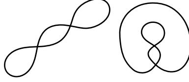
FIGURE 5. Two curves with Arnold invariants J^+ = 0 , J^- = -2 , St = 0 and winding number W = 1
