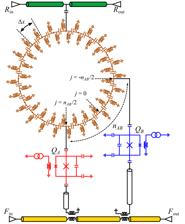
FIG. 6. The full physical-circuit schematic. Right-handed transmission lines labeled R_{\text{in}}/R_{\text{out}} and F_{\text{in}}/F_{\text{out}} , in green and yellow, respectively, are used for microwave readout. The 24-cell ring-resonator circuit is shown in orange. The capacitively coupled qubits, Q_A and Q_B , are shown in red and blue, respectively, and are separated by a distance of n_{AB} = 6 . The qubit readout cavities are comprised of quarter-wave coplanar waveguide resonators.
