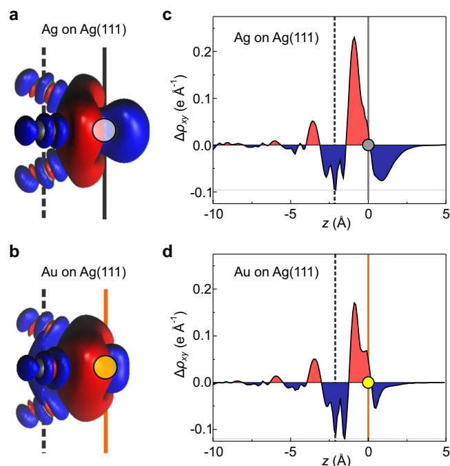
Fig. 5 | Charge density differences of Ag and Au adatoms. a, b Isosurface plots of \Delta\rho(\mathbf{r}) = \pm 0.007 \text{ e } \text{\AA}^{-3} for a single Ag or Au adatom, respectively. Charge accumulation is shown in red, depletion in blue. Indicated are the z height of the Ag surface atoms (grey, dashed) and of the adatom at z=0 (solid). c, d Plots of the xy -integrated charge density difference \Delta\rho_{xy}(z) for a single Ag or Au adatom (indicated as grey or yellow circle respectively).
