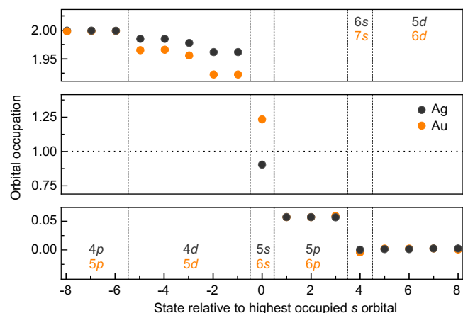
Fig. 6 | Orbital occupation. Occupation of several orbitals of single Ag and Au adatoms on Ag(111). Vertical dashed lines separate subshells. The horizontal dotted line indicates half occupation. Note that y -axis scaling varies between panels.
