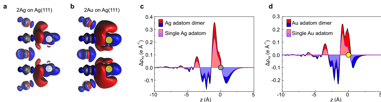
Fig. 8 | Charge density difference for dimer adsorption. a, b Isosurface plots of \Delta\rho(r) = \pm 0.02 e \text{ \AA}^{-3} for the adsorption of a Ag or Au adatom dimer (as a whole) onto Ag(111). Adatom positions are indicated by filled grey and yellow circles. Charge
