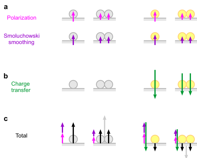
Fig. 9 | Schematic summary of dipole contributions. a The per-atom dipole contributions from polarization (pink) and Smoluchowski smoothing (purple) are positive for Ag (grey) and Au (yellow) and decrease upon dimer formation. b The charge transfer (green) which is only present for Au adatoms is negative and likewise decreases when a dimer forms. c As a result, the total (absolute) per-atom dipole (black) of Ag adatoms decreases upon dimerization, while it remains constant for Au adatoms. Grey arrows represent the dipole moments of the dimers. Note that all arrow lengths only visualize trends without being quantitative.
