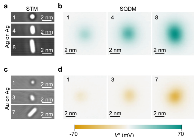
Fig. 2 | STM topography and electrostatic potential images. a Selected constant-current STM images of 1, 4, and 8 Ag adatom chains on Ag(111). b V^* images of the chains in (a). c Constant-current STM images of 1, 3, 7 Au adatoms on Ag(111). d V^* images of the chains in (c). The colour scale applies to all V^* images shown.
