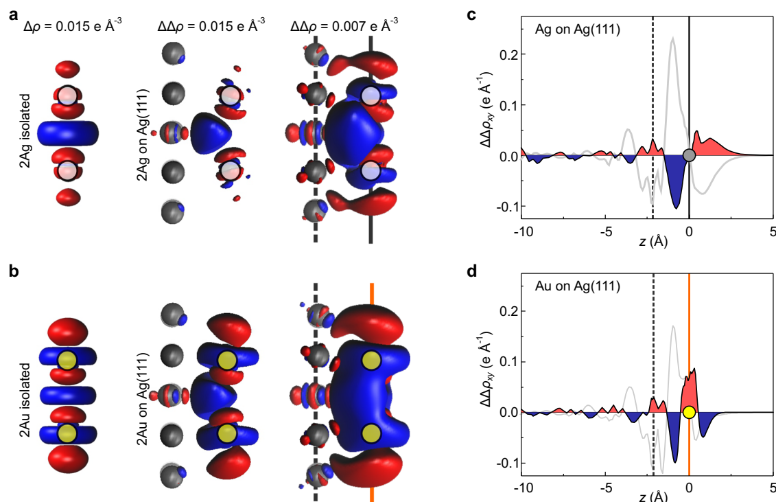
Fig. 7 | Charge density difference for dimer formation. a, b Isosurface plots for isolated Ag and Au dimers ( \Delta\rho(r) = \pm 0.015 \text{ e } \text{\AA}^{-3} , left) and for Ag and Au adatom dimer on the Ag(111) surface ( \Delta\rho(r) = \pm 0.015 \text{ e } \text{\AA}^{-3} and \pm 0.007 \text{ e } \text{\AA}^{-3} , centre, right). Charge accumulation is shown in red, depletion in blue. Vertical lines indicate the z height of the Ag surface atoms (grey, dashed) and of the adatom (solid grey (Ag)
