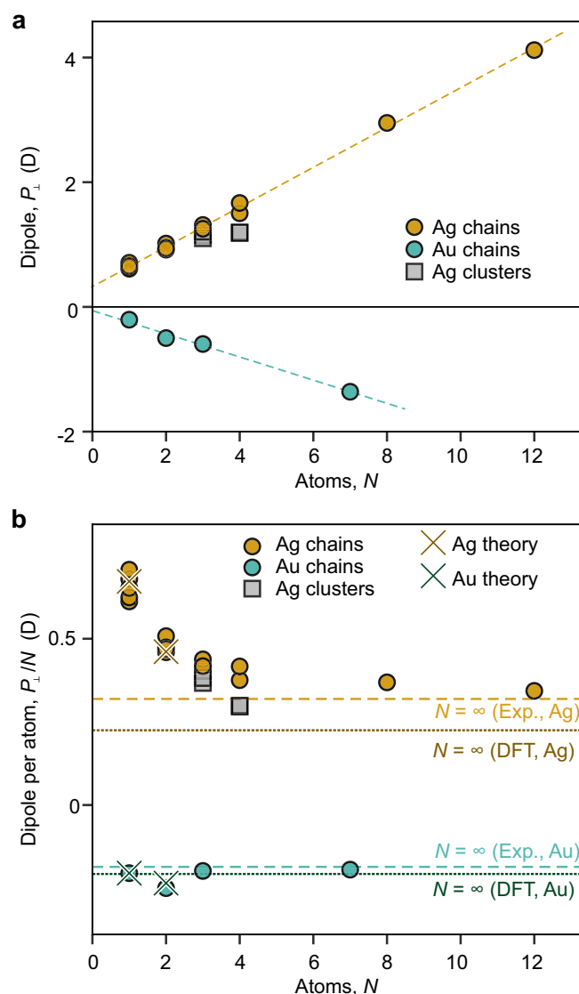
Fig. 3 | Surface dipole moments. a Measured total dipole moments P_{\perp} of Ag adatom chains and clusters (dark yellow circles and grey squares), and Au adatom chains (teal circles). The uncertainty interval of our P_{\perp} values can be assessed since we have fabricated and measured several Ag structures with 1 \leq N \leq 4 , the P_{\perp} values of which largely overlap in the plot. b Dipole moment per atom P_{\perp}/N , for the data in (a). The crosses and dotted lines (brown and dark green) mark the values obtained from our DFT calculations for N=1, 2, \infty , the dashed dark yellow and teal lines mark the respective asymptotic limits N=\infty for the experimental data as obtained from the linear fits in (a).
