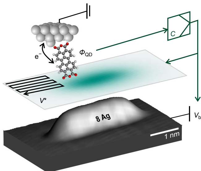
Fig. 1 | Measurement principle of SQDM. A single molecule, in this case PTCDA, is attached to the probe tip. It acts as a quantum dot (QD) that can be gated and charged with individual electrons by applying a bias voltage V_b to the sample. To image the electrostatic potential V^* , the probe scans the sample (here, a chain of 8-Ag adatoms on Ag(111)) while changes in the surface potential beneath the tip are compensated by adjusting V_b via a controller C, maintaining a constant QD potential \Phi_{QD} .
