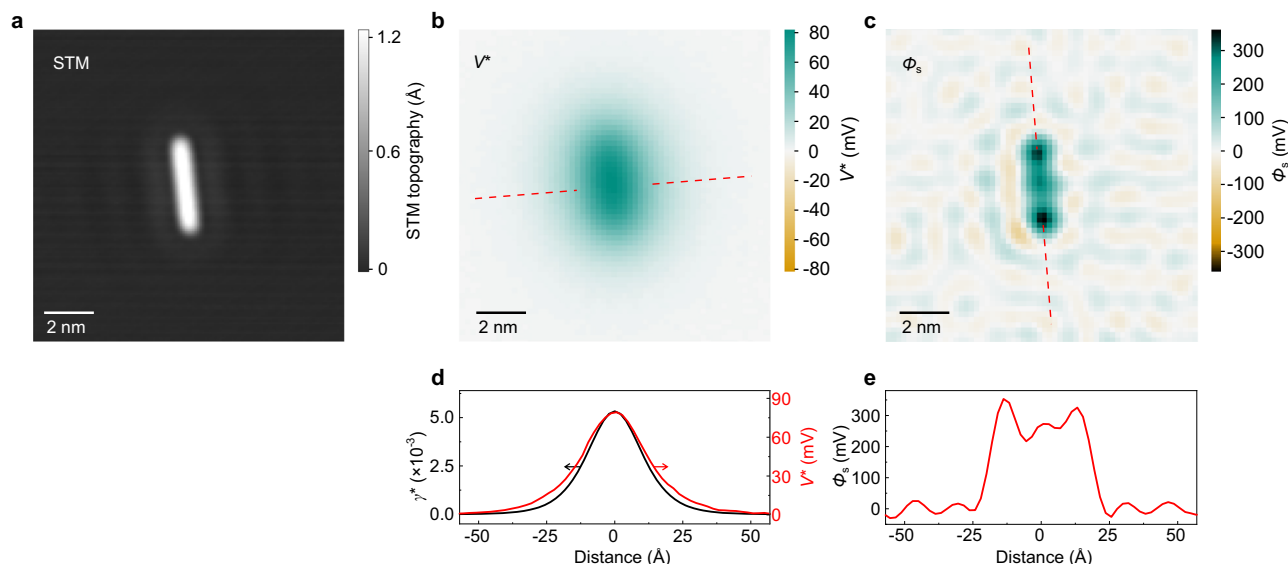
Fig. 4 | Surface potential obtained by deconvolution. a STM image of a 12-atom Ag chain. b SQDM V^* image of the chain in (a) . c Surface potential \Phi_s obtained from deconvolving the V^* image in (b) using \gamma^{*18} . d Comparison of cross sections
