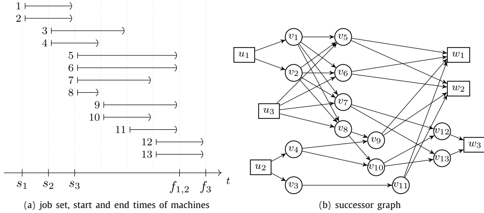
Fig. 6. Successor graph for the FLEXMISMA instance with m = 3 and C = 2 .
