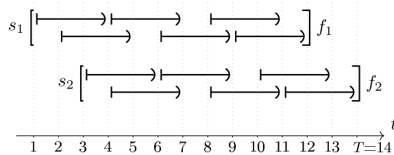
Fig. 9. An instance of 3-FLEXMISMA and its feasible solution. All pairs of equivalent jobs are split.
