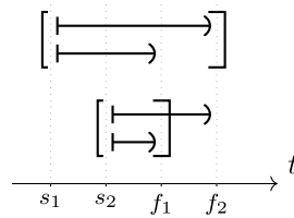
Fig. 2. An infeasible instance of FLEXMISMA that respects the available machine capacity.
