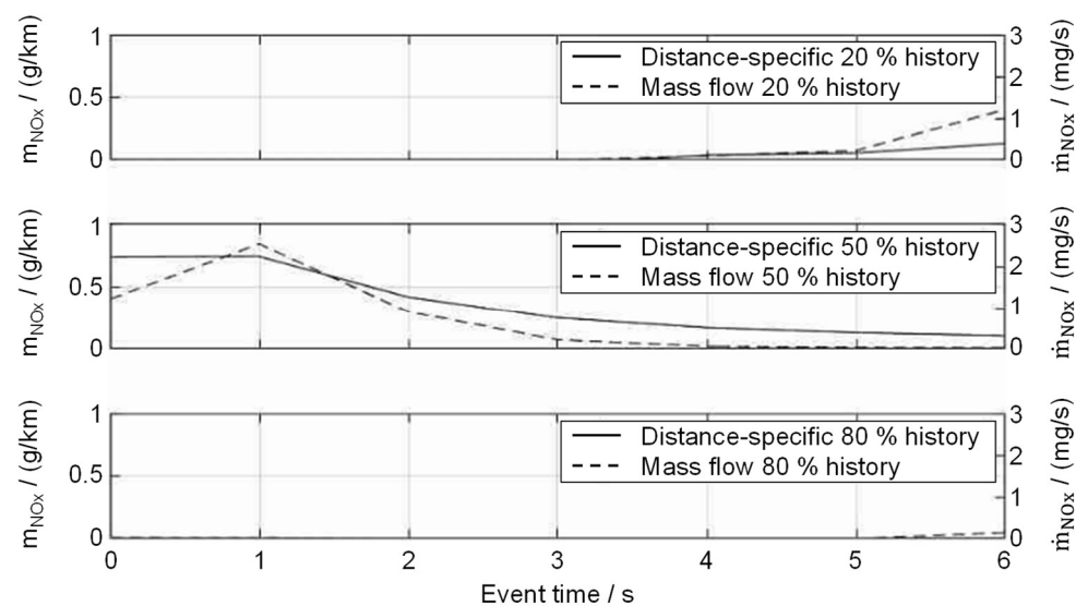
Figure 10. Event emission profile for 20% ( top ), 50% ( center ) and 80% ( bottom ) history.
