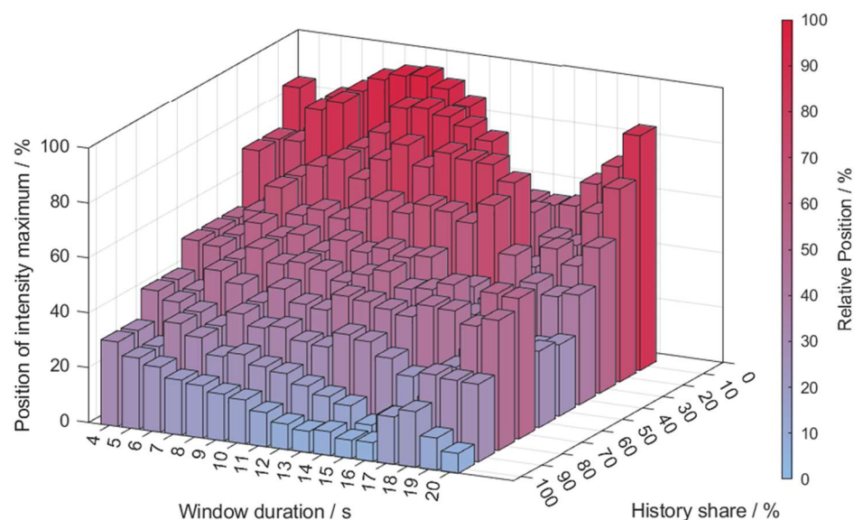
Figure 8. Relative position of emission intensity peak in NO x events.
