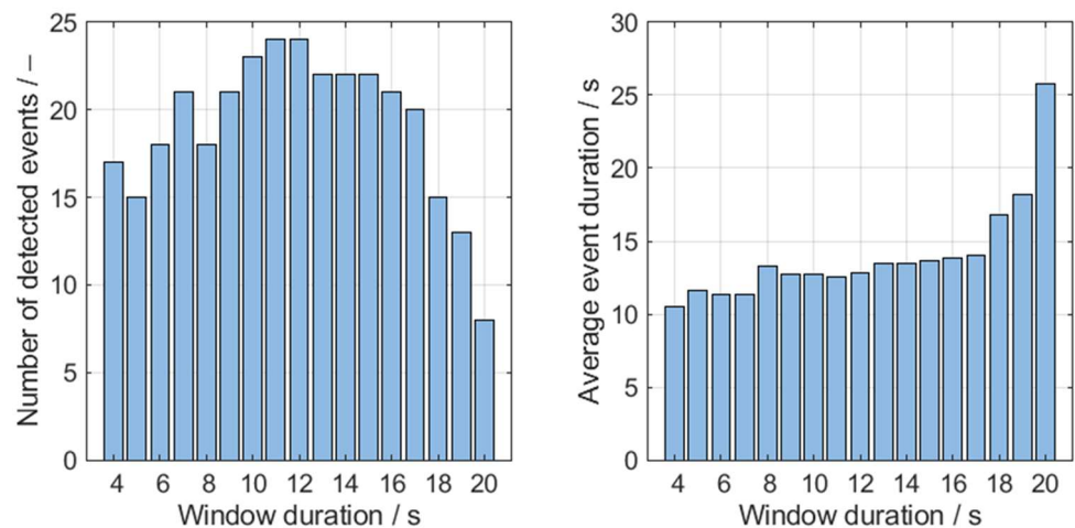
Figure 6. Influence of the window duration on the number of detected events ( left ) and average duration ( right ) for \text{NO}_x emissions and 20% history consideration.
