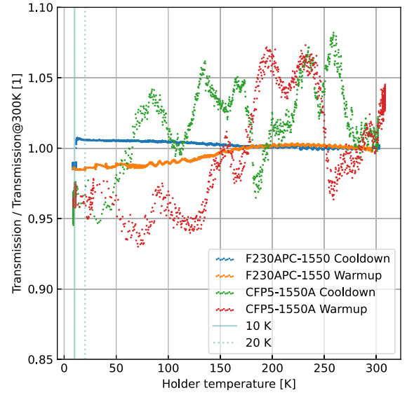
Fig. 4. Measurement of the temperature dependency of the light transmission for the optical system of collimator and fibers. Each shown measurement displays data from a thermal cycle similar to Fig. 2. The CFP5-1550 showed significantly more fluctuations during the cooling cycle compared to the F230APC. Compared to during the temperature ramping, the F230APC had a significantly more stable light throughput at a constant temperature.
