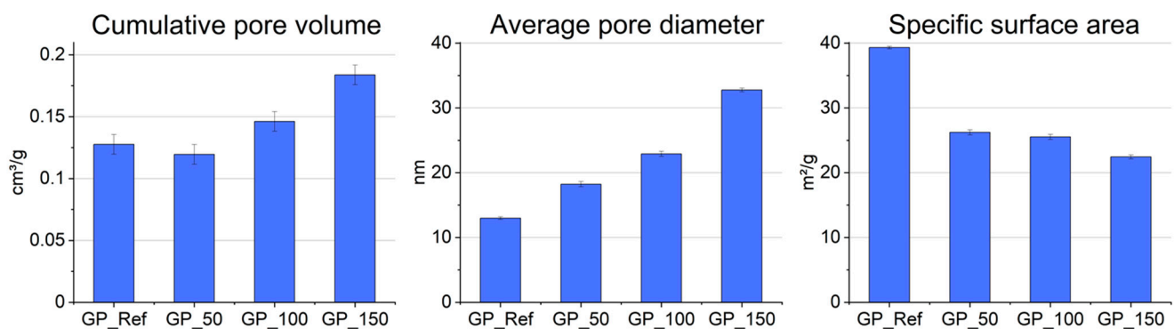
Figure 4. Results of the mercury intrusion porosimetry. Pore volumes are presented in cm 3 /g of geopolymer with an error of \pm 0.008 cm 3 , according to [32].
