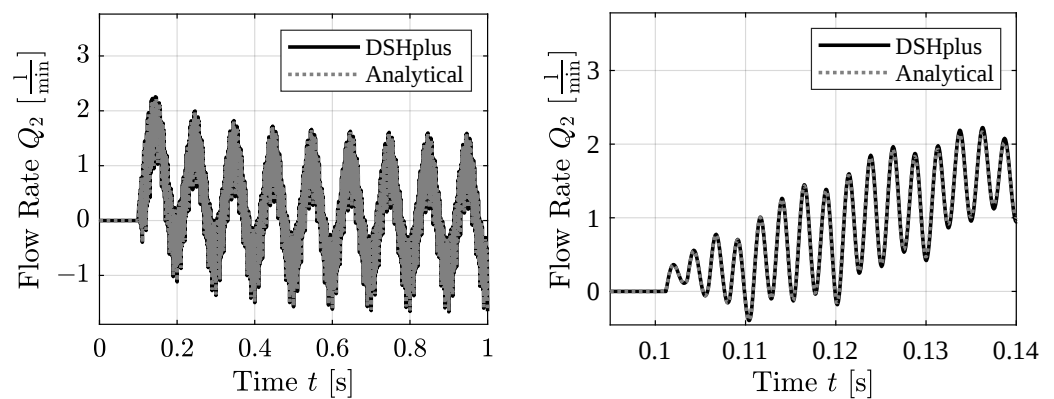
Figure 11. Sum of sine waves with 10 Hz, 100 Hz, 200 Hz, and 400 Hz pressure boundaries at 50 bar level.
