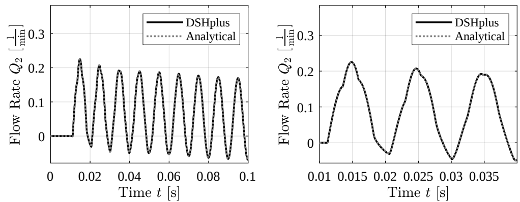
Figure 8. The 100 Hz sine wave pressure boundary at the 50 bar level.
