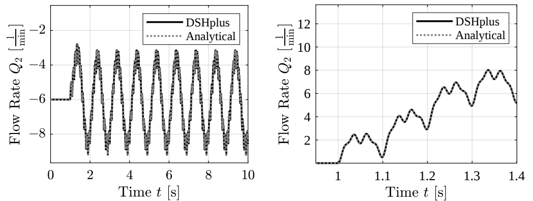
Figure 10. Sum of sine waves with 1 Hz, 10 Hz, 20 Hz, and 40 Hz pressure boundaries at 50 bar level.
