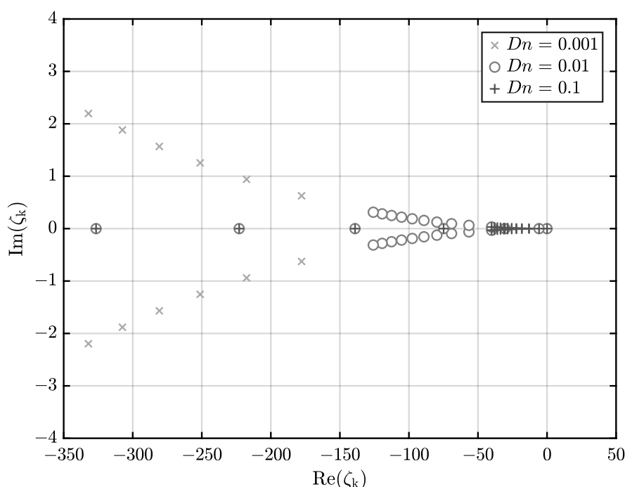
Figure 6. Position of the poles of W_1^*(\zeta) for various Dn .
