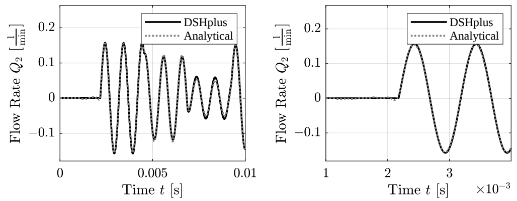
Figure 9. The 1000 Hz sine wave pressure boundary at the 50 bar level.
