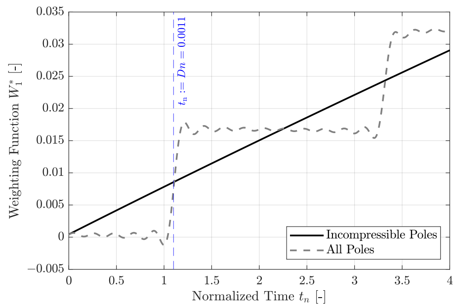
Figure 4. Weighting functions featuring only residues of negative real poles (incompressible solution) and residues of all poles (compressible solution).
