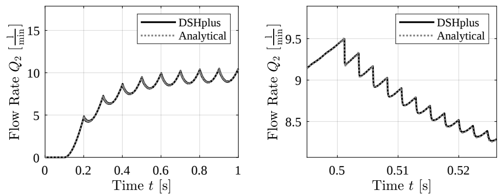
Figure 12. Sawtooth pressure boundary at 50 bar level.
