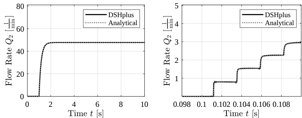
Figure 13. Step function pressure boundary at 50 bar level.
