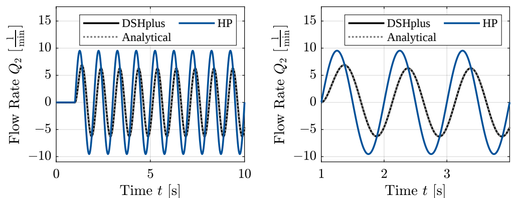
Figure 7. The 1 Hz sine wave pressure boundary at the 50 bar level.
