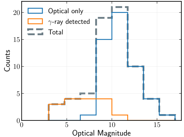
Figure 2. Peak optical magnitudes of the novae used in this analysis. Those novae that were detected in gamma rays or were identified as candidate gamma-ray emitters in Franckowiak et al. (2018) are shown in the orange histogram, whereas the blue histogram shows novae that were not detected in gamma rays. The gray histogram shows the total of all novae used in the analysis.
