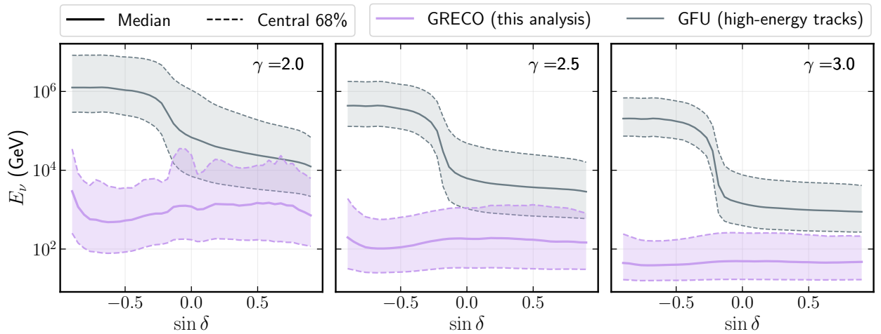
Figure 9. Central 68% of the expected true neutrino energies for sources with F_{\nu+\bar{\nu}} \propto E^{-2} (left), E^{-2.5} (middle), or E^{-3} (right) spectra. We compare this analysis (pink) to a higher-energy event selection (gray). This distribution only shows the distribution of true energies that are present in the dataset, although higher-energy and better reconstructed events tend to have a larger effect on the analysis sensitivity than lower-energy events.
