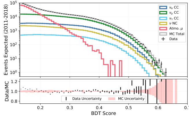
Figure 7. The expected contributions from each atmospheric background component, including neutrinos and simulations of atmospheric muons. Neutrino charged-current (CC) interactions for each neutrino flavor, neutral-current (NC) interactions for neutrinos of all flavors, and atmospheric muons are labeled in the legend, with the total of all contributions shown in gray. Error bars shown are statistical and do not include any relevant systematic uncertainties. Events with a BDT score below 0.13 are removed, yielding a sample with 60% atmospheric neutrinos and 40% atmospheric muons.
