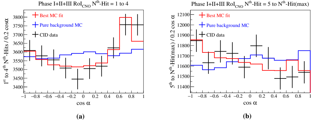
Figure 2: Illustration of the CID data (black) and the best fit results (red) summed for the Phase-I + Phase-II+III in the RoI CNO . The background-only Monte Carlo predictions (blue) scaled to the same total number of events is shown. (a) The sum of the first to fourth N^{\text{th}} -hits \cos \alpha histograms shows the Cherenkov peak. (b) The sum of the fifth to the N^{\text{th}} -hit(max) \cos \alpha histograms shows the effect the \Delta r_{\text{dir}} parameter on these later hits.
