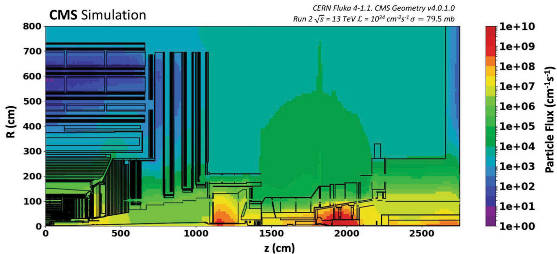
Fig. 6 Neutron flux in CMS due to \sqrt{s} = 13 TeV pp -collisions at \mathcal{L} = 10^{34} \text{ cm}^{-2} \text{ s}^{-1} simulated with FLUKA. Results are averaged over 360 degrees in \varphi , the geometry of the CMS detector is overlaid as a cut in the Z-Y plane
