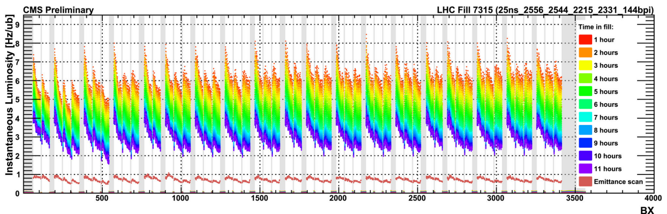
Fig. 5 Evolution of the instantaneous luminosity ( \text{Hz}/\mu\text{b} - or equivalently \times 10^{30} \text{ cm}^{-2} \text{ s}^{-1} ) per bunch along the orbit during Fill 7315. The instantaneous luminosity is averaged over different periods of about
