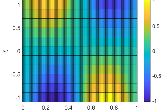
Figure 2: Numerical solution obtained by the proposed method with modified cost functional in the linear program (2.26). Initial data are u(0, x, \xi) = \xi \sin(2\pi x) . The final time is T = 1/4 .
