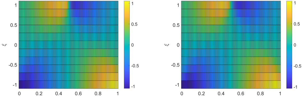
Figure 1: Numerical solutions obtained by the stochastic collocation LxF method (left) and the proposed method (right). Initial data are u(0, x, \xi) = \xi \sin(2\pi x) . The final time T = 1/4 .
