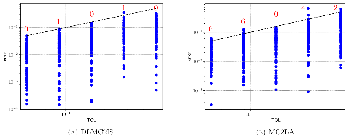
Fig. 3 Example 1: Error vs. tolerance consistency plot for various tolerances TOL with a predefined confidence parameter C_\alpha = 1.96 ( \alpha = 0.05 ). Panel A DLMC2IS estimator. Panel B MC2LA estimator
