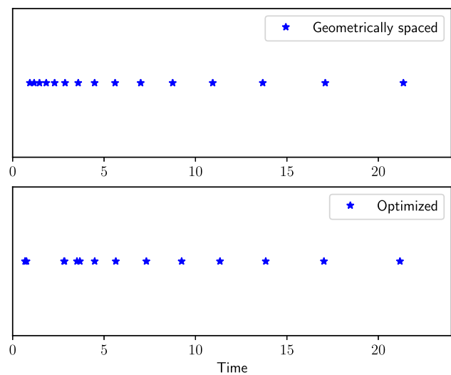
Fig. 5 Example 2: Geometrically spaced design (Goda et al. 2020) yielding expected information gain (EIG) of 6.12 vs. optimized design yielding EIG of 6.25. Clustering of measurement times appeared to have a positive impact on the EIG of the experiment. Later measurement times had little effect on the EIG and were mostly unaffected by the optimization
