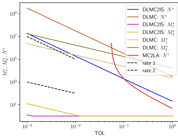
Fig. 6 Example 2: Optimal number of outer ( N^* ) and inner ( M_1^* , M_2^* ) samples vs. tolerance TOL for the DLMC, DLMC2IS, and MC2LA estimators for optimized sampling times
