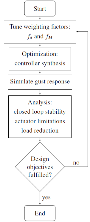
Fig. 5 Controller design workflow
