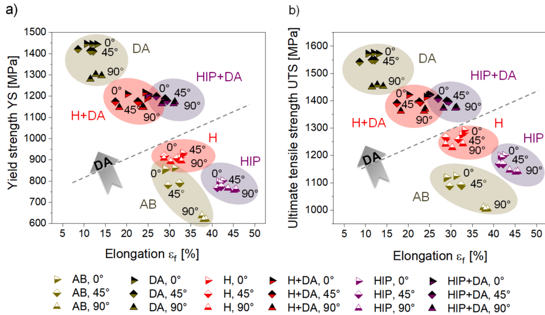
Fig. 11. The yield strength (YS, (a)) and ultimate tensile strength (UTS, (b)) as a function of elongation at fracture ( \epsilon_f ) of LPBF IN718 with optimized parameters E_v , \text{opt} = 60 \text{ J/mm}^3 for both as built and thermomechanical treated states for the different vertical build orientations of the specimens ( 0^\circ , 45^\circ and 90^\circ ).
