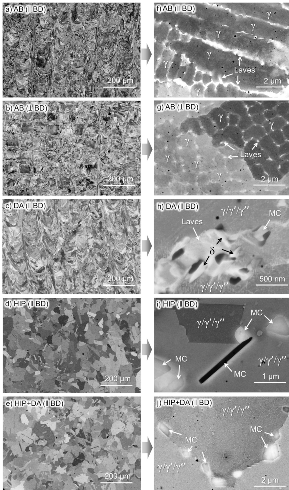
Fig. 5. Microstructures of the LPBF IN 718: as-built (|| and ⊥ to the BD in (a, f) and (b, g), respectively), DA (|| to BD, (c, h)), HIP (|| to BD, (d, i)) and HIP + DA (|| to BD, (e, j)) conditions. The figures on the right show detailed regions from the corresponding conditions on the left.
