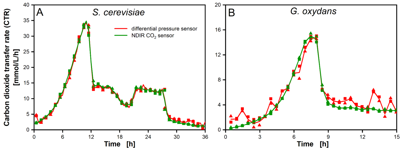
Fig. 2 Comparison of differential pressure sensor ( \Delta p sensor) and non-dispersive infrared CO 2 sensor (NDIR CO 2 sensor) for CTR measurement. CTR over time determined with \Delta p sensor (red) (as described by Anderlei et al. [17]) and NDIR CO 2 sensor (green). For comparison of both methods, a \Delta p sensor was included in the measurement setup as illustrated in Additional file 2 B. The open vent hole was replaced by a switchable outlet valve, to allow for gas tightness. Data points are presented as duplicate measurements in two individual shake flasks (square and triangle). The solid line connects the average of these two data points. A Saccharomyces cerevisiae ( S. cerevisiae ) cultivation in yeast extract peptone medium (YEP-medium) containing 20 g/L glucose. Operation conditions: shaking frequency n=200 rpm, shaking diameter d_0=50 mm, liquid filling volume V_L=25 mL, 250 mL shake flask, temperature T=30 °C, measurement time t_{\text{meas}}=6 min; B Gluconobacter oxydans ( G. oxydans ) in Jülich-medium containing 80 g/L mannitol. Operation conditions: n=350 rpm, d_0=50 mm, V_L=10 mL, 250 mL shake flask, T=30 °C, t_{\text{meas}}=6 min
