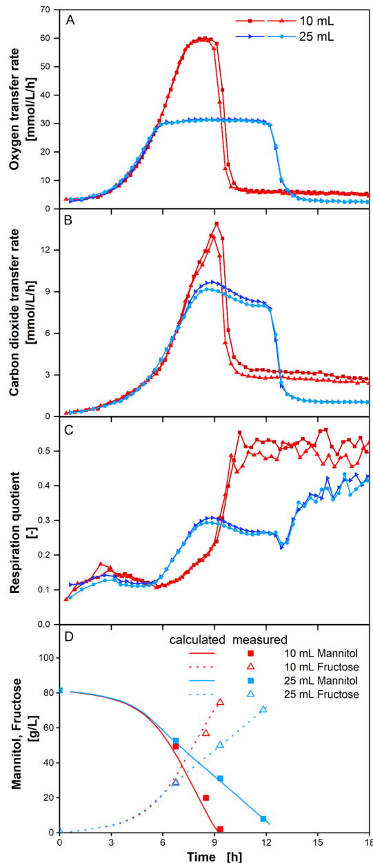
Fig. 5 Respiration activity of G. oxydans at varying oxygen limitations. OTR, CTR, RQ and sugar concentrations over time of G. oxydans 621 H \Delta hsdR in Jülich-medium containing 80 g/L mannitol as C-source at two different filling volumes (10 mL and 25 mL). Experiments were performed as duplicate measurements in two individual shake flasks. Time on x-Axis is shifted at some curves for clarity: -0.25 h for 10 mL red square, +0.25 h for 10 mL red triangle. A OTR B CTR C RQ D Measured (square and triangle symbols) and model predicted (solid and dotted lines) sugar concentrations. Model based on total oxygen consumption, total carbon dioxide production and reaction stoichiometry (see Additional file 4); mannitol (measurement: closed squares, model prediction: solid line); fructose (measurement: open triangles, model prediction: dotted line). Sugar measurements are single point measurements. Calculated values are based on average total oxygen consumption and average total carbon dioxide production from two individual shake flasks (see Additional file 3). Operation conditions: n=350 rpm, d_0=50 mm, V_L=10 and 25 mL, 250 mL shake flask, T=30^\circ\text{C} , t_{\text{meas}}=12 min reduced to t_{\text{meas}}=6 min after 3 h
