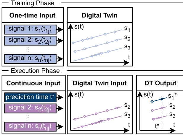
Fig. 1. Proposed DT concept.
