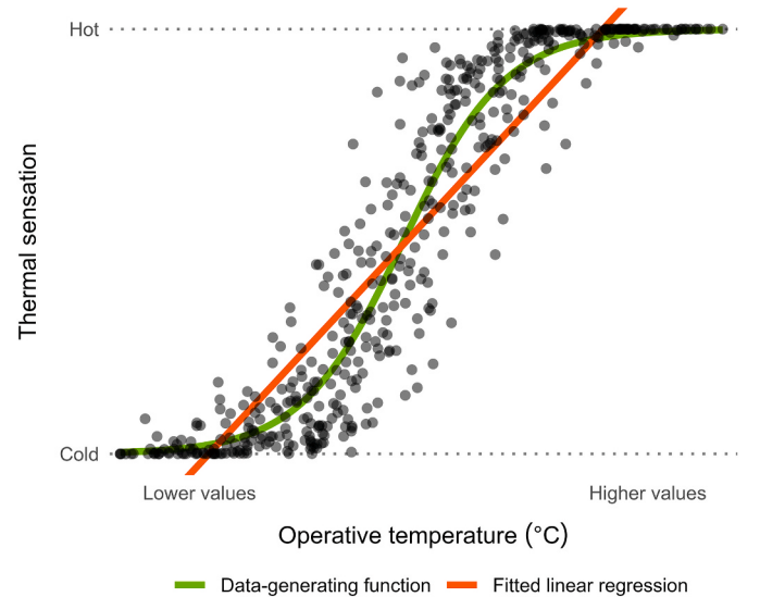
Fig. 4. – Schematic view of ceiling and floor effects. The green and orange lines represent the data-generating function and a fitted linear regression, respectively. (For interpretation of the references to colour in this figure legend, the reader is referred to the Web version of this article.)
