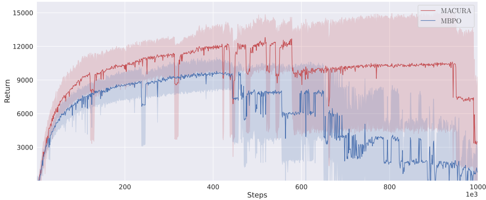
Figure 19: MACURA and MBPO with prolonged experiment length on Halfcheetah.
