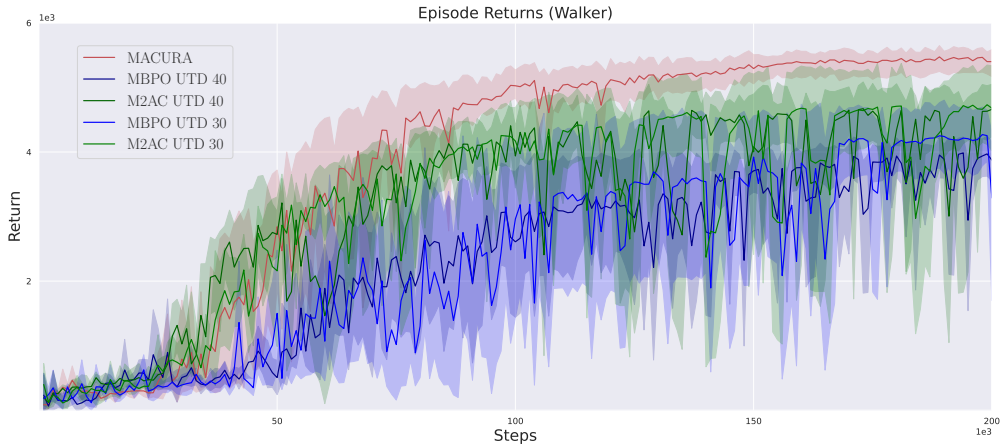
Figure 17: Comparison of returns obtained on Walker.
