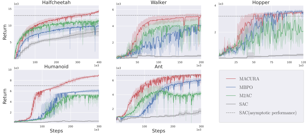
Figure 3: Performance on the MuJoCo Benchmark. MACURA shows substantial improvements in data efficiency and asymptotic performance over state-of-the-art Dyna-style MBRL approaches (MBPO, M2AC) in most tasks. Most noticeably, MACURA is on par with or outperforms the asymptotic performance of the model-free SAC baseline.
