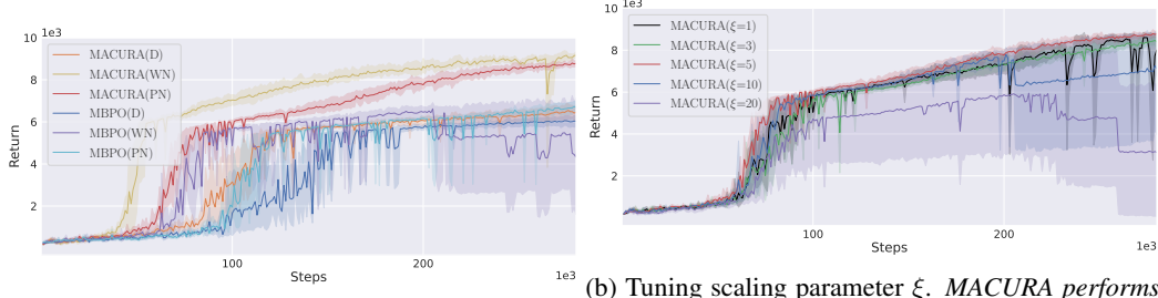
(a) Exploration Schemes on MACURA and MBPO. (b) Tuning scaling parameter \xi . MACURA performs well for intermediate \xi . Too large values of \xi lead to impact of deterministic (D), white noise (WN), and pink model exploitation, too small values lead to overfitting noise (PN) exploration on algorithmic performance. of the agent.
