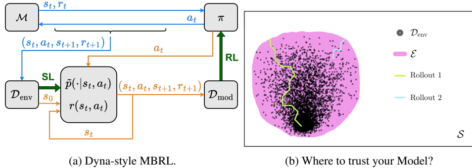
Figure 1: Algorithmic Diagrams. (a) An agent with policy \pi interacts with the environment \mathcal{M} . This data is stored in \mathcal{D}_{\text{env}} and used to train a dynamics model \tilde{p} via supervised learning (SL). Model-based rollouts under \pi are performed from start states s_0 in \mathcal{D}_{\text{env}} and stored in \mathcal{D}_{\text{mod}} . The policy is trained on \mathcal{D}_{\text{mod}} via reinforcement learning (RL). (b) \mathcal{D}_{\text{env}} induces a set of sufficient model accuracy \mathcal{E} \subseteq \mathcal{S} . A notion of \mathcal{E} allows to reason whether rollouts are in a region of sufficient model accuracy. We use this reasoning to schedule rollout length.
