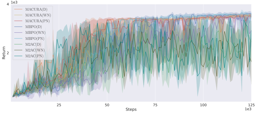
Figure 10: Exploration Schemes on MACURA, MBPO, and M2AC on Hopper. Impact of deterministic (D), white noise (WN), and pink noise (PN) exploration on algorithmic performance.
