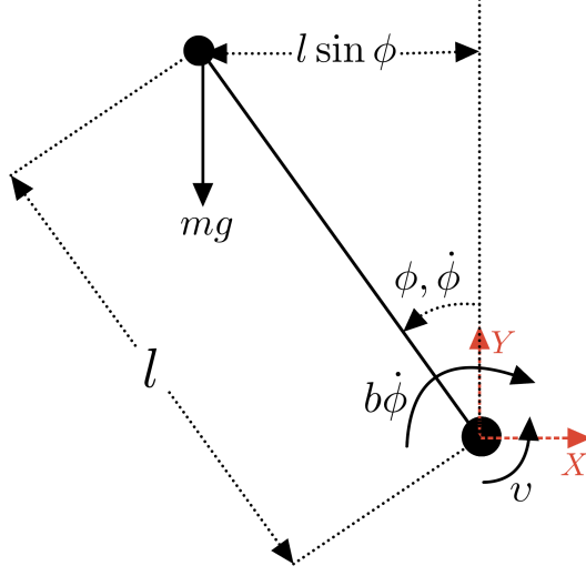
Figure 5: Free body diagram of the pendulum.
