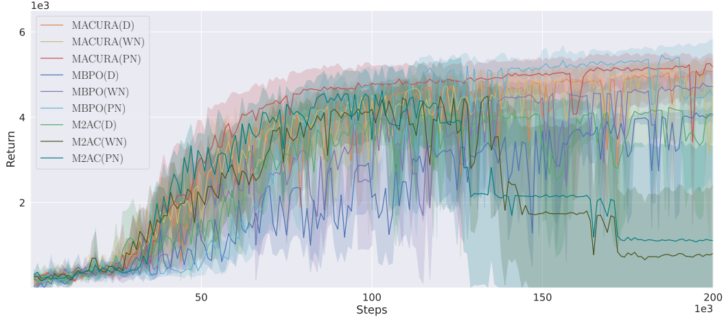
Figure 9: Exploration Schemes on MACURA, MBPO, and M2AC on Walker. Impact of deterministic (D), white noise (WN), and pink noise (PN) exploration on algorithmic performance.
