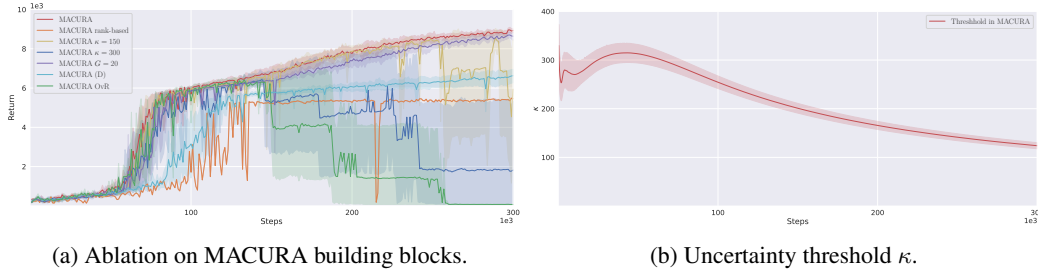
Figure 4: Ablation Study (a) The rank-based rollout mechanism with GJS uncertainty (11) and adaptive threshold (14) yields strong performance. (b) MACURA initially keeps \kappa comparatively high and reduces \kappa over time as more precise information is required to refine the policy.
