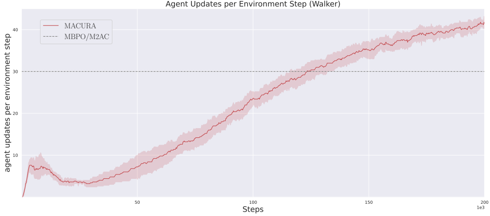
Figure 16: SAC Update Steps
