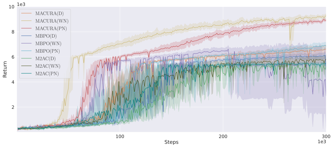
Figure 11: Exploration Schemes on MACURA, MBPO, and M2AC on Humanoid. Impact of deterministic (D), white noise (WN), and pink noise (PN) exploration on algorithmic performance.
