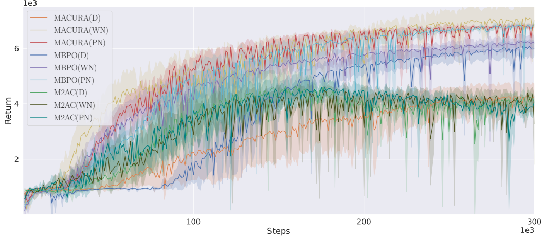
Figure 12: Exploration Schemes on MACURA, MBPO, and M2AC on Ant. Impact of deterministic (D), white noise (WN), and pink noise (PN) exploration on algorithmic performance.
