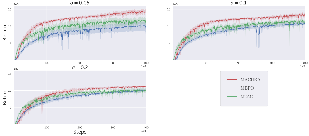
Figure 13: Returns obtained by MACURA, MBPO, and M2AC on noisy Halfcheetah.
