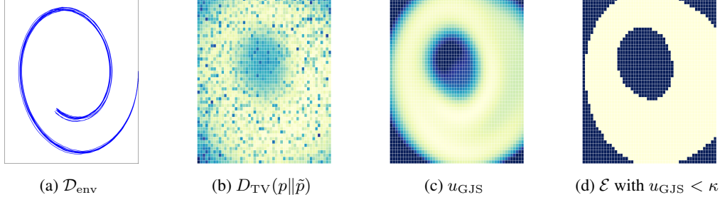
Figure 2: Constructing \mathcal{E} on a toy example. (a) Data to train the PE model. (b) Dynamics misalignment. (c) Proposed measure for model uncertainty (11). (d) Set of sufficient model accuracy to perform branched model-based rollouts (13).
