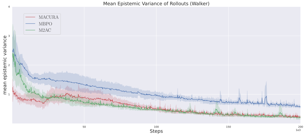
Figure 15: Mean epistemic uncertainty of rollouts for MACURA, MBPO, and M2AC on Walker.
