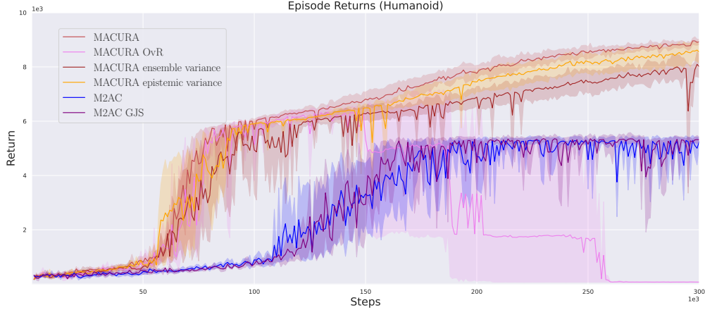
Figure 18: MACURA and M2AC with different uncertainty metrics on Humanoid.
