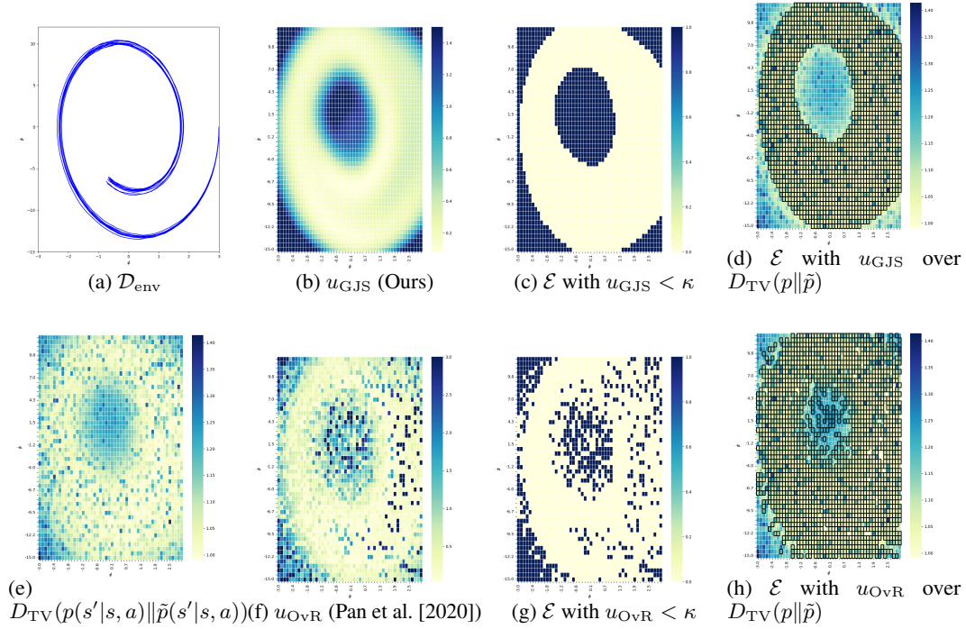
Figure 6: Effectiveness of the GJS uncertainty measure
