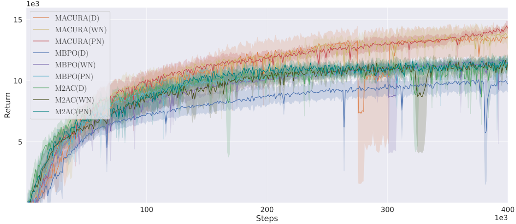
Figure 8: Exploration Schemes on MACURA, MBPO, and M2AC on Halfcheetah. Impact of deterministic (D), white noise (WN), and pink noise (PN) exploration on algorithmic performance.
