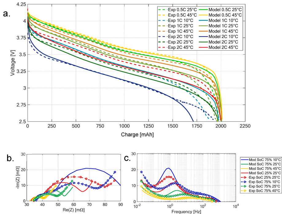
Fig. 8. Simulations of the validation dataset: a) set of discharge and EIS at various operating conditions in b) Nyquist and c) Bode of the imaginary component representations.
