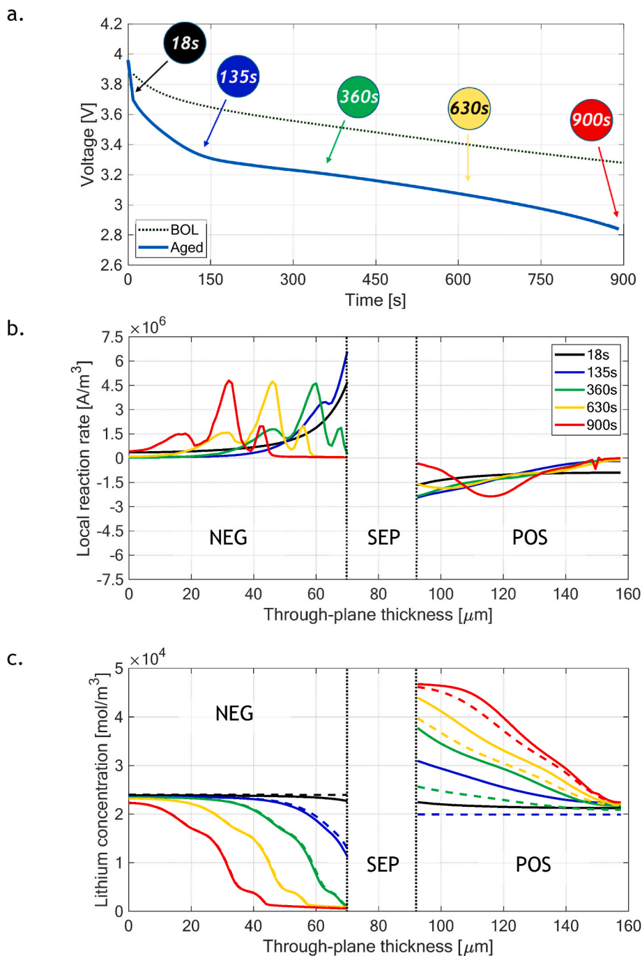
Fig. 3. Model simulation of aged cell cycled with IEC at 45 °C performing discharge 100 %–50 % SoC at 10 °C 2C. a) Voltage profile, highlighting specific time instants at which is shown: b) Volumetric current over electrode thickness. c) Lithium concentration on the surface (full lines) and center (dashed) of electrode particles.
