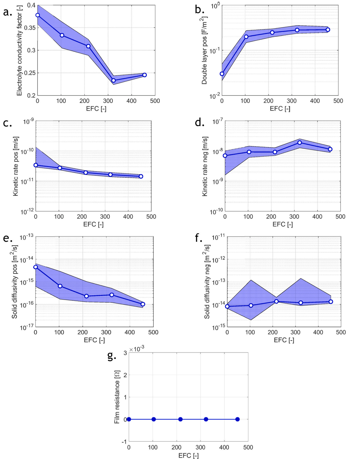
Fig. 2. Trend of physical parameters over EFC with uncertainty bands: a) electrolyte conductivity factor, b) positive electrode double layer capacitance, kinetic rate constant of c) positive and d) negative electrodes, solid-state diffusivity of e) positive and f) negative electrodes, g) negative electrode film resistance.
