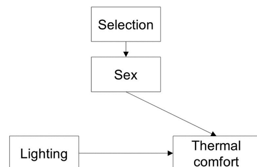
Fig. 4. Example selection diagram assuming that only sex modifies the effect of lighting on thermal comfort.
