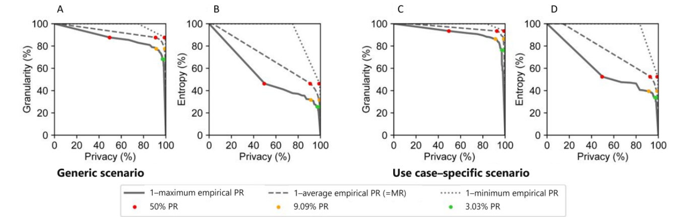
Figure 1. Privacy-utility curves based on general-purpose utility metrics. Granularity and nonuniform entropy served as general-purpose utility metrics. Privacy is demonstrated as 1–empirical maximum PR, average PR (ie, MR), and minimum PR. We used the anonymization processes implementing thresholds on PR for generating the points on the curve: 50% PR, 9.09% PR, and 3.03% PR. Results of granularity in the (A) generic and (C) use case-specific anonymized data sets and results of entropy in the (B) generic and (D) use case-specific anonymized data sets are shown. Results for 50% PR+MR were analogous and are illustrated in Figure S2 in Multimedia Appendix 1. The extreme points at (0,100) and (100,0) have been added to the graph but were not directly measured. MR: marketer risk; PR: prosecutor risk.
