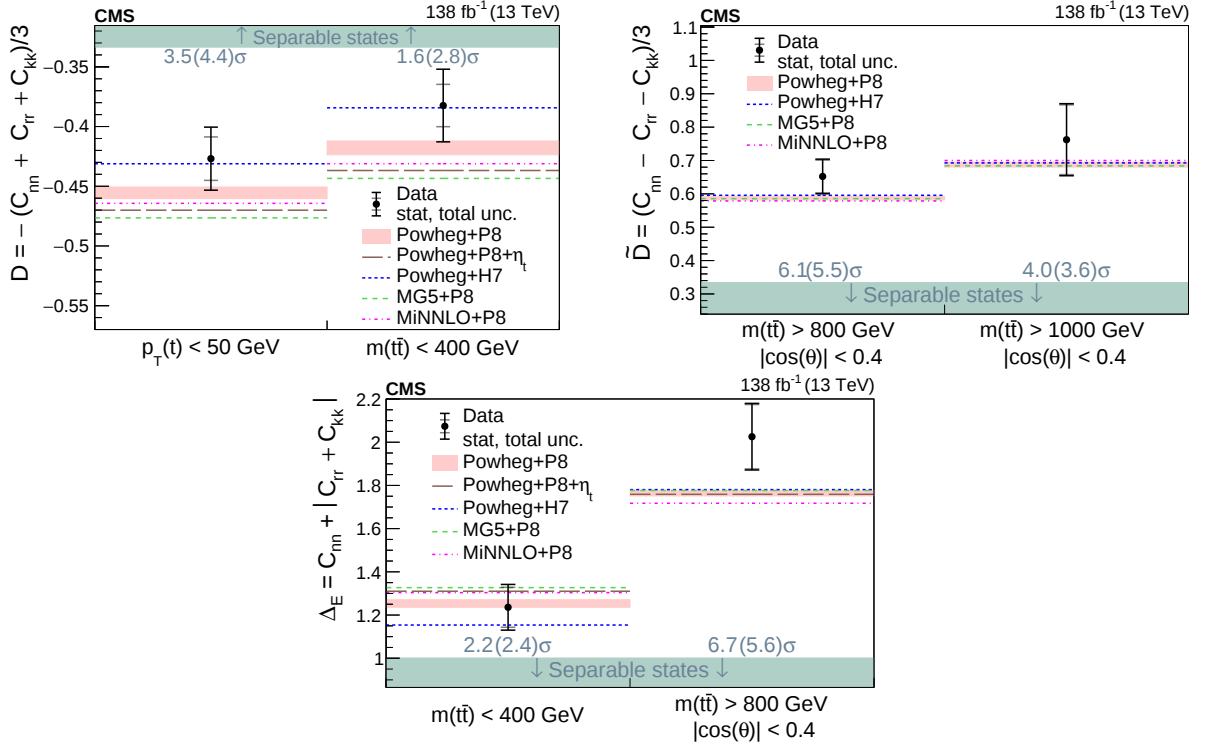
Figure 28: Entanglement results for the D measurement in the threshold region (upper left), \bar{D} measurement in the high- m(t\bar{t}) region (upper right), and the full matrix measurement in different m(t\bar{t}) regions (lower). The measurements (points) are shown with the statistical uncertainty (inner error bars) and total uncertainty (outer error bars) and compared to the predictions of POWHEG+PYTHIA, POWHEG+PYTHIA+ \eta_t , POWHEG+HERWIG, MADGRAPH5_aMC@NLO+PYTHIA, and MINNLO+PYTHIA. The POWHEG+PYTHIA prediction is displayed with the ME scale and PDF uncertainties, while for all other predictions only the central values are indicated. The observed (expected) significance of the deviation from the boundary of separable states (green region) is quoted in standard deviations ( \sigma ).
