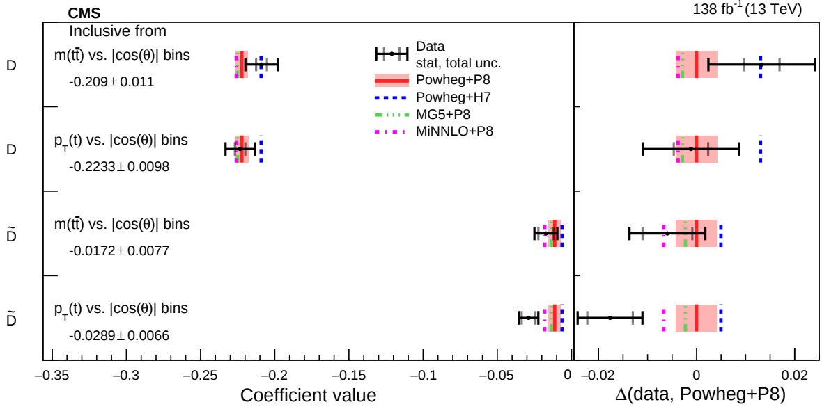
Figure 18: Results of the inclusive D and \bar{D} measurement obtained by combining the bins of the m(t\bar{t}) vs. |\cos(\theta)| and p_T(t) vs. |\cos(\theta)| measurements. The measurements (markers) are shown with the statistical uncertainty (inner error bars) and total uncertainty (outer error bars) and compared to the predictions of POWHEG+PYTHIA, POWHEG+HERWIG, MADGRAPH5_aMC@NLO+PYTHIA and MINNLO+PYTHIA. In the right panel, results are presented with the POWHEG+PYTHIA predictions subtracted. The POWHEG+PYTHIA prediction is displayed with ME scale and PDF uncertainties.
