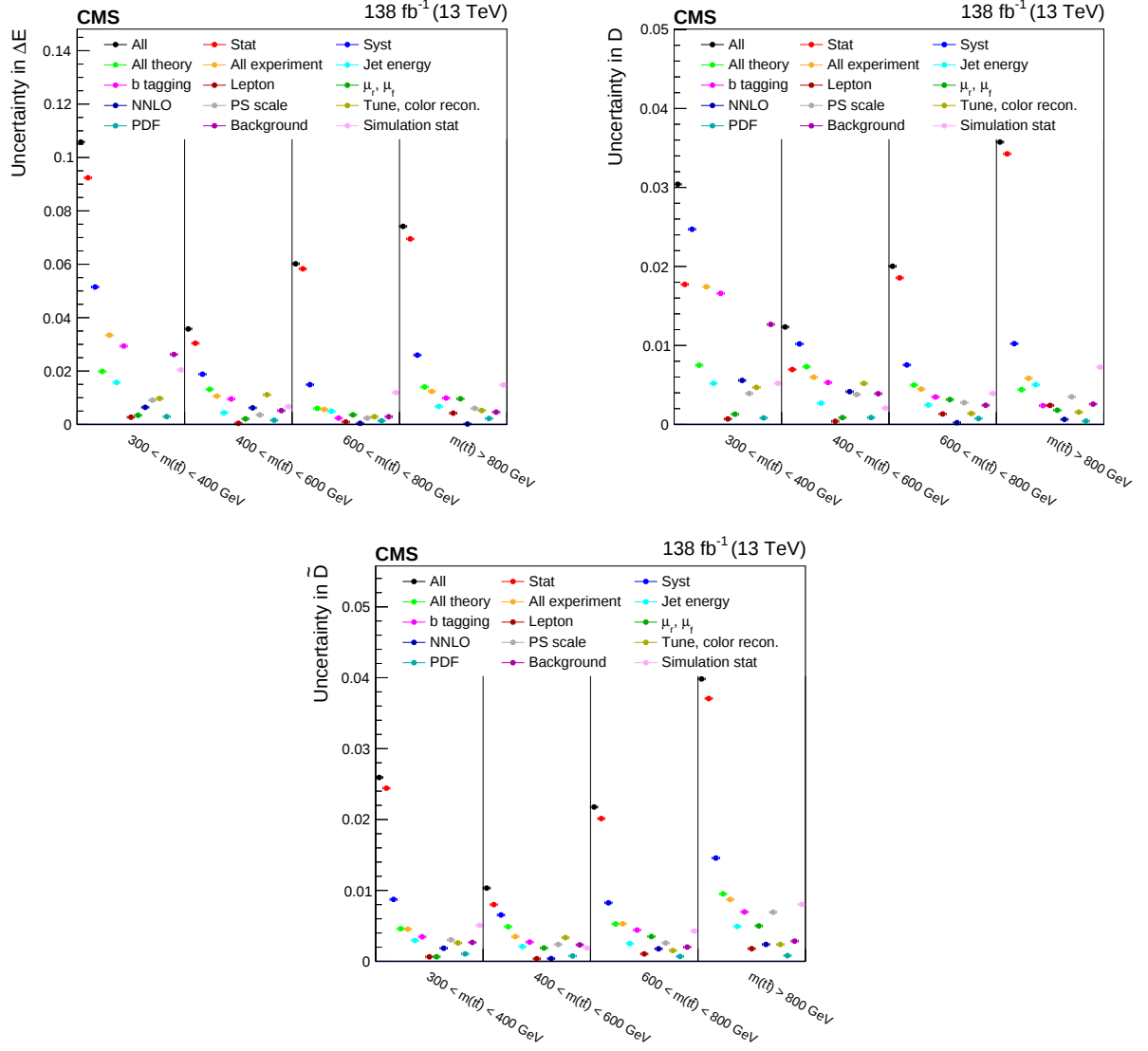
Figure 24: Contribution of individual uncertainty sources or groups of uncertainties in the measured \Delta E , D , and \bar{D} in bins of m(t\bar{t}) .
