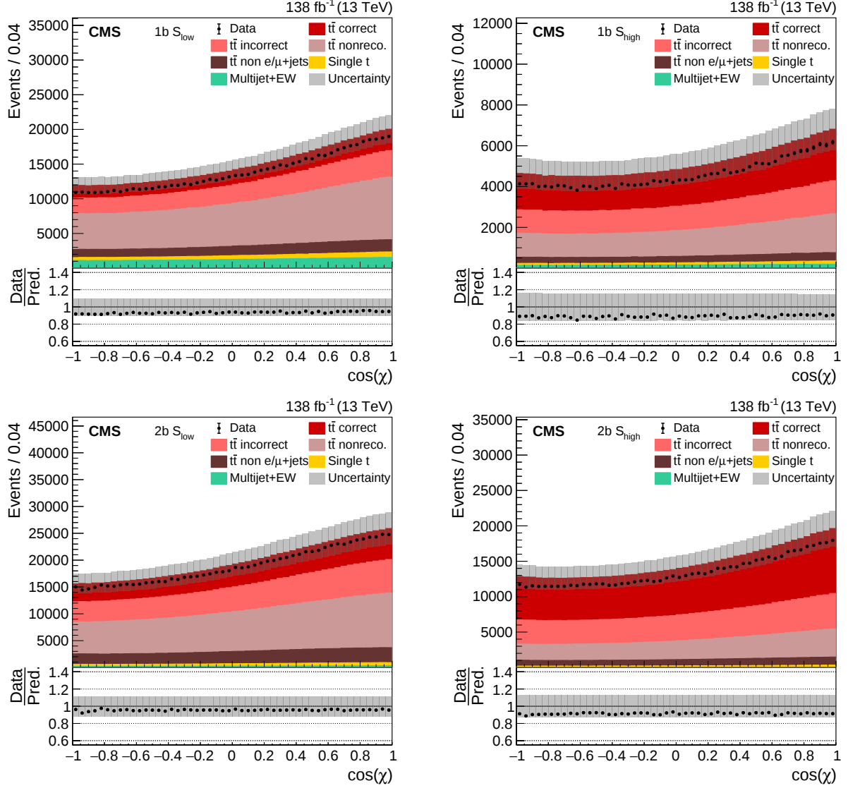
Figure 8: Distribution of \cos(\chi) in all four categories. The data (points) are compared to the prediction (stacked histograms). The \text{tt} and single top quark contributions are taken from the simulation, while the multijet+EW background is obtained from the CR. The \text{tt} contribution is split into the correctly and incorrectly reconstructed, “nonreconstructable”, and non e/\mu +jets events. The gray uncertainty band indicates the combined statistical and systematic uncertainties in the prediction. The vertical bars on the points show the statistical uncertainty of the data. Ratios to the predicted yields are provided in the lower panels.
