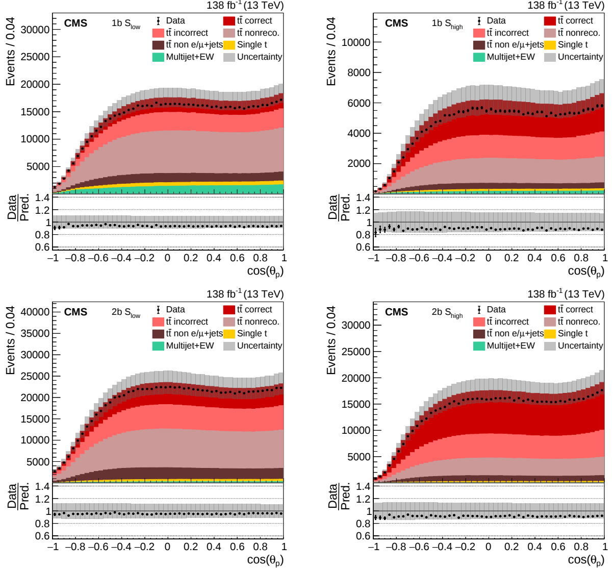
Figure 6: Distribution of \cos(\theta_p) in all four categories. The data (points) are compared to the prediction (stacked histograms). The t\bar{t} and single top quark contributions are taken from the simulation, while the multijet+EW background is obtained from the CR. The t\bar{t} contribution is split into the correctly and incorrectly reconstructed, “nonreconstructable”, and non e/\mu +jets events. The gray uncertainty band indicates the combined statistical and systematic uncertainties in the prediction. The vertical bars on the points show the statistical uncertainty of the data. Ratios to the predicted yields are provided in the lower panels.
