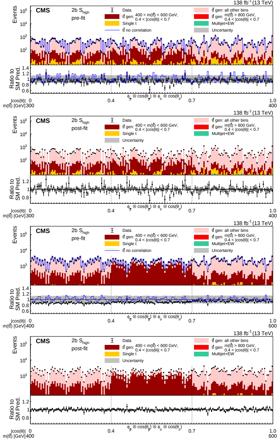
Figure 11: Pre- and post-fit distributions comparing the data (points) to the POWHEG+PYTHIA simulation (stacked histograms) for the full matrix measurement in bins of m(t\bar{t}) vs. |\cos(\theta)| in the 2b S_{\text{high}} category. The x axis shows the bins of the unrolled 4-dimensional distribution of \phi_{\bar{p}}, \cos(\theta_{\bar{p}}), \phi_p, and \cos(\theta_p) , listed from the outermost to the innermost variable in each of the m(t\bar{t}) vs. |\cos(\theta)| bins. The boundaries of the |\cos(\theta)| and m(t\bar{t}) bins are labeled and indicated by dashed and solid lines, respectively. For the illustration of resolution effects, t\bar{t} events generated in two selected m(t\bar{t}) vs. |\cos(\theta)| bins are shown in different shades of red. All other t\bar{t} contributions are shown in pink. A model without any polarization and spin correlation is shown as a blue line. The gray uncertainty band indicates the combined statistical and systematic uncertainties in the prediction. The vertical bars on the points show the statistical uncertainty. Ratios to the predicted yields are provided in the lower panels.
