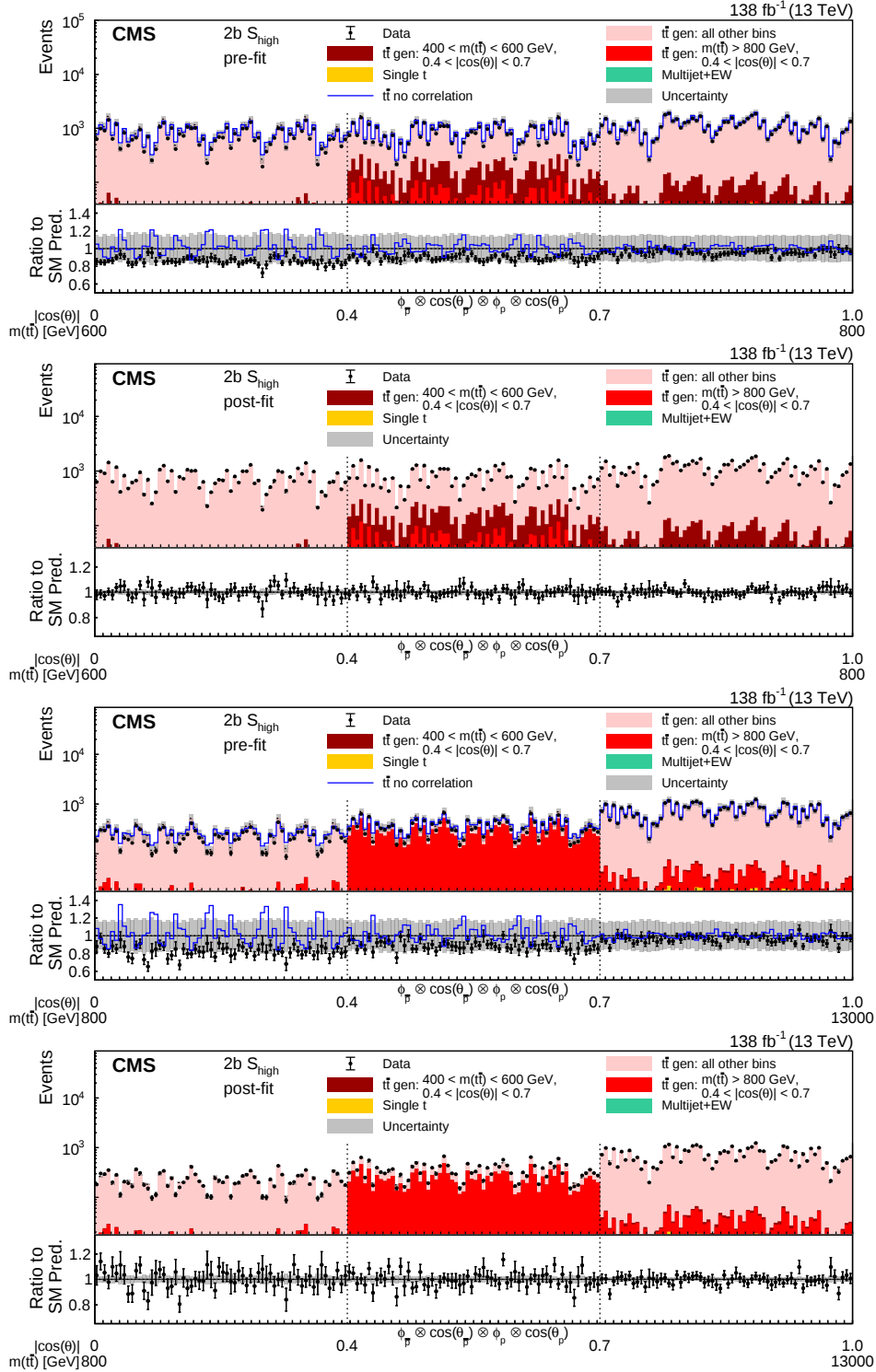
Figure 12: Pre- and post-fit distributions comparing the data (points) to the POWHEG+PYTHIA simulation (stacked histograms) for the full matrix measurement in bins of m(t\bar{t}) vs. |\cos(\theta)| in the 2b S_{\text{high}} category. The x axis shows the bins of the unrolled 4-dimensional distribution of \phi_{\bar{p}}, \cos(\theta_{\bar{p}}), \phi_p , and \cos(\theta_p) , listed from the outermost to the innermost variable in each of the m(t\bar{t}) vs. |\cos(\theta)| bins. The boundaries of the |\cos(\theta)| and m(t\bar{t}) bins are labeled and indicated by dashed and solid lines, respectively. For the illustration of resolution effects, t\bar{t} events generated in two selected m(t\bar{t}) vs. |\cos(\theta)| bins are shown in different shades of red. All other t\bar{t} contributions are shown in pink. A model without any polarization and spin correlation is shown as a blue line. The gray uncertainty band indicates the combined statistical and systematic uncertainties in the prediction. The vertical bars on the points show the statistical uncertainty. Ratios to the predicted yields are provided in the lower panels.
