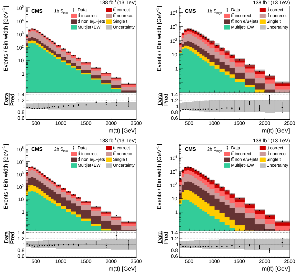
Figure 4: Distribution of m(t\bar{t}) in all four categories. The data (points) are compared to the prediction (stacked histograms). The t\bar{t} and single top quark contributions are taken from the simulation, while the multijet+EW background is obtained from the CR. The t\bar{t} contribution is split into the correctly and incorrectly reconstructed, “nonreconstructable”, and non e/μ+jets events. The gray uncertainty band indicates the combined statistical and systematic uncertainties in the prediction. The vertical bars on the points show the statistical uncertainty of the data. Ratios to the predicted yields are provided in the lower panels.
