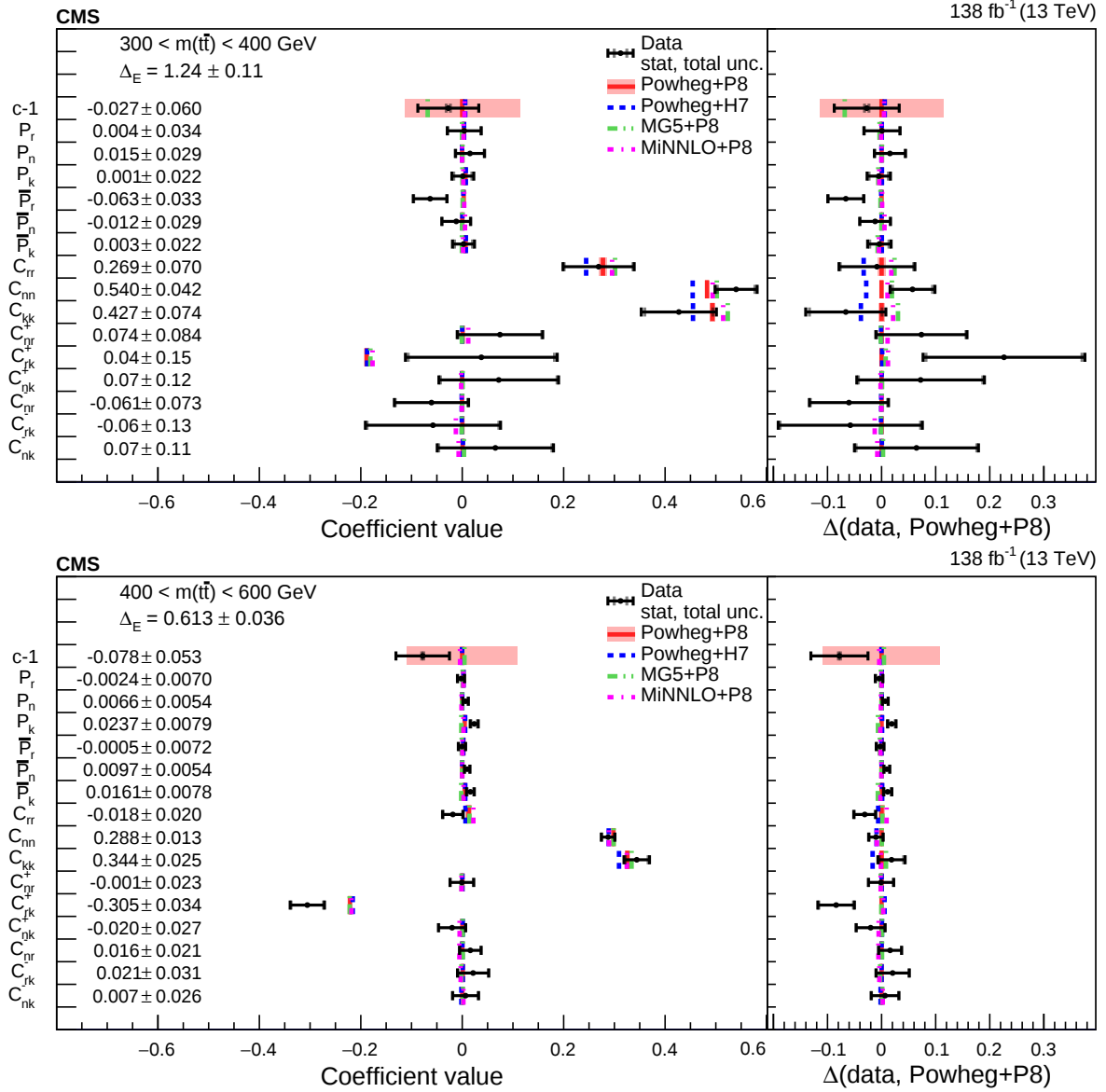
Figure 19: Results of the full matrix measurement in bins of m(\text{t}\bar{\text{t}}) . The measurements (markers) are shown with the statistical uncertainty (inner error bars) and total uncertainty (outer error bars) and compared to the predictions of POWHEG+PYTHIA, POWHEG+HERWIG, MADGRAPH5_aMC@NLO+PYTHIA and MINNLO+PYTHIA. In the right panels, results are presented with the POWHEG+PYTHIA predictions subtracted. The POWHEG+PYTHIA prediction is displayed with ME scale and PDF uncertainties. The values of \Delta_E are displayed for each measurement.
