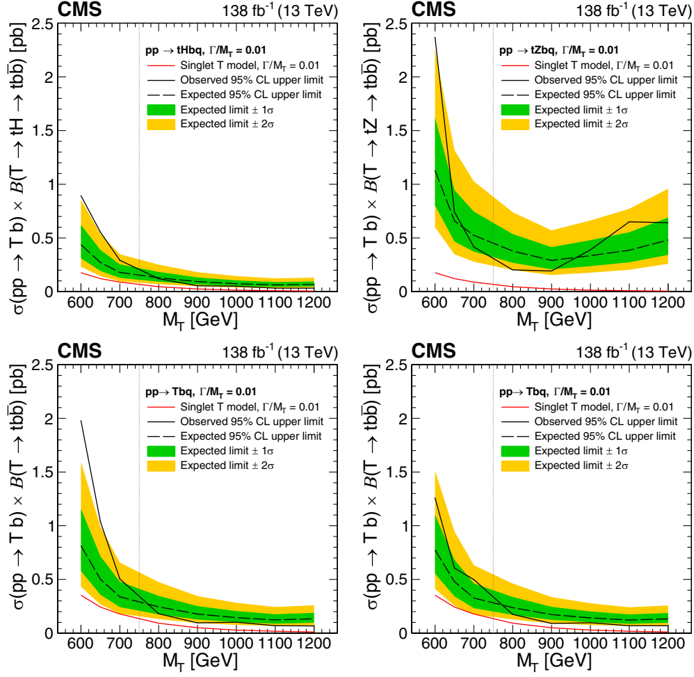
FIG. 7. The observed and expected 95% CL limits on the cross section for associated production with a b quark for final states tHbq (upper left), tZbq (upper right), their sum tHbq + tZbq (lower left), and tHbq + tZbq including the leakage of tH events into the tZ channel (lower right) for different assumed values of the T quark mass. The vertical dashed line represents the crossover point in sensitivity: for masses to the left, the low-mass selection is used to set limits, while for masses to the right, the high-mass selection is used to set limits. The red lines indicate the theoretical cross section for the singlet model [9].
