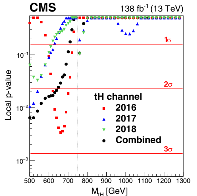
FIG. 6. Observed p -values when considering the tH channel for each year and their combination.
