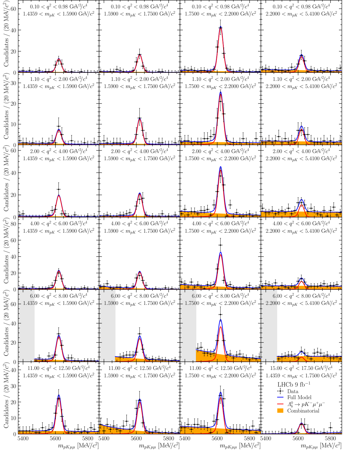
Figure 2. Mass distributions of selected \Lambda_b^0 \rightarrow p K^- \mu^+ \mu^- decay candidates in bins of m_{pK} and q^2 . The data are overlaid with the result of the fit described in the text. The shaded regions are populated by poorly reconstructed \Lambda_b^0 \rightarrow J/\psi p K^- decays and are excluded from the analysis.
