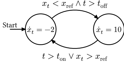
Figure 3: Automaton of the temperature control system
