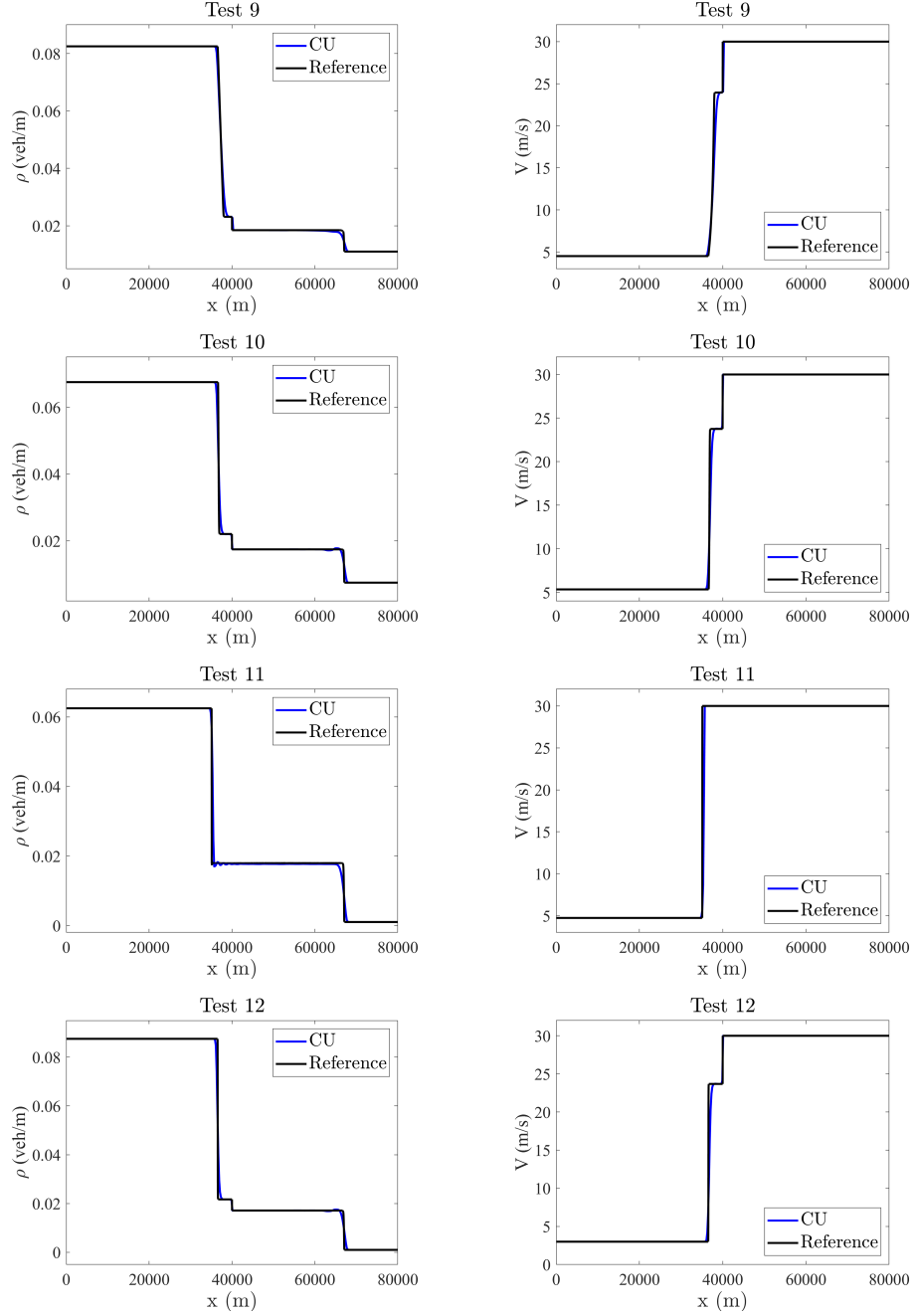
Figure 4.3: Example 1, Tests 9–12: \rho (left column) and V (right column) at time T_{\text{final}} = 900 .
