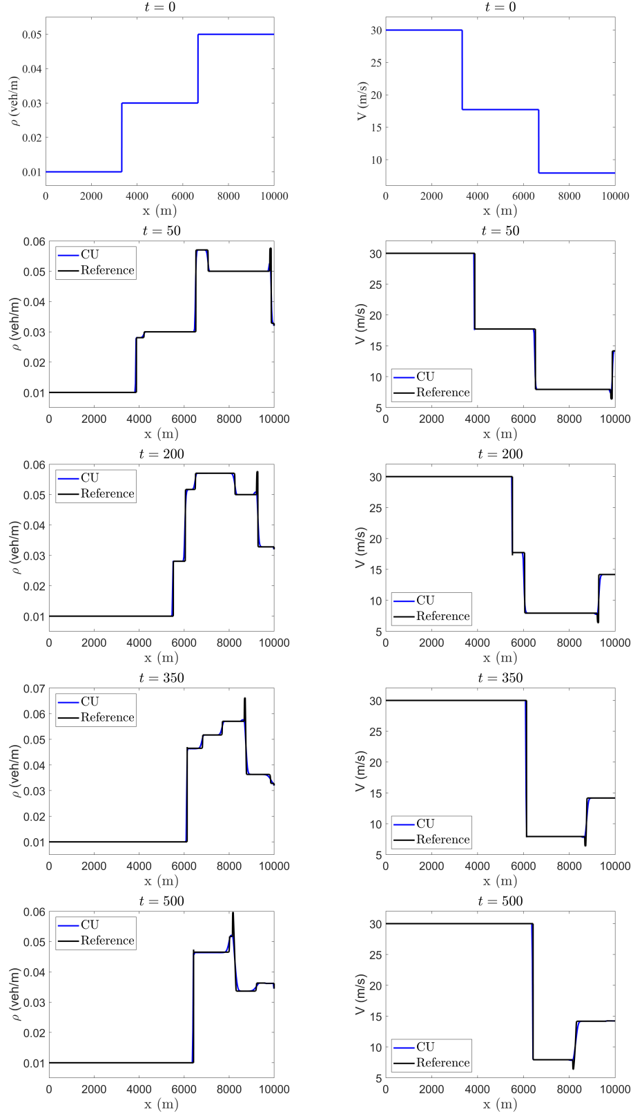
Figure 4.6: Example 3: \rho (left column) and V (right column) at times t = 0 (top row), t = 50 (second row), t = 200 (third row), t = 350 (fourth row), and t = 500 (bottom row).
