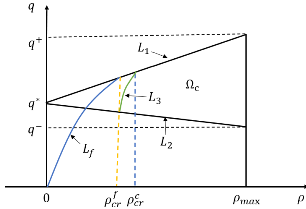
Figure 2.1: (\rho, q) -diagram of the phase-transition traffic flow model.
