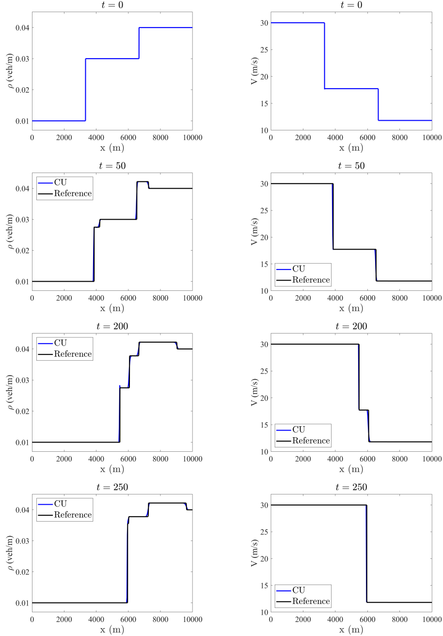
Figure 4.4: Example 2: \rho (left column) and V (right column) at times t = 0 (top row), t = 50 (second row), t = 200 (third row), and t = 250 (bottom row).
