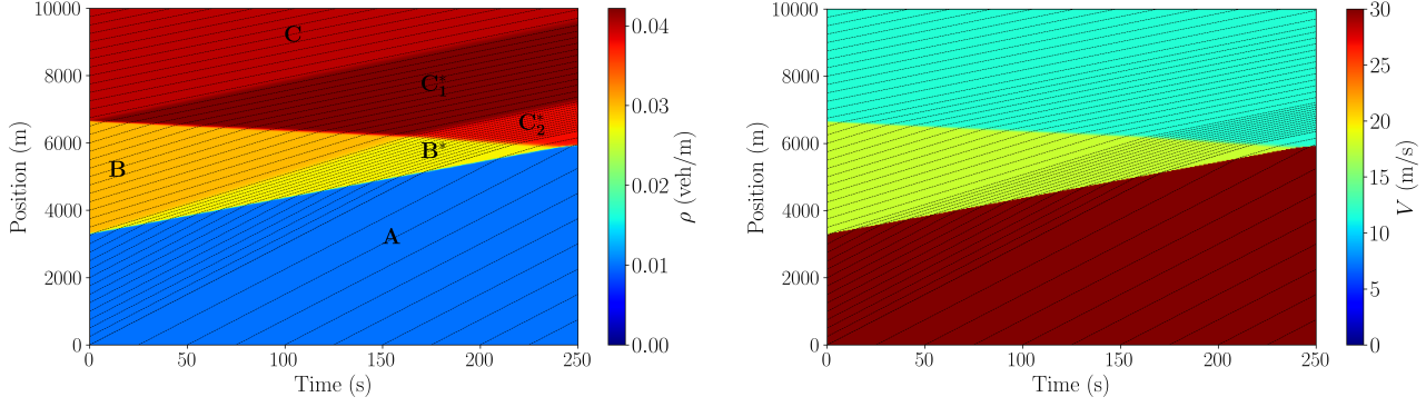
Figure 4.5: Example 2: Spatio-temporal evolution of \rho (left) and V (right) for t \in [0, 250] .
