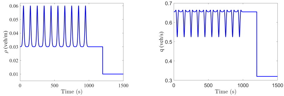
Figure 4.9: Example 4: Boundary conditions for \rho and q at the right end of the computational domain.
