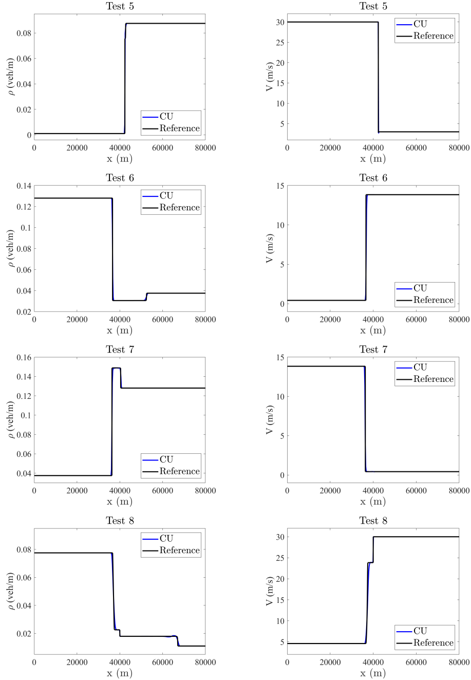
Figure 4.2: Example 1, Tests 5–8: \rho (left column) and V (right column) at time T_{\text{final}} = 900 .
