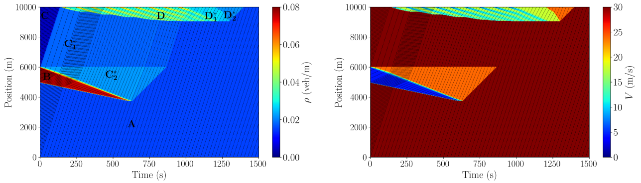
Figure 4.10: Example 4: Spatio-temporal evolution of \rho (left) and V (right) for t \in [0, 1500] .
