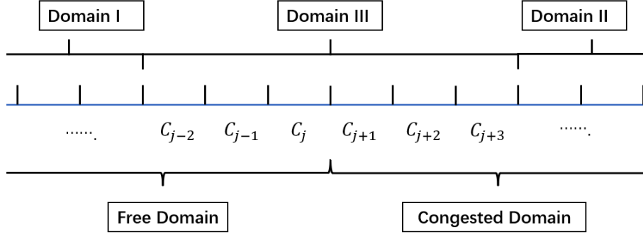
Figure 3.1: Domains I, II, and III of the phase-transition traffic flow model.
