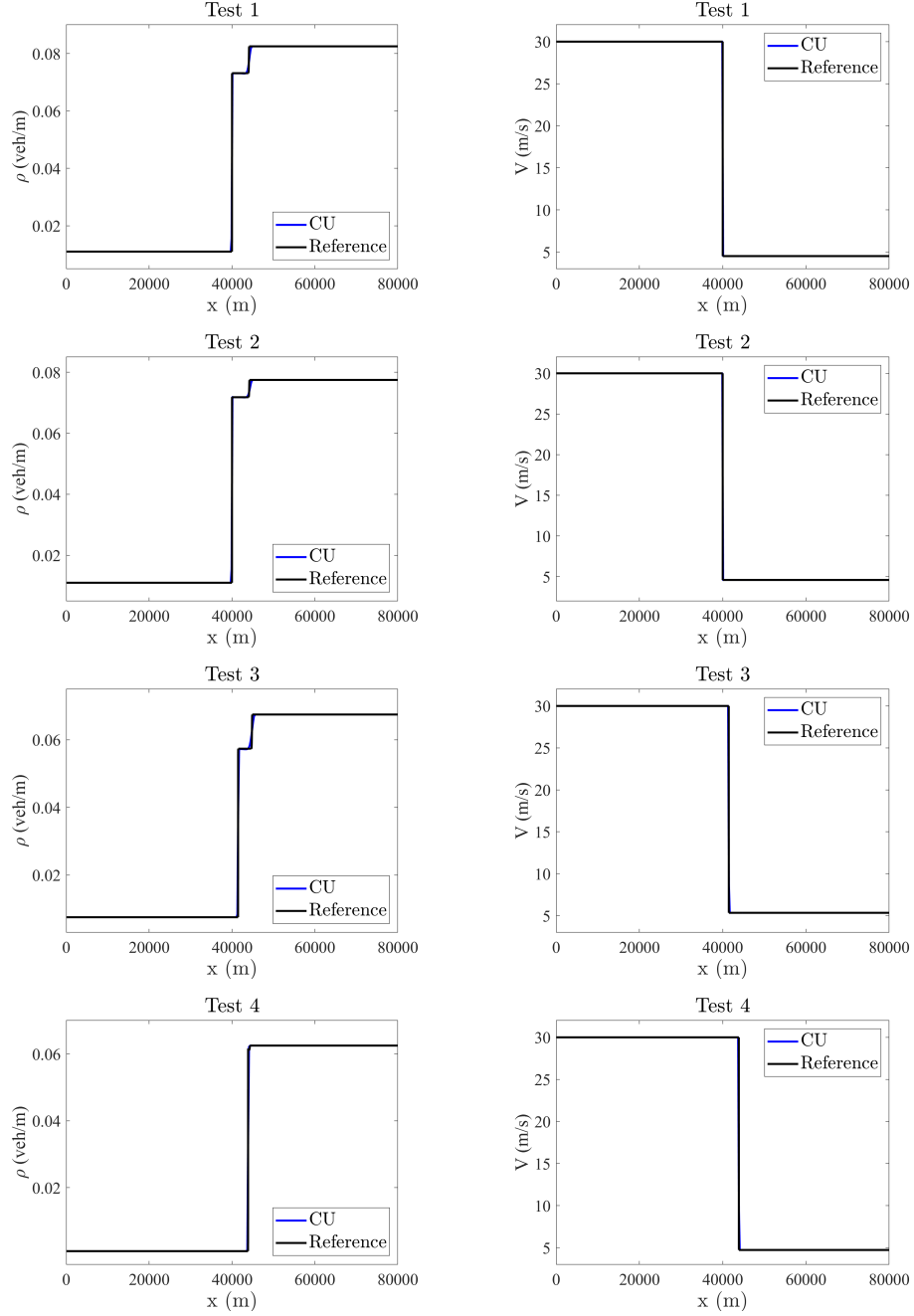
Figure 4.1: Example 1, Tests 1–4: \rho (left column) and V (right column) at time T_{\text{final}} = 900 .
