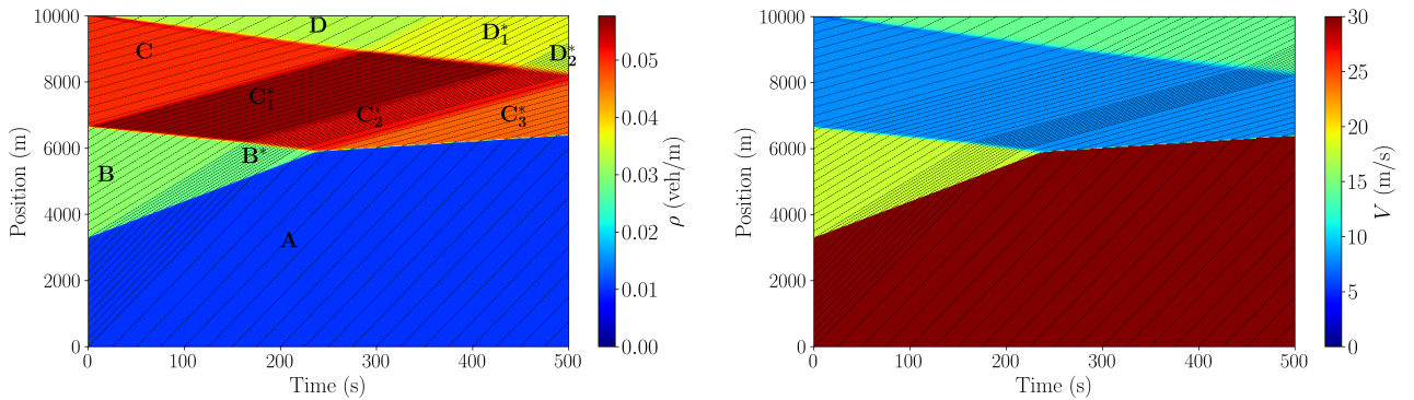
Figure 4.7: Example 3: Spatio-temporal evolution of \rho (left) and V (right) for t \in [0, 500] .
