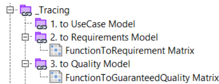
Figure 8.17: The matrices created to refer to models of other DSML building blocks.
