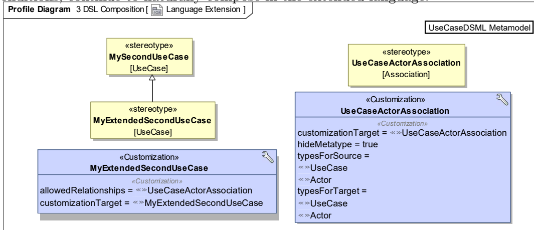
Figure 4.9: An example of the MySecondUseCase being extended and customised to MyExtendedSecondUseCase with an association dependency UseCaseActorAssociation between a UseCase and an Actor. Figure adapted from [BGJ + 23].
