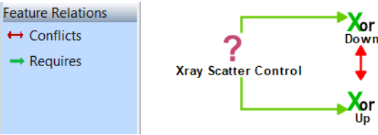
Figure 8.14: A feature model showing relations between an optional and Xor features.
