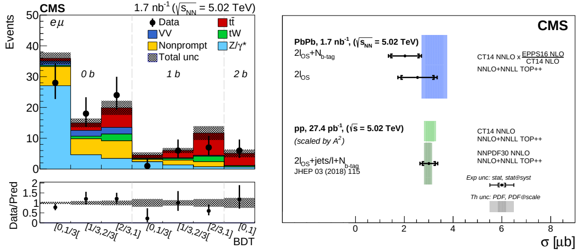
Figure 66: Left: Observed and postfit predicted BDT discriminator distributions in the e^\pm\mu^\pm final state separately in the 0b-, 1b-, and 2b-tagged jet multiplicity categories. The data are shown with markers, and the signal and background processes with filled histograms. The vertical bars on the markers represent the statistical uncertainties in data. The hatched regions show the uncertainties in the sum of t\bar{t} signal and backgrounds. The lower panel displays the ratio between the data and the predictions, including the t\bar{t} signal, with bands representing the uncertainties in the postfit predictions. Right: Inclusive t\bar{t} cross sections measured with two methods in the combined e^\pm\mu^\pm , \mu^+\mu^- , and e^+e^- final states in PbPb collisions at \sqrt{s_{NN}} = 5.02 TeV, and pp results at \sqrt{s} = 5.02 TeV (scaled by A^2 ). The measurements are compared with theoretical predictions at NNLO+NNLL accuracy in QCD. The inner (outer) experimental uncertainty bars include statistical (statistical and systematic, added in quadrature) uncertainties. The inner (outer) theoretical uncertainty bands correspond to nPDF or PDF (PDF and scale, added in quadrature) uncertainties. (Figures adapted from Ref. [149].)
