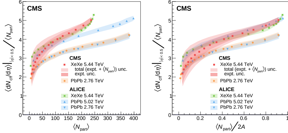
Figure 33: Average dN_{ch}/d\eta at midrapidity normalised by \langle N_{part} \rangle , shown as a function of \langle N_{part} \rangle (left) and \langle N_{part} \rangle / 2A (right), where A is the mass number of the nuclei. (Figures adapted from Ref. [231].)
