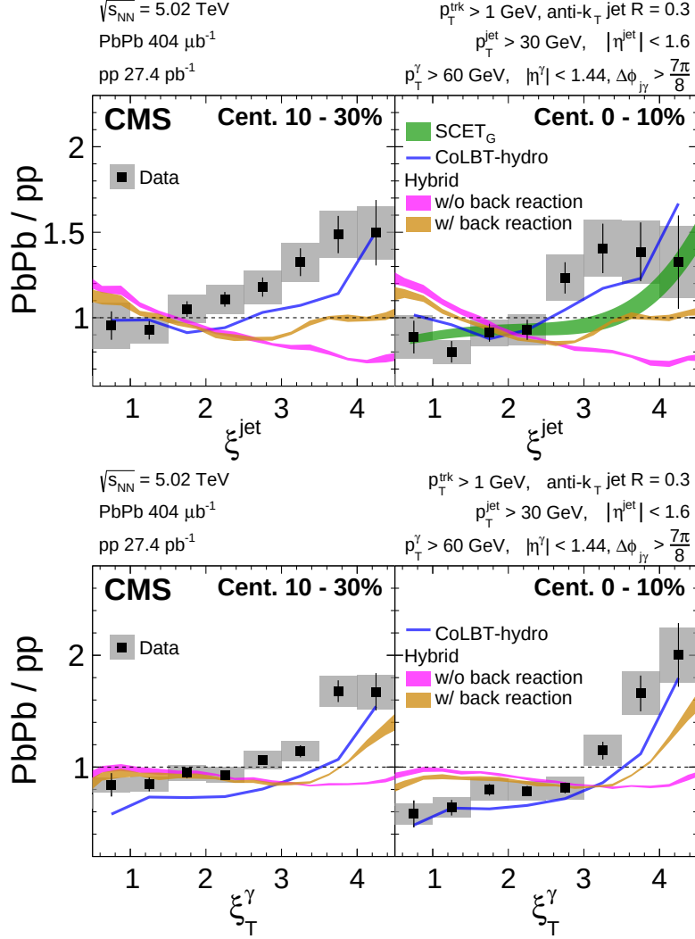
Figure 68: Comparison of \gamma -tagged fragmentation functions in centrality bins 10–30% (left) and 0–10% (right) as a function of the observables \xi_{\text{jet}}^{\gamma} (upper), defined in Eq. (21), and \xi_T^{\gamma} (lower), defined in Eq. (22). For comparison, curves from the theoretical models SCET G [352], CoLBT-hydro [383–385], and HYBRID [386] are overlaid. The widths of the bands represent variations of the coupling strength in the SCET G case and of the dimensionless parameter \kappa in the HYBRID case. Vertical bars and shaded boxes represent the statistical and systematic uncertainties, respectively. (Figures adapted from Ref. [387].)
