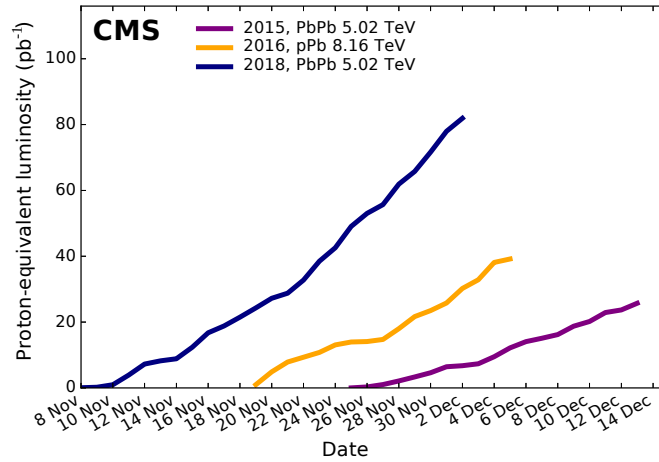
Figure 1: Integrated luminosity delivered to the CMS experiment with PbPb and pPb collisions at \sqrt{s_{\text{NN}}} = 5.02 [48] and 8.16 TeV [49], respectively, as a function of time during the LHC Run 2 period. The years of data collection shown correspond to 2015 (purple), 2016 (orange), and 2018 (navy blue). This plot shows the proton-equivalent luminosity, i.e., the values for the PbPb data have been scaled by A^2 = 208^2 and the values for the pPb data by A = 208 .
