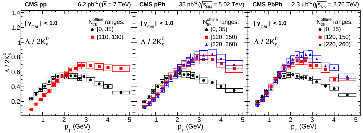
Figure 87: Ratios of p_T spectra for \Lambda/2K_S^0 in the center-of-mass rapidity range |y_{\text{cm}}| < 1.0 for pp collisions at \sqrt{s} = 7 TeV (left), pPb collisions at \sqrt{s} = 5.02 TeV (middle), and PbPb collisions at \sqrt{s_{\text{NN}}} = 2.76 TeV (right). Two (for pp) or three (for pPb and PbPb) representative multiplicity intervals are presented. (Figure adapted from Ref. [504].)
