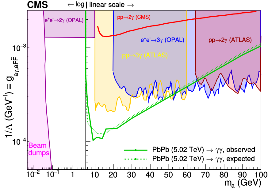
Figure 111: Exclusion limits at 95% CL in the ALP-photon coupling g_{a\gamma} vs. ALP mass m_a plane, for the operators a\tilde{F}/4\Lambda assuming ALP coupling to photons only, derived in Refs. [587, 593] from measurements at beam dumps [594], in e^+e^- collisions at LEP 1 [593] and LEP 2 [595], and in pp collisions at the LHC [574, 596, 597], and compared to the limits obtained from Ref. [548]. (Figure adapted from Ref. [548].)
