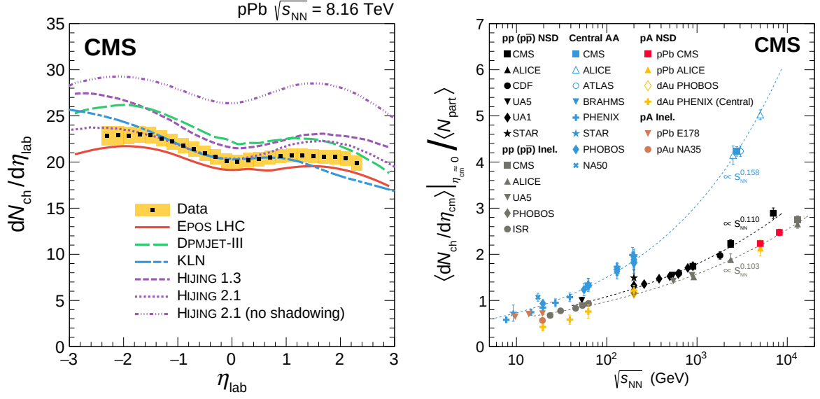
Figure 85: Left: Pseudorapidity density of charged hadrons in the range |\eta_{lab}| < 2.4 in pPb collisions at 8.16 TeV. The results are compared to predictions from the MC event generators EPOS LHC [123, 476] (v3400), HIJING [124] (versions 1.3 [477] and 2.1 [478]), and DPMJET-III [479], as well as from the KLN model [257]. The shaded boxes around the data points indicate their systematic uncertainties. The proton beam goes in the positive \eta_{lab} direction. Right: Comparison of the measured density at midrapidity, scaled by N_{part} in pPb [480, 481], pAu [482], dAu [483–485] and central heavy ion collisions [111, 234, 484, 486–497], as well as NSD [235, 236, 238, 239, 497–499] and inelastic [234, 237, 238, 500, 501] pp collisions. The dashed curves, included to guide the eye, are from Refs. [237, 494].
