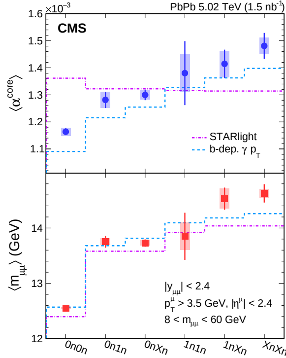
Figure 103: Neutron multiplicity dependence of the (upper) average acoplanarity \langle \alpha^{\text{core}} \rangle and (lower) average invariant mass \langle m_{\mu\mu} \rangle of \mu^+\mu^- pairs in ultraperipheral PbPb collisions at \sqrt{s_{\text{NN}}} = 5.02 TeV. The vertical lines on data points depict the statistical uncertainties while the systematic uncertainties of the data are shown as shaded areas. The dot-dashed line shows the STARLIGHT MC prediction and the dashed line corresponds to the LO QED calculation of Ref. [571]. The calculation incorporating Sudakov radiative corrections is also compared to data in Ref. [218], leading to an overall better agreement. (Figure adapted from Ref. [218].)
