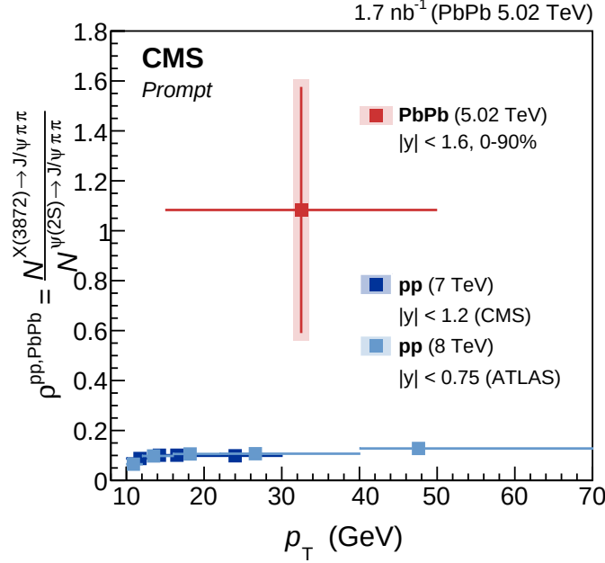
Figure 79: The yield ratio \rho^{\text{PbPb}} of prompt X(3872) over \psi(2S) production in pp and PbPb collisions as a function of p_T . (Figure adapted from Ref. [431].)
