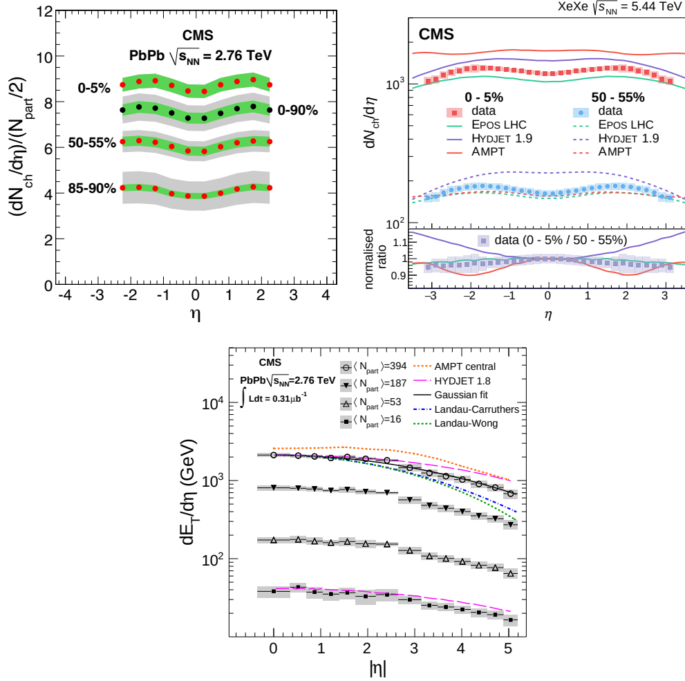
Figure 32: Distributions (dN_{\text{ch}}/d\eta)/(N_{\text{part}}/2) in 2.76 TeV PbPb (top left) and dN_{\text{ch}}/d\eta in 5.44 TeV XeXe (top right) collisions, and dE_T/d\eta in 2.76 TeV PbPb collisions (bottom) as functions of \eta in various centrality bins. The inner green band in the left panel shows the measurement uncertainties affecting the scale of the measured distribution, while the outer gray band shows the full systematic uncertainty, i.e. affecting both the scale and the slope. (Figures adapted from Refs. [111, 231, 232].)
