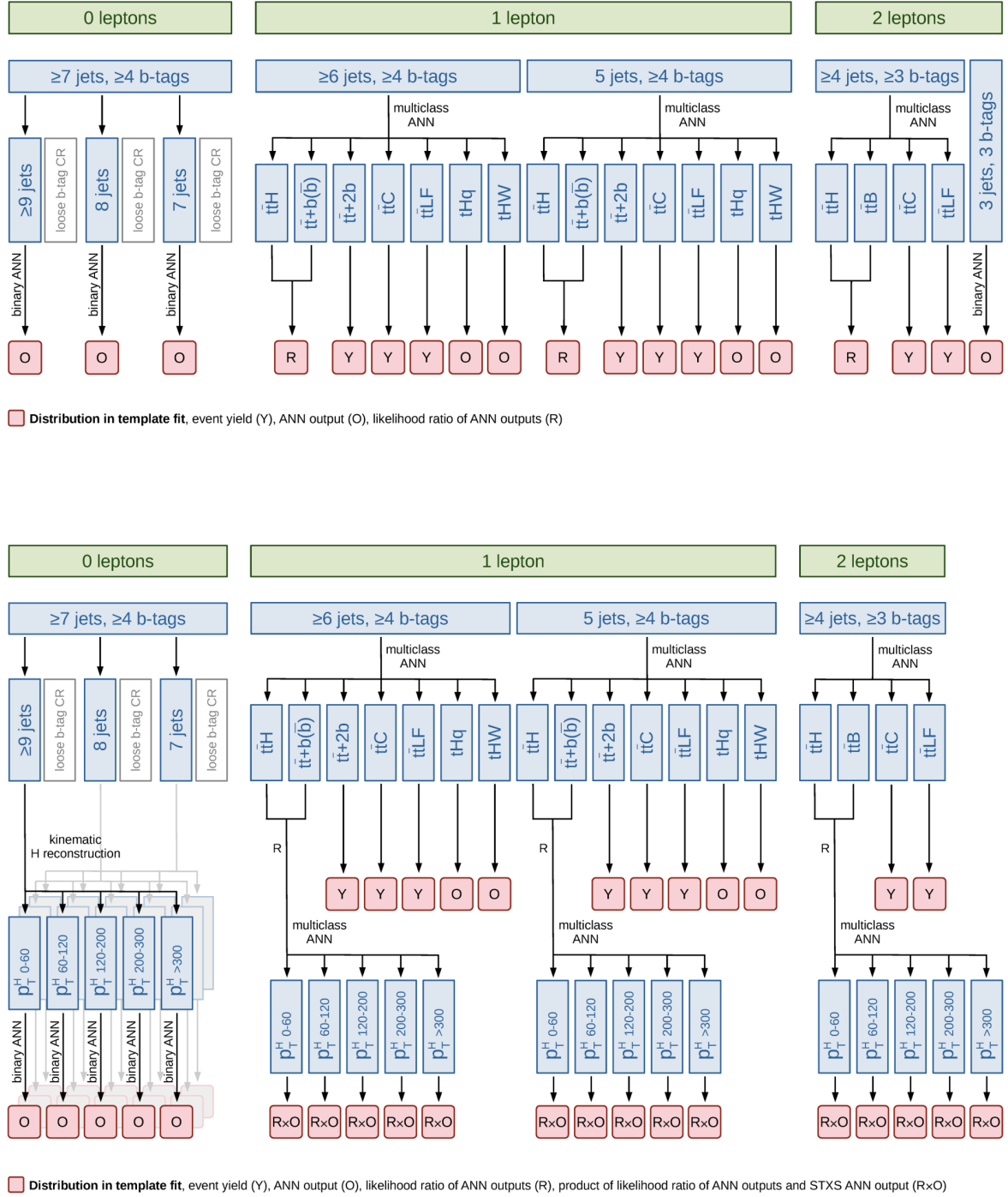
Figure 5. Illustration of the analysis strategy for the inclusive t\bar{t}H and tH production rate, coupling, and CP measurements (upper), and for the t\bar{t}H STXS measurement (lower). Details of the ANNs and the definition of the likelihood ratio are given in the text. The procedure is applied separately for the three years of data taking.
