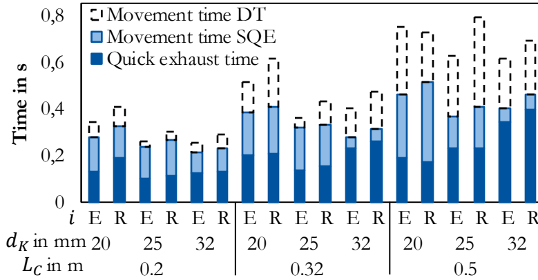
Figure 4: Movement time and quick-exhaust time of cylinders with different piston diameters d_K and cylinder lengths L_C , equipped with a switchable quick-exhaust (SQE) valve and a moving mass of 10 kg. The index i denotes the extension stroke ( i = E ) or the retraction stroke ( i = R ).
