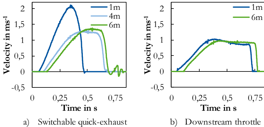
Figure 6: Cylinder velocity with varying pneumatic line lengths.
