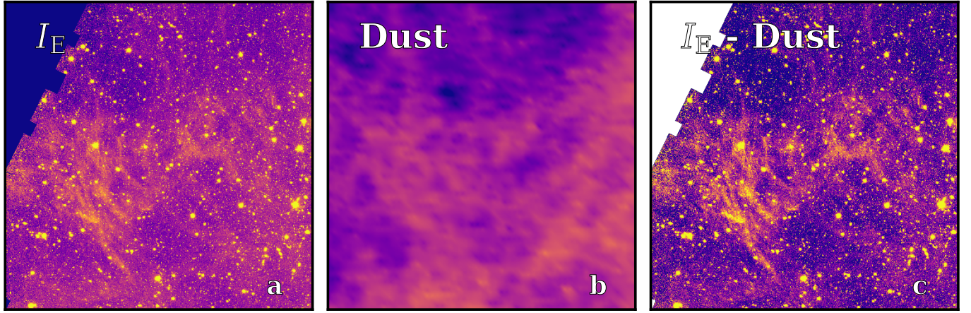
Fig. A.1. Example of the problem of using the WISE dust maps to correct for cirrus in the Euclid images. Panel a shows a region of 25' \times 25' in the I_E band. Panel b shows the corresponding WISE dust map for the region. Panel c shows the result of subtracting the WISE dust map from the I_E image. The residual shows cirrus filaments that the WISE map does not capture.
