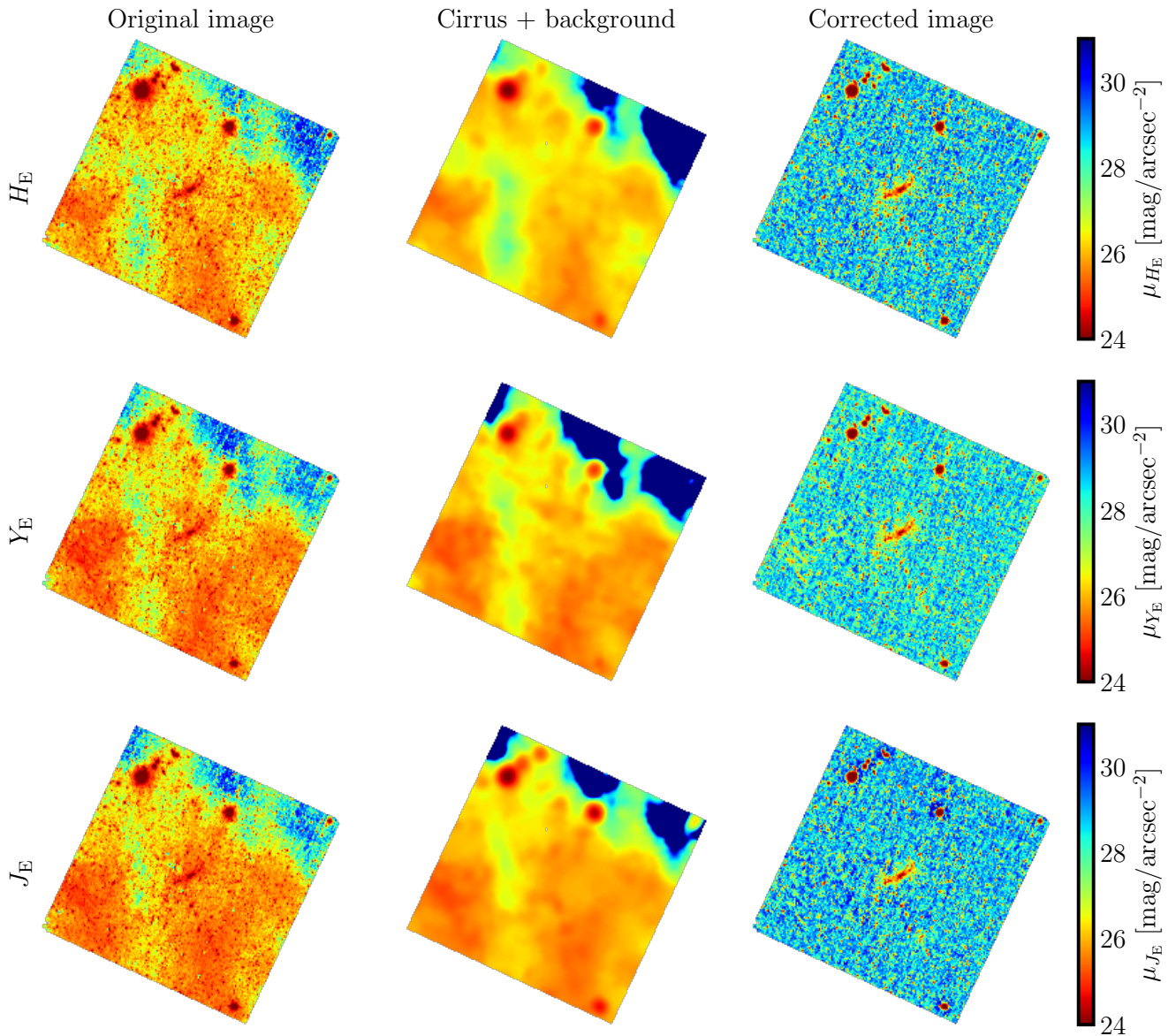
Fig. 3. Effect of cirrus removal for all NISP filter images. From left to right: original image; cirrus+background map; cirrus-corrected image. The angular size of the images is 0.7 \times 0.7 .
