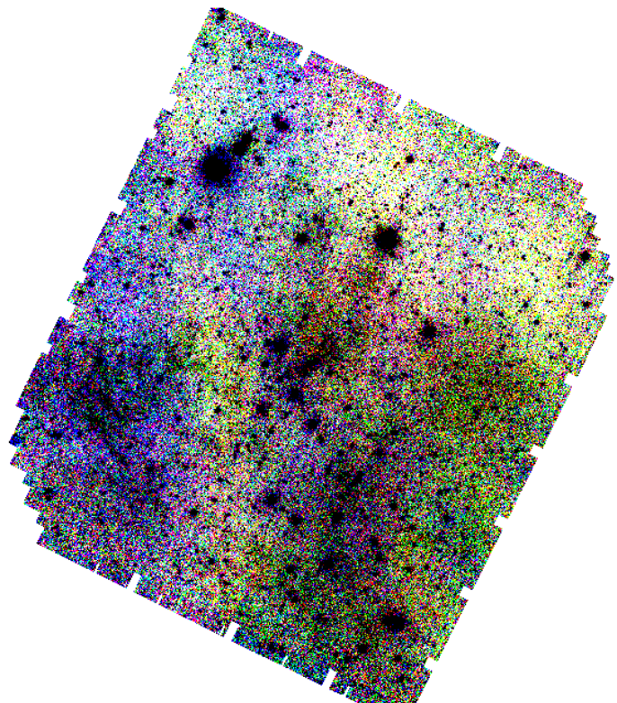
Fig. 2. RGB image of the A 2390 galaxy cluster Euclid FoV. The contrast is greatly enhanced to highlight large-scale colour variations (due to cirrus and background inhomogeneities) across the whole image in the LSB regime. Blue is VIS, green is the J_E band, and red is the H_E band. North is up and east is to the left.
