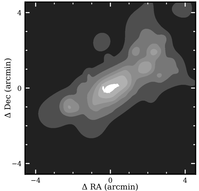
Fig. 7. A 9' \times 9' ( 2 \text{ Mpc} \times 2 \text{ Mpc} ) region around A 2390 on the DAWIS BCG+ICL J_E map.
