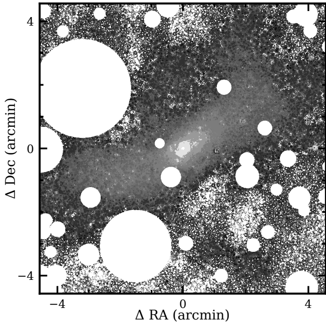
Fig. 6. A 9' \times 9' ( 2 \text{ Mpc} \times 2 \text{ Mpc} ) region around A 2390 on the CICLE BCG+ICL J_E map. The white circles are masks over stars in the FoV.
