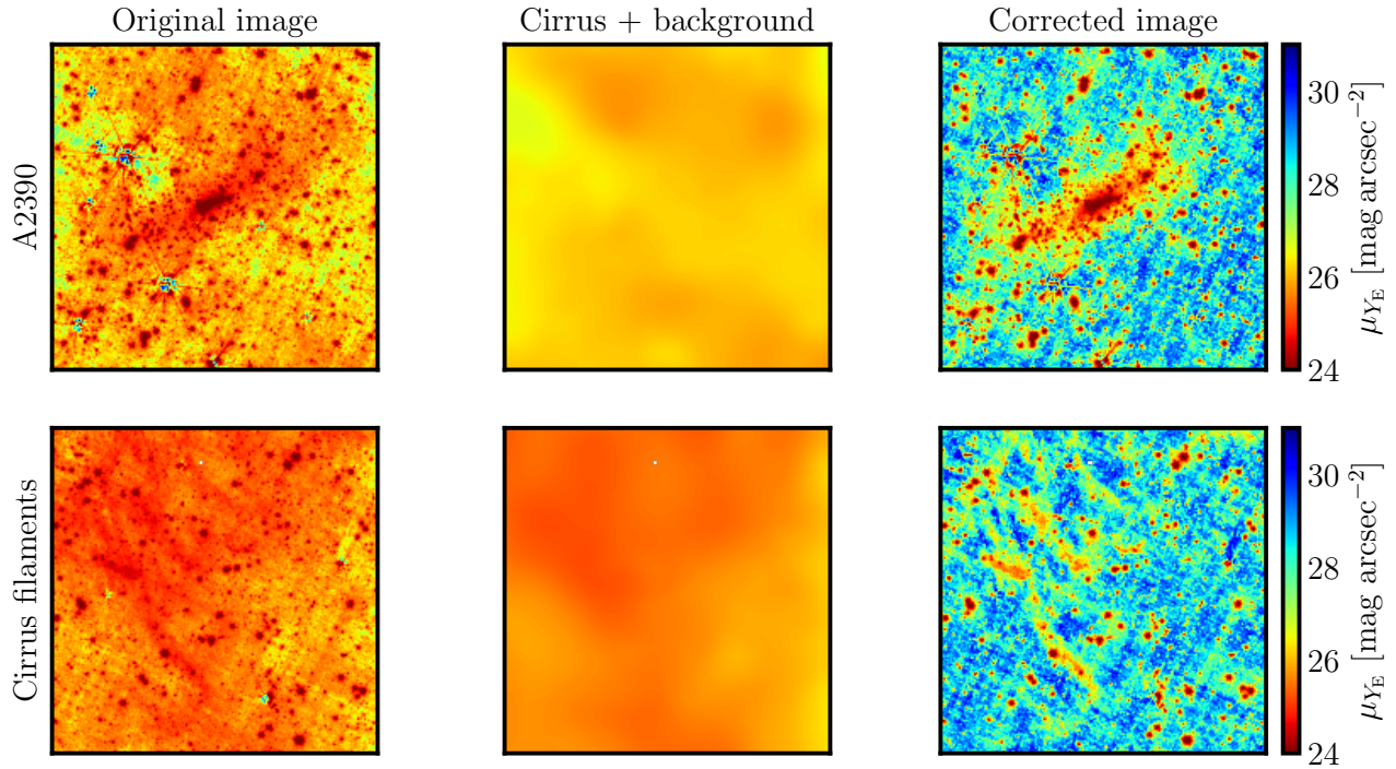
Fig. 4. Zoom-in on regions of interest in the Y_E band, which displays the most cirrus residuals after correction. The top row shows a 12.5 \times 12.5 image centred on A 2390. The bottom row shows a high-intensity cirrus region ( 12.5 \times 12.5 ) situated in the east of the image, displaying obvious small-scale cirrus residuals in the corrected image. From left to right: original image; cirrus model; cirrus-corrected image.
