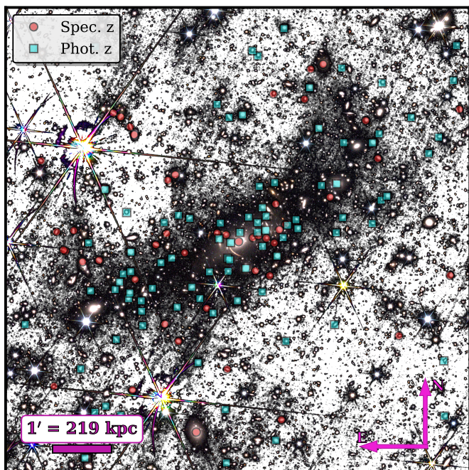
Fig. 1. Image of the 9'.1 \times 9'.1 (2 Mpc \times 2 Mpc, approximately 0.5R_{200} of the cluster) region around A 2390. The image is a combination of an RGB image of the PSF-subtracted NISP images and a J_E + H_E black and white background. Cluster members are colour-coded according to whether their redshift is spectroscopic (red circles) or photometric (teal squares). North is up and east is to the left. This image highlights the importance of removing bright stars close to the cluster centre to study the diffuse light (see Sect. 3.1).
