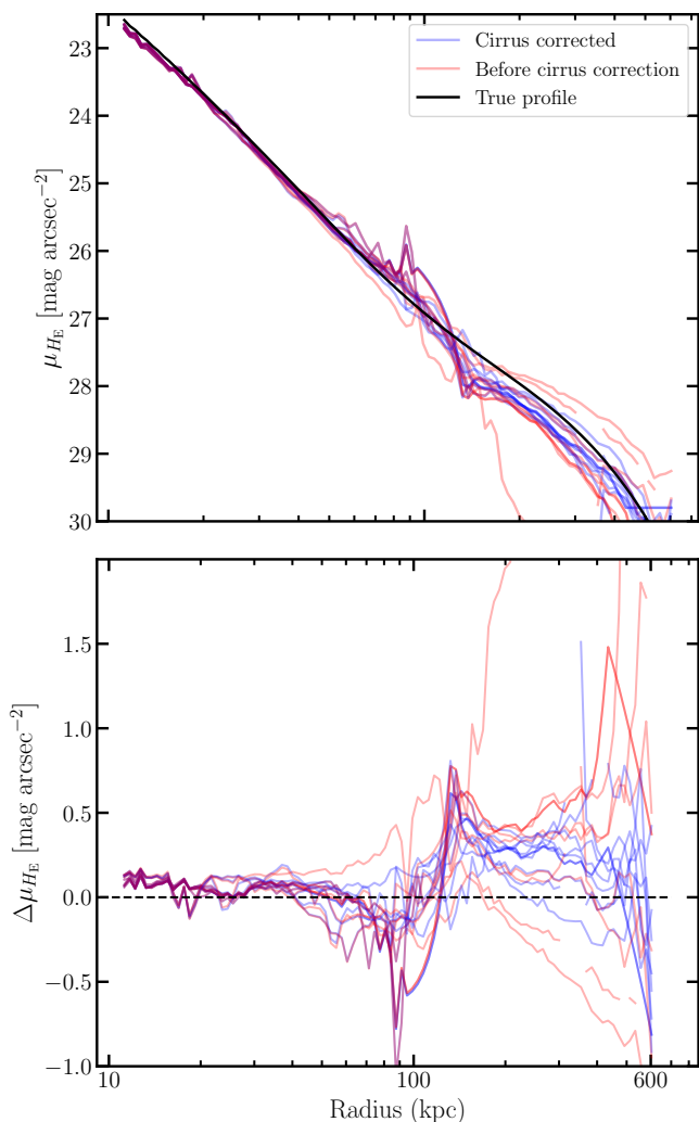
Fig. 5. Top: mock cluster radial profiles in the H_E band before (red) and after (blue) cirrus correction. The true BCG+ICL light profile is shown as a black line. Bottom: difference between true BCG+ICL light profile and the measured BCG+ICL profiles.
