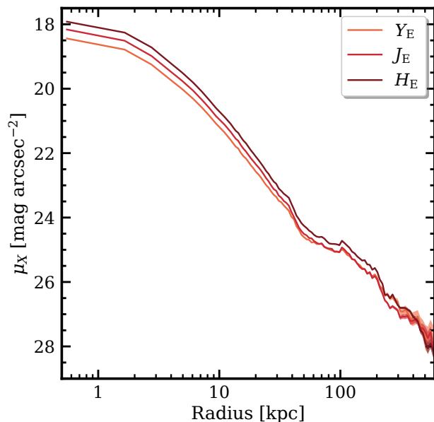
Fig. 10. Surface brightness radial profiles for the BCG+ICL of A 2390 from the 1-D method Ahad. The plot shows the profiles for the Y_E (orange), J_E (red), and H_E (dark red) NISP bands.
