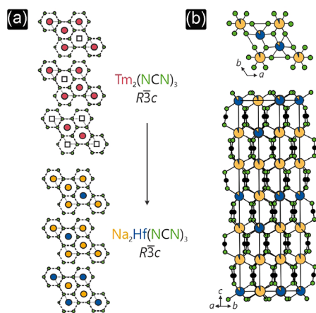
Figure 3. a) Schematic structural relation between \text{Tm}_2(\text{NCN})_3 and \text{Na}_2\text{Hf}(\text{NCN})_3 along the stacking direction. b) Crystal structure of \text{Na}_2\text{Hf}(\text{NCN})_3 .
