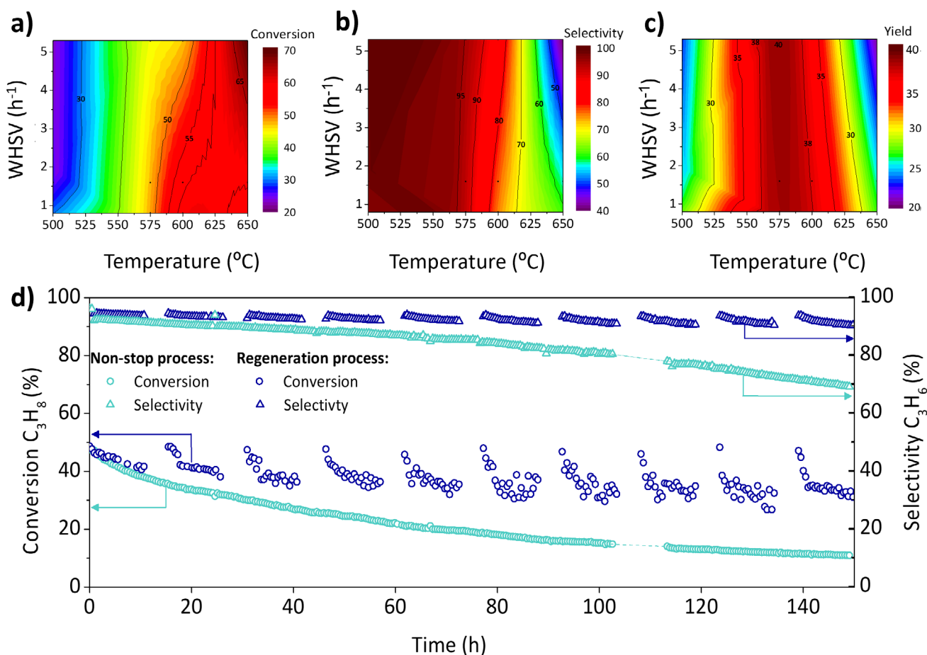
Figure 4. a) Conversion, b) Selectivity, and c) Yield as a function of temperature and WHSV (h -1 ) at initial reaction time (0.9 h) for 0.5%Pt-3%Sn-2%Eu \gamma -Al 2 O 3 catalyst; d) Long-term PDH reaction for 150 h using a 0.5%Pt-3%Sn-2%Eu \gamma -Al 2 O 3 catalyst at 575 °C, WHSV = 1.6 h -1 , and a C 3 H 8 :N 2 ratio of 12:3 mL·min -1 , shown in light blue, versus regeneration cycles, dark blue. Each cycle includes 10.6 h of reaction (under the same conditions), 4 h of regeneration with air at 50 mL min -1 , and 2 h of reactivation with H 2 : Ar at a 1:1 ratio.
