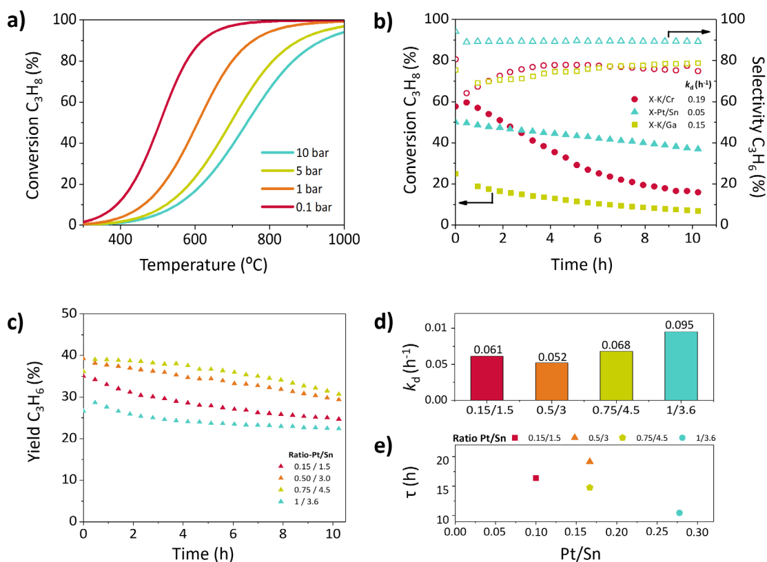
Figure 1. a) Pressure and temperature dependence of C_3H_8 equilibrium conversion in the PDH reaction (side reactions not considered); b) C_3H_8 conversion (filled symbols, left) and C_3H_6 coke-free selectivity (empty symbols, right) during PDH at 575 °C, WHSV = 1.6 h -1 , and C_3H_8:N_2 = 12:3 mL·min -1 and deactivation coefficients c) C_3H_6 yield at same operating conditions as (b); d) Deactivation coefficient and e) Catalyst life, all plotted against the Pt/Sn ratio from synthesis feed (% wt). For reference, the actual Pt/Sn ratios measured by ICP-OES are provided in Table S1.
