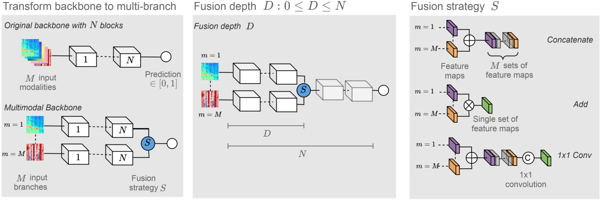
Fig. 2. Architectural hyperparameters optimized by AutoMergeNet. Compared to previous work, our NAS data fusion approach extends the application domain to more than two modalities and automatically tunes the merge depth. (Left) The backbone architecture consists of N blocks and is transformed into multimodal image networks by creating identical but independent branches for each modality. (Center) The fusion depth D determines at which stage in the network a fusion strategy S fuses the branches into a single branch. The branches are fused right before the output layer if the fusion depth equals the number of modules in the network. (Right) The fusion strategy determines how the input branches are fused: concatenating the feature maps of all branches (concatenation); summing the feature maps (addition), or concatenating the feature maps and dividing the number of maps by the number of modalities M using a 1 \times 1 convolution to restore the original number of feature maps (convolution).
