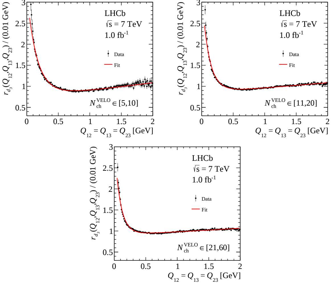
Figure 1: Results of the fit to the three-particle double ratio ( r_{d_3} ) for same-sign pion triplets, are presented in three bins of the VELO track multiplicity: (top left) [5,10] , (top right) [11,20] , (bottom) [21,60] . The red line illustrates the fit performed using the parameterisation outlined in Eq. 13, selecting the triplets of same-sign pions with Q values within the same bin.
