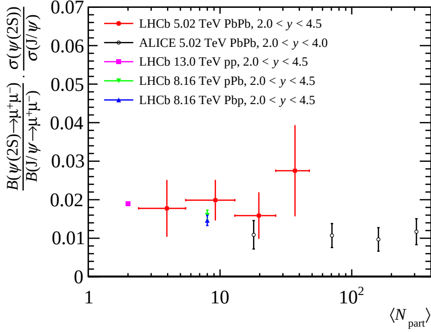
Figure 2: Cross-section times branching fraction ratio between \psi(2S) and J/\psi states as a function of the number of participating nucleons \langle N_{\text{part}} \rangle in the p_T > 0.3 GeV/ c region compared with ALICE PbPb [44] and LHCb pp [45] and p\text{Pb} [46] results. The vertical error bars represent the sum in quadrature of the statistical and systematic uncertainties.
