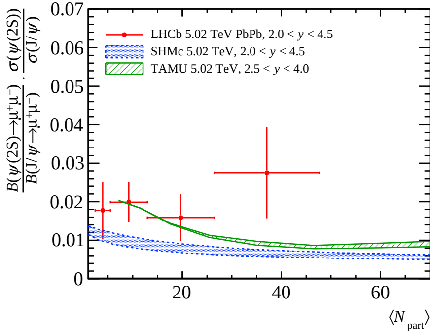
Figure 3: Cross-section times branching fraction ratio between \psi(2S) and J/\psi states as a function of the number of participating nucleons \langle N_{\text{part}} \rangle in the p_T > 0.3 GeV/ c region compared with the SHMc [47, 48] and TAMU model [49, 50] predictions shown by the coloured bands representing the uncertainties. The vertical error bars represent the sum in quadrature of the statistical and systematic uncertainties.
