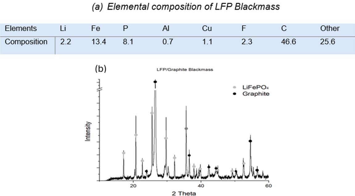
Fig. 1. (a) Elemental Composition of Industrially shredded Blackmass (b) XRD Pattern of LFP Blackmass, comprising of LFP and graphite.
