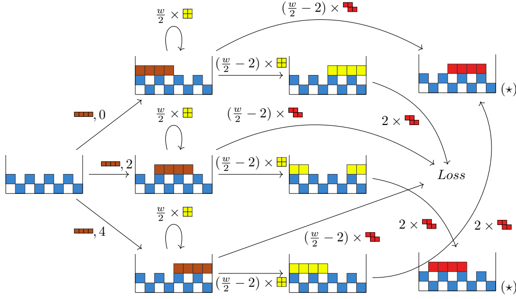
■ Figure 3 Game graph for bifurcation sequence presented in Lemma 8 with board width w = 8 . The board configurations marked with (*) are only reachable for offline players.
