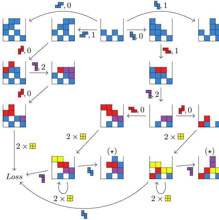
■ Figure 4 Game graph for bifurcation sequence described in Lemma 9 for boards with w = 4 , even h , and h \geq 4 . The board configurations marked with (\star) are only reachable for offline players.
