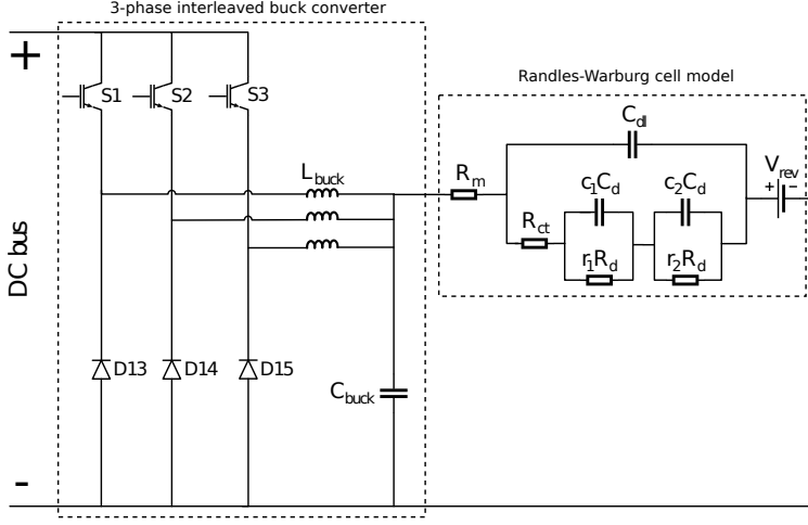
Figure 6.11: Electrolyzer with three-phase interleaved buck converter [Zha+22a; AE20]. Figure reproduced from [MZB24] under the CC BY 4.0 license.
