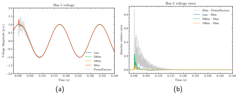
Figure 3.8: (a) Voltage magnitude of Bus5 with different simulation time step, (b) Evolution of absolute relative error during simulation, compared with SFA at 50us time step. Figure reproduced from [ZMB24] under the CC BY 4.0 license.
