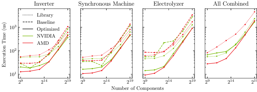
Figure 6.12: Execution time for performing numerical integration with different component models and component counts, with simulating each type of component along or with all types combined. Figure reproduced from [MZB24] under the CC BY 4.0 license.
