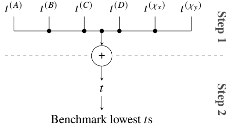
Figure 6.8: Visualization of the optimization flow. The first phase benchmarks each part isolated. The second part then combines the results to predict runtimes for combinations and benchmarks the ones with the lowest predicted runtimes. Figure reproduced from [MZB24] under the CC BY 4.0 license.
