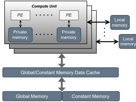
Figure 2.5: Hardware abstraction of heterogeneous computing frameworks like OpenCL, CUDA or HIP. Illustration using terminology of OpenCL. Figure reproduced based on [MZB24] under the CC BY 4.0 license.
