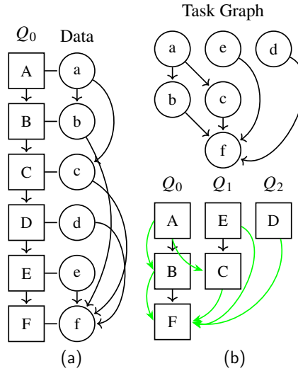
Figure 3.3: An example execution task graph during one time step. Q_i represents command queue or stream. Squares represent the task and round circles represent the associated data, (a) shows an in-order execution of tasks, data dependency is illustrated to the right but usually has no effect to the execution. (b) shows the task graph based on the data dependency, and the concurrent execution of the original tasks based on the task graph. Green edges indicate the synchronization among tasks. Figure reproduced from [ZMB24] under the CC BY 4.0 license .
