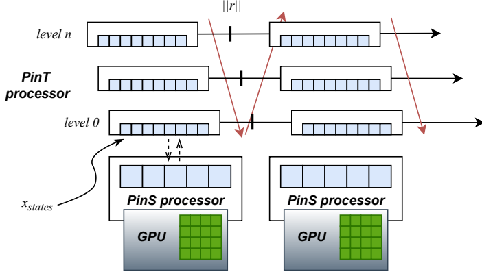
Figure 4.7: PinTS Implementation
