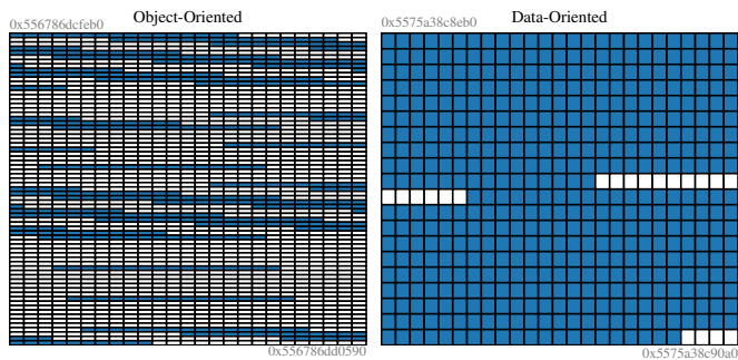
Figure 5.2: Comparison of memory layout in data-oriented and object-oriented design, each cell represents a memory address. Addresses with data allocated are marked.
