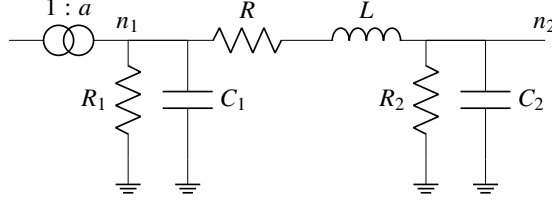
Figure 2.4: Pi-Model to represent transmission line with lumped parameters or transformers, the grounding branches can be removed depending on the need.
