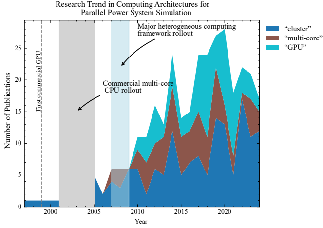
Figure 1.2: Relative research interest in power system simulation with different parallel hardware.
