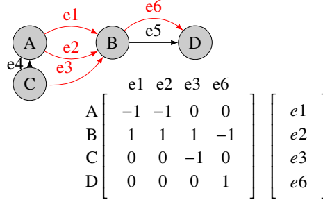
Figure 3.2: Simple connected directed graph and its incidence matrix. The dynamic edges are marked with red. Figure reproduced from [ZMB24] under the CC BY 4.0 license .
