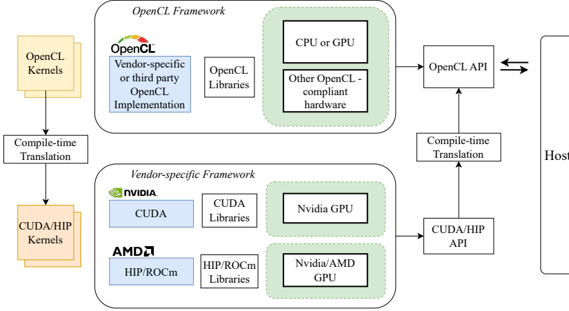
Figure 3.4: Implementation of the fully parallel program. Figure reproduced from [ZMB24] under the CC BY 4.0 license.
