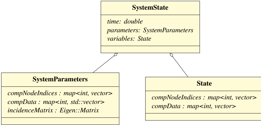
Figure 5.5: Class diagram of SystemState
