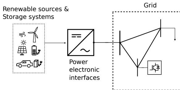
Figure 3.12: All the generators are replaced by inverter-based resources, the three-phase inverter model is taken from [Vyg+21].
