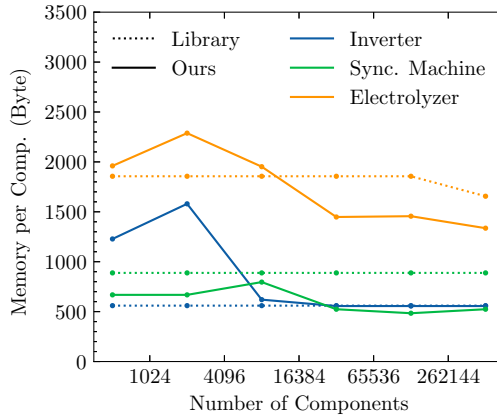
Figure 6.14: Memory consumption per component on the NVIDIA A100 GPU of different component models, for our and the library implementation. The lower limit is calculated by considering the minimum number of parameters required for each component. Figure reproduced from [MZB24] under the CC BY 4.0 license.
