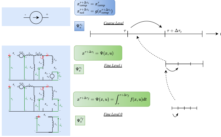
Figure 4.2: Illustration of hybrid models, different models are applied at different PinT level.
