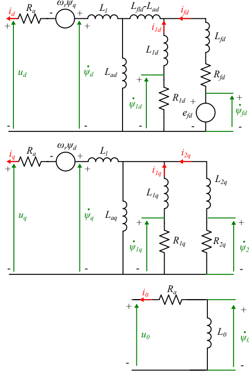
Figure 2.3: Equivalent circuit on dq0 -axis of synchronous machine. Figure reproduced from [MZB24] under the CC BY 4.0 license.
