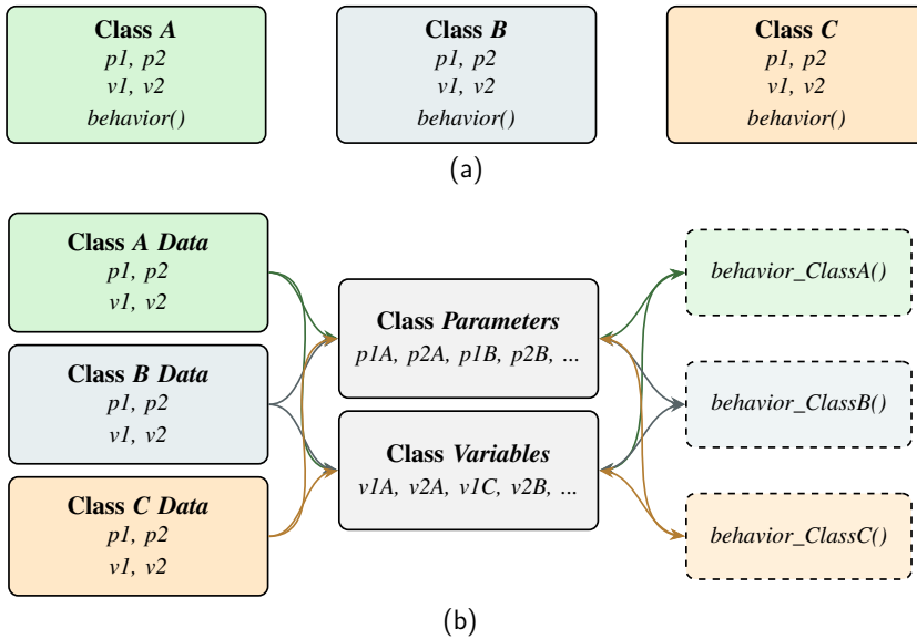
Figure 5.1: Example of (a) object-oriented design: objects has its data and own behavior internally implemented, explicit interaction among objects is not needed; (b) data-oriented design: data and behavior of the objects are implemented separately.
