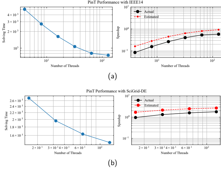
Figure 4.6: Estimated parallel speedup using the performance model compared with actual measurement
