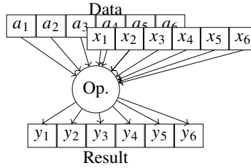
Figure 3.5: Illustration of SIMD execution on single CPU core.
