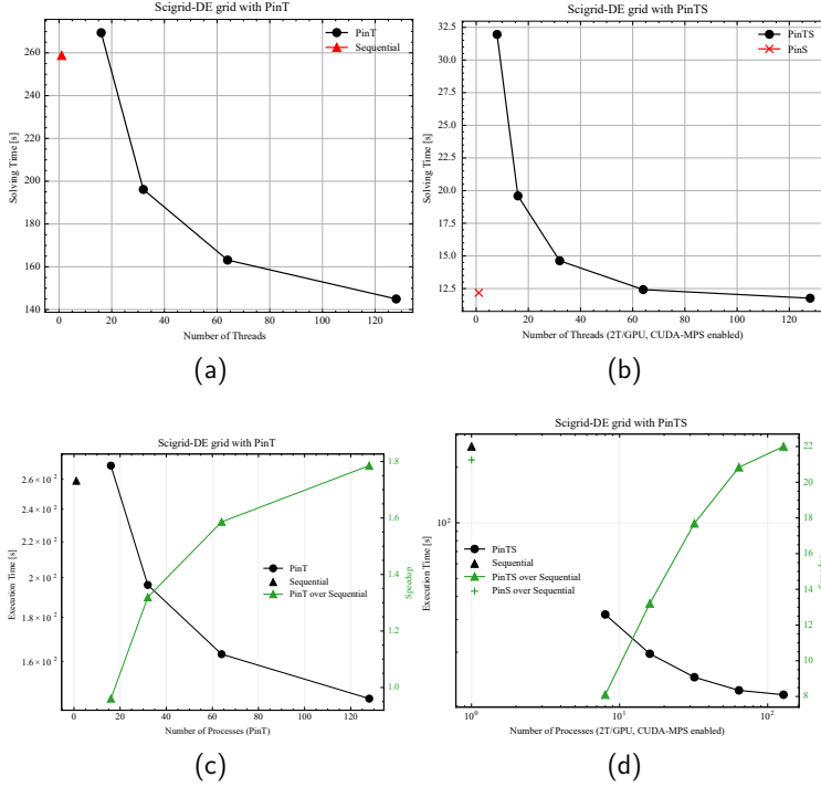
Figure 4.8: Benchmark result on dynamic SciGrid-DE system. (a)(c) Solving time and speedup with PinT , (b)(d) Solving time and speedup with PinTS
