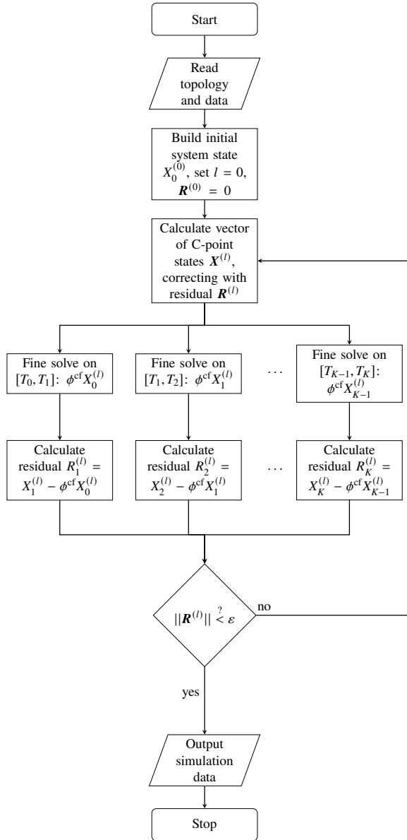
Figure 4.1: Execution flow-chart of the implemented PinT algorithm in two-levels. Figure reproduced based on [SDB22] under the CC BY 4.0 license .
