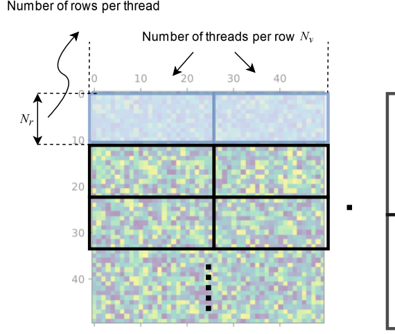
Figure 6.7: Illustration of two of the vectorization parameters N_v and N_r on the matrix-vector multiplication (mv). When more than one thread work on the same row, a parallel binary reduction is used to collect the sum for each row. Figure reproduced from [MZB24] under the CC BY 4.0 license .
