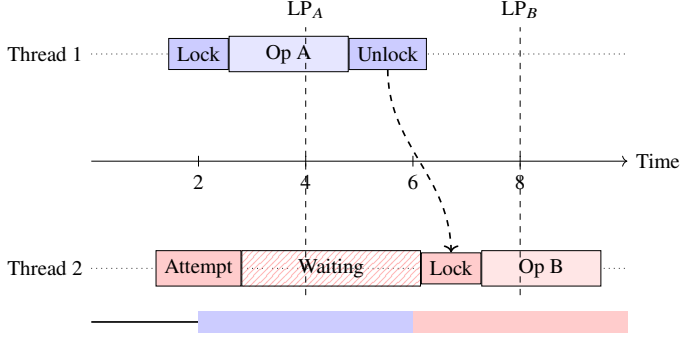
Figure 6.2: Traditional lock-based approach for resource contention. Synchronization timeline with critical sections (colored regions) and linearization points. The dashed arrow shows lock handoff.
