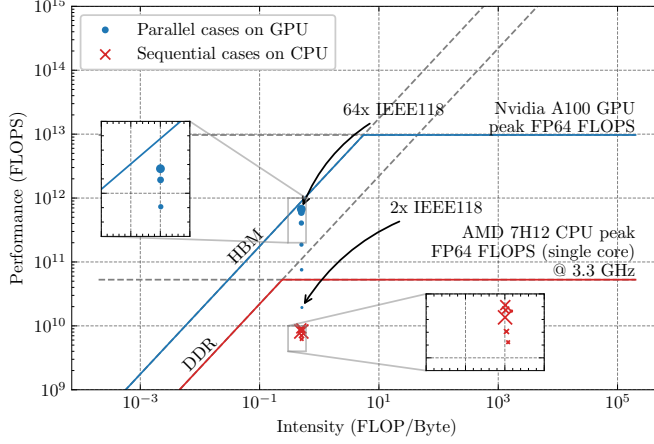
Figure 6.1: Roofline model of the parallel and sequential cases, larger marker represent larger network sizes. Figure reproduced from [ZMB24] under the CC BY 4.0 license .
