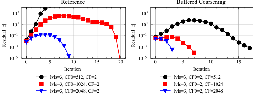
Figure 4.4: Convergence performance using buffered coarsening, where the coarse grid first uses a small coarsening factor, and then applying more aggressive coarsening
