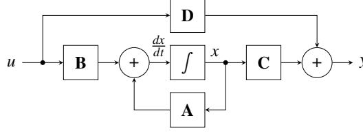
Figure 6.6: Block diagram of the model described by Eq. (6.24) and Eq. (6.25) when setting the nonlinearities \chi_{\dot{x}} = \chi_y = 0 . Figure reproduced from [MZB24] under the CC BY 4.0 license.
