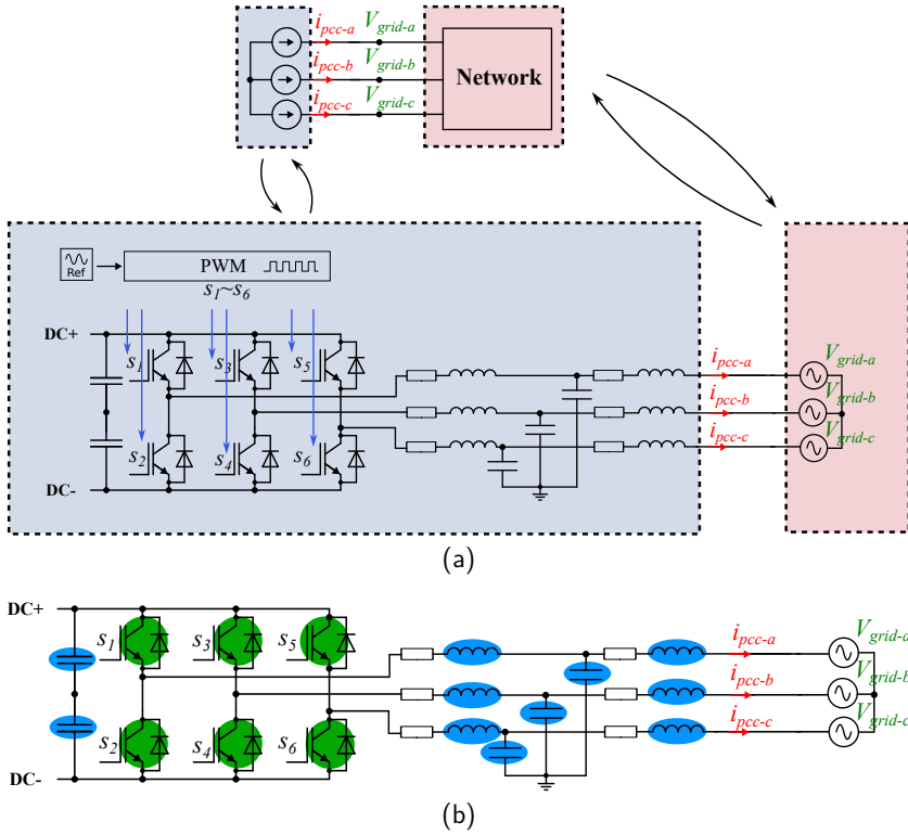
Figure 3.11: (a) The inverter subsystem as a component and its representation in the network (b) Decoupling of component computations within the inverter subsystem
