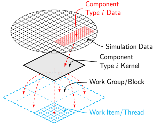
Figure 3.1: SIMT -based compute kernel design for different components. Figure reproduced from [ZMB24] under the CC BY 4.0 license .
