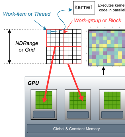
Figure 2.6: Illustration of the parallel execution model [KH13], based on terminology from OpenCL and CUDA/HIP. Figure reproduced from [MZB24] under the CC BY 4.0 license.
