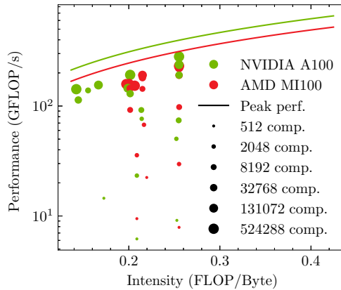
Figure 6.13: Performance of the optimized kernels in a roofline plot to relate kernel performance to peak performance. The size of the dots relates to the number of components. Figure reproduced from [MZB24] under the CC BY 4.0 license.
