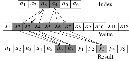
Figure 5.4: Illustration of the gather-scatter approach for parallel execution on device.
