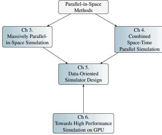
Figure 1.3: Dissertation Outline
