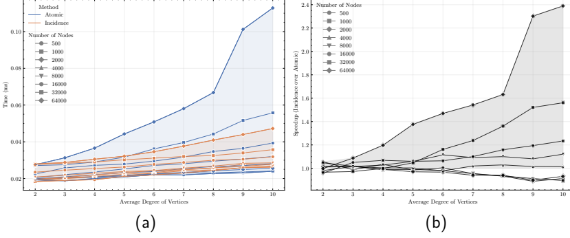
Figure 6.4: Comparison of execution time for using atomic operation and incidence matrix with respect to different network size and different degrees
