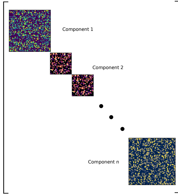
Figure 6.9: Illustration of the library implementation to represent computations in generic solvers, e. g. in [Bal+21]. Figure reproduced from [MZB24] under the CC BY 4.0 license.
