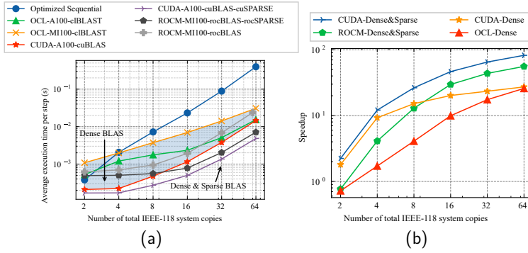
Figure 3.10: (a) Average execution time per simulation step, (b) Speedup of parallel simulation on GPU over optimized sequential simulation on CPU. Figure reproduced from [ZMB24] under the CC BY 4.0 license.
