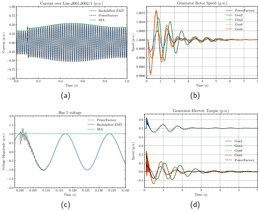
Figure 3.7: System responses after opening Line_0001_0005, (a) Current over Line_0001_0002/1, (b) Generator rotor speed, (c) Voltage at Bus 5, (d) Generator electric torque. Figure reproduced from [ZMB24] under the CC BY 4.0 license.
