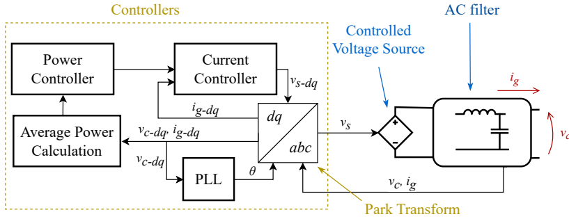
Figure 6.10: Distributed generation inverter model [PPG07; Zha+22b] . Figure reproduced from [MZB24] under the CC BY 4.0 license .
