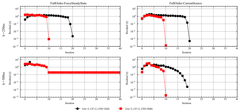
Figure 4.3: Comparison of different hybrid model approaches on the coarse level to improve convergence.
