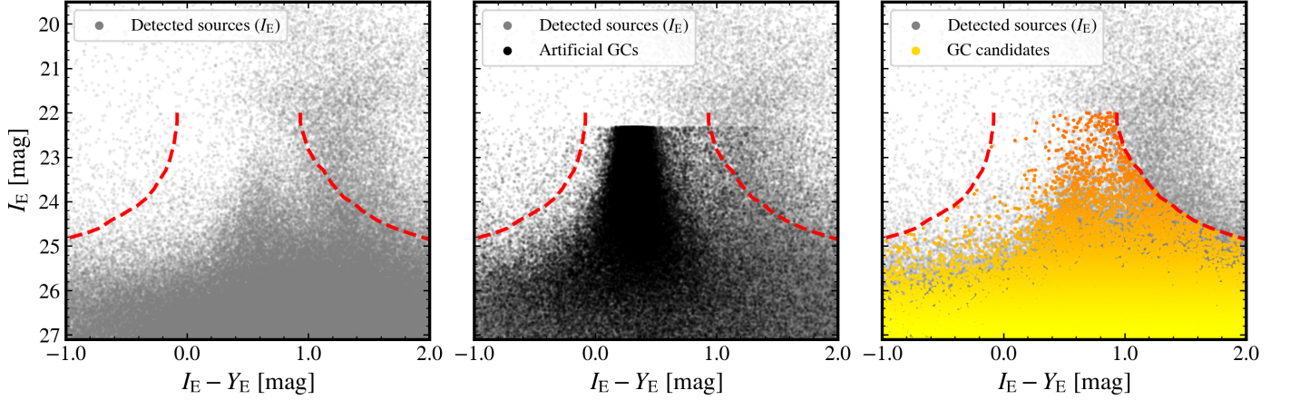
Fig. 4. Photometric criteria applied for GC identification, aiming for high completeness. The three rows demonstrate these criteria for compactness index ( C_{2-4} ), ellipticity ( \epsilon ), and I_E - Y_E colour (as an example). In each row, we show the real-sky sources detected in Euclid I_E images (grey points), the detected artificial GCs (black points), and the real-sky sources selected as GC candidates (yellow points). The dashed red curves represent the selection boundaries adopted based on the distribution of artificial GCs in each parameter space. In the top row, we see that the artificial GCs follow the vertical sequence of point sources (with an average C_{2-4} = 0.7 ), and the scatter becomes larger with fainter magnitude due to an increase in photometric uncertainties. In the bottom row, we see that the selection boundaries reject the majority of objects with I_E < 24 and I_E - Y_E > 1 , which are foreground stars. However, a fraction of those stars end up in the final catalogue. This contamination is unavoidable considering the expected colour range of GCs. Tightening the selection criteria removes these contaminant stars, but leads to lower completeness.
