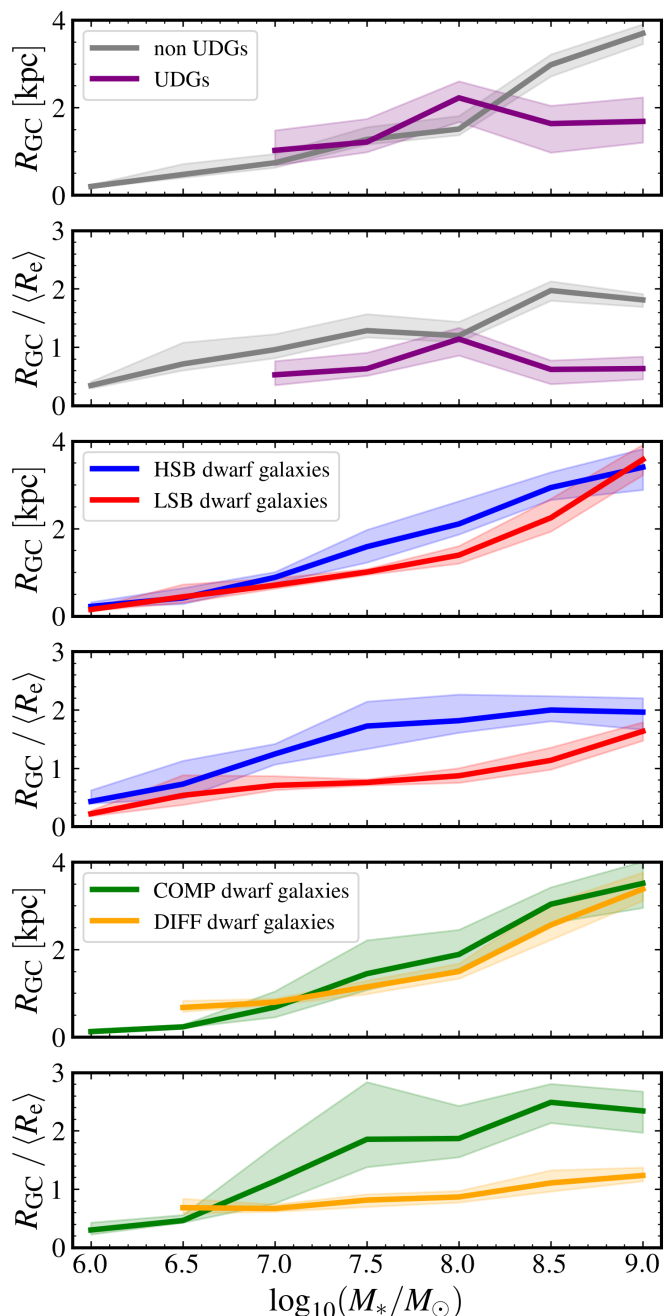
Fig. 8. Similar to Fig. 7 for different dwarf galaxy categories. The two top panels represent the estimations for UDGs and non-UDGs (in purple and grey), the two middle panels for LSB and HSB dwarf galaxies (in red and blue), and the bottom two panels for DIFF and COMP dwarf galaxies (in yellow and green).
