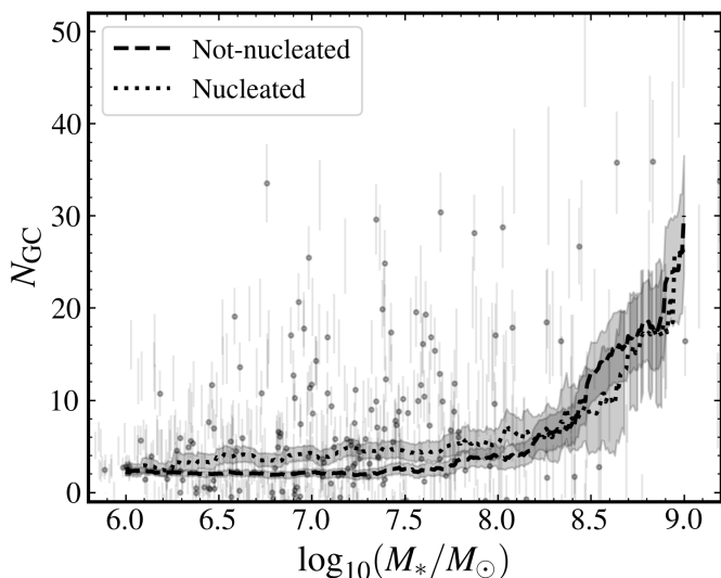
Fig. 12. Similar to Fig. 10 and Fig. 11, for the nucleated and not-nucleated dwarf galaxies in the sample. The vertical lines with and without a central small circle indicate nucleated and not-nucleated dwarf galaxies, respectively.
