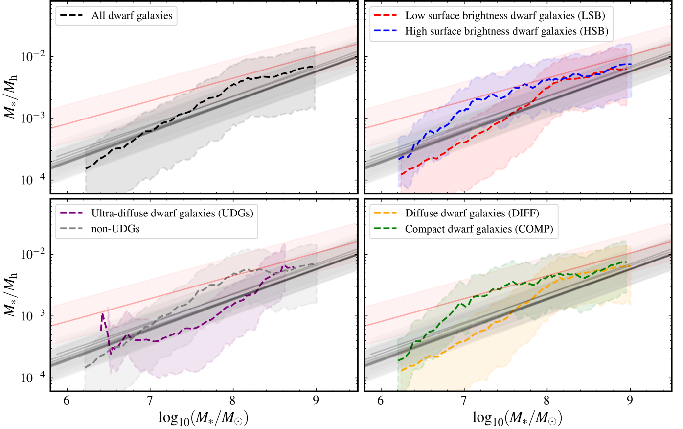
Fig. 15. Stellar-to-halo mass ratios (SHMR, grey and red solid curves) of dwarf galaxies of various categories at z = 0 based on their GC numbers, versus models (various techniques). Grey curves represent a compilation of the SHMRs as presented in Behroozi et al. (2019). The shaded area around these SHMRs correspond to 0.25 dex uncertainty for the SHMR relations. The shown SHMR at these mass regime is an extrapolation of the SHMR obtained for the more massive galaxies. The red solid line and the shaded area around it (in panels on the left) show the SHMR relation for low-mass galaxies (at z = 0 ) in Zaritsky & Behroozi (2023) and its uncertainties (0.31 dex). The shaded area around dashed curves represents the uncertainties in M_h , converted from uncertainties in N_{GC} . These uncertainties are converted from uncertainties in N_{GC} as estimated in Sec. 4.3 (using bootstrapping) and shown in Figures 10 and 11. The shown uncertainties also include to overall uncertainties regarding the N_{GC} - M_h conversion, which is \pm(2 \times 10^9 N_{GC}) .
