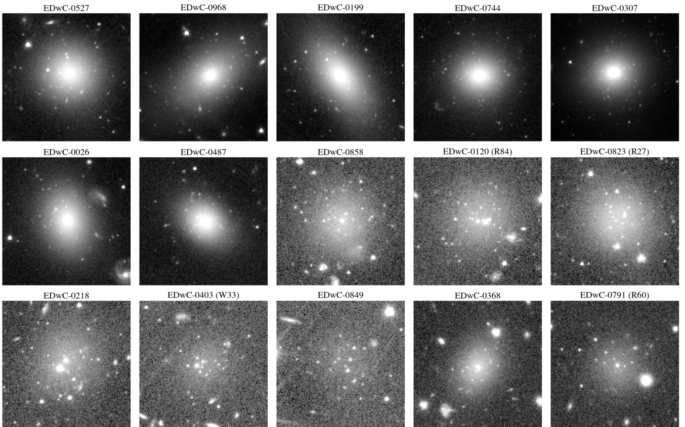
Fig. 13. A few examples of Perseus cluster dwarf galaxies with more than 10 GCs ( N_{GC} > 10 ) in I_E data. The majority of such dwarf galaxies have a stellar mass of M_* > 10^8 M_\odot while they cover a range of central surface brightness ( \mu_0 ) and effective radius ( R_e ). The Euclid ID of dwarf galaxies from Marleau et al. (2025) are written on top of each cutouts, as well as their name in Janssens et al. (2022) when available (written in parenthesis). The cutouts have dimensions of 40'' \times 40'' (about 14 \text{ kpc} \times 14 \text{ kpc} ).
