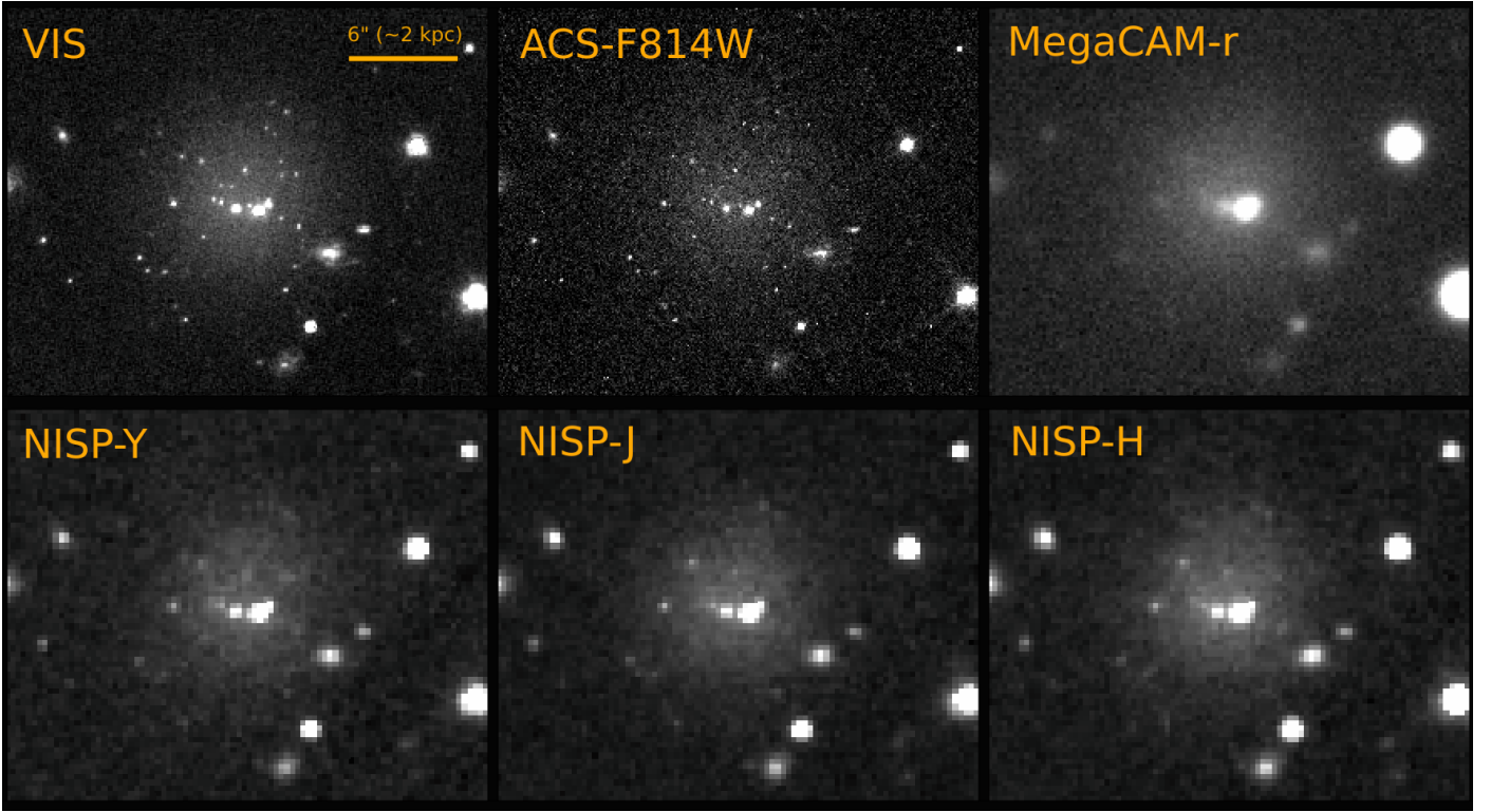
Fig. 1. A view of a Perseus cluster dwarf galaxy (EDwC-0120 in Marleau et al. 2025 , and R84 in Janssens et al. 2024 ) as seen by the VIS and NISP instruments onboard Euclid (in I_E , Y_E , J_E , and H_E ), by HST/ACS (in F814W) and by CFHT/MegaCAM (in r ). The galaxy seems to host several GCs, which appear as point sources on top of the galaxy, as well as a nuclear star cluster (NSC) in the centre of the diffuse component. The brightest object projected near the centre of the galaxy could be a foreground star, or a massive GC destined to merge with the already existing NSC.
