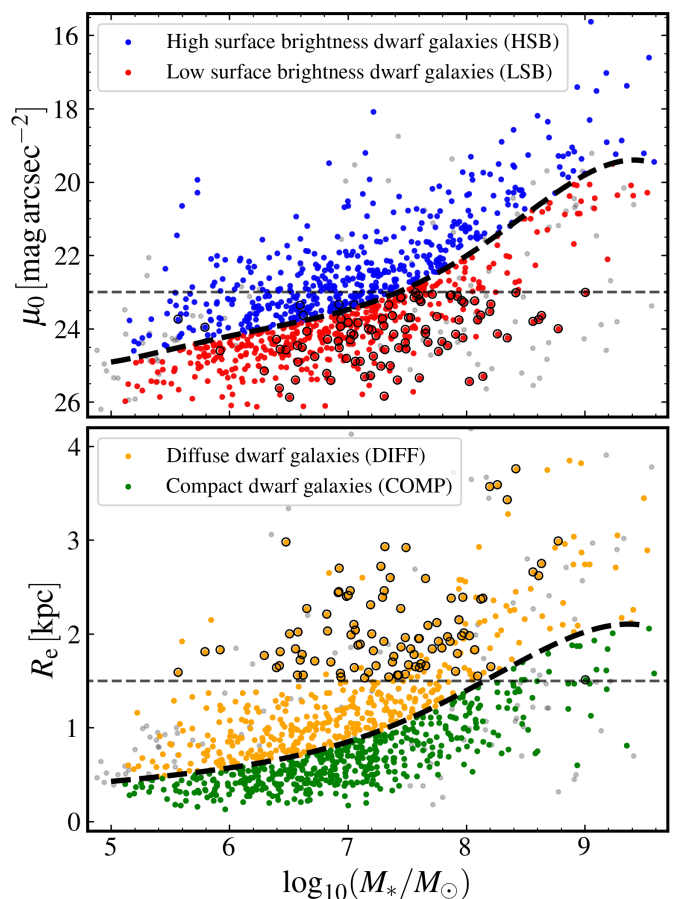
Fig. 6. Division of the dwarf galaxy sample into high surface brightness dwarf galaxies (HSB, blue points), low surface brightness dwarf galaxies (LSB, red points), compact dwarf galaxies (COMP, green points), and diffuse dwarf galaxies (DIFF, yellow points) based on their central surface brightness ( \mu_0 ) and effective radius ( R_e ). A distance of 72 Mpc was assumed to convert angular to physical scale. This division is stellar mass dependent and is indicated with the black dashed curve. Coloured points represent the dwarf galaxies that have been used for the analysis in this paper. Those dwarf galaxies that also satisfy the UDG criteria in \mu_{0,I_E} and R_e ( \mu_{0,I_E} < 23 \text{ mag arcsec}^{-2} and R_e > 1.5 \text{ kpc} , shown with dashed horizontal lines) are indicated with the black circles around the coloured circles. Grey points show those dwarf galaxies that have been removed from the sample after initial assessment (as was mentioned in Sect. 2.2).
