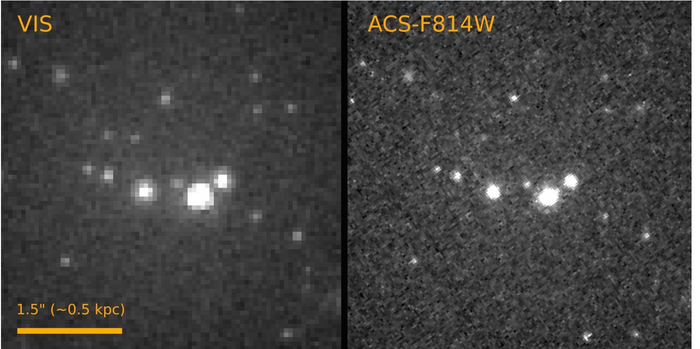
Fig. 2. A zoomed view of the dwarf galaxy in Fig. 1 as seen by Euclid /VIS in I_E and HST/ACS in F814W (PIPER survey, Harris et al. 2020 ). The total integration times for these images are 8960 s and 2100 s respectively. The depths of both data sets are comparable while HST/ACS provides a higher spatial resolution with a better sampled PSF than Euclid /VIS.
