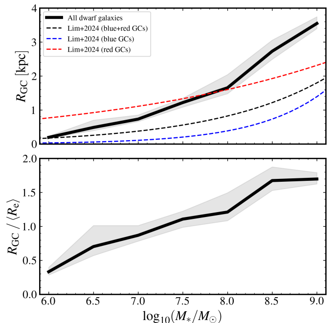
Fig. 7. GC half-number radius ( R_{GC} , top panel), and ratio between the GC half-number radius and the average of the host-galaxies effective radius ( R_{GC}/\langle R_e \rangle , bottom panel), as functions of the stellar mass of the host galaxies ( M_* ) for all dwarf galaxies in the sample. The values are estimated from stacked GC radial profiles that we fit with a Sérsic function, with a Sérsic index fixed to n = 1 (see text). The shaded region around each line represent the 68% percentiles of the estimated average value. The dashed lines show the trends one would expect from a simple extension of the equations in Lim et al. (2024), that were derived for GCs in massive galaxies, to our lower mass regime (an extrapolation beyond the range examined by these authors).
