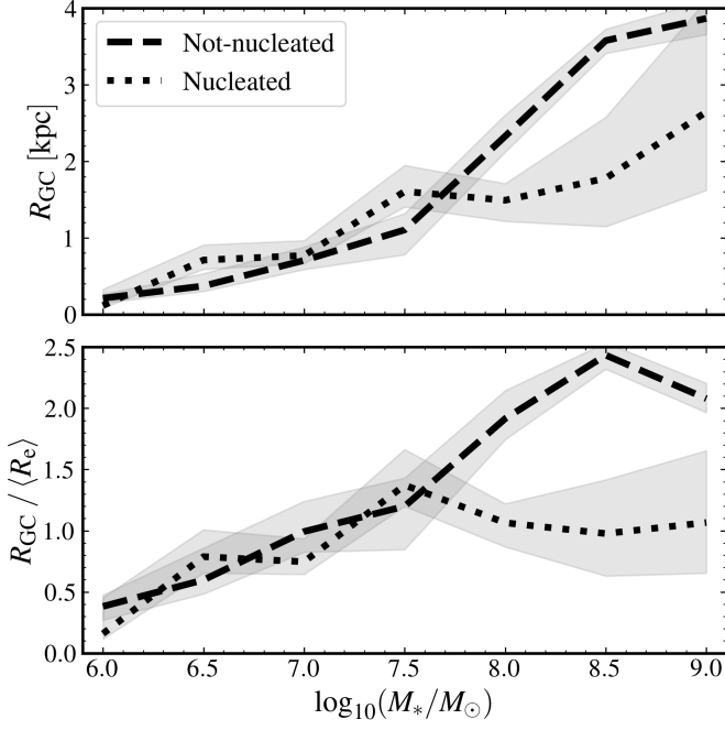
Fig. 9. Same as Fig. 7 and Fig. 8, but for nucleated and non-nucleated dwarf galaxies in our sample.
