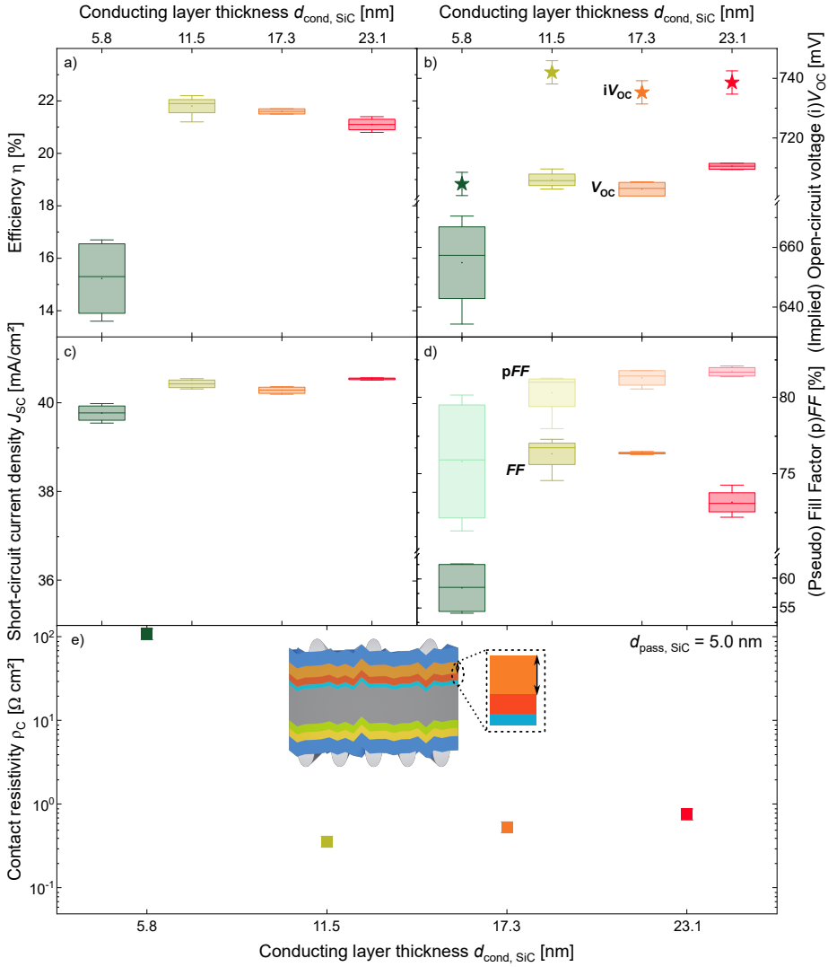
Figure 4.9.: Effect of varying the conducting nc\text{-SiC:H}(n) layer thickness ( d_{\text{cond, SiC}} ) on a) power conversion efficiency ( \eta ), b) implied open-circuit voltage ( iV_{\text{oc}} ) and open-circuit voltage ( V_{\text{oc}} ), c) short-circuit current density ( J_{\text{sc}} ), d) pseudo Fill Factor (pFF) and Fill Factor (FF), and e) contact resistivity ( \rho_c ). Extremely thin d_{\text{cond, SiC}} detrimentally affects most solar cell parameters. Thicker layers primarily reduce FF. The inset illustrates the sample with the varied layer within the stack.
