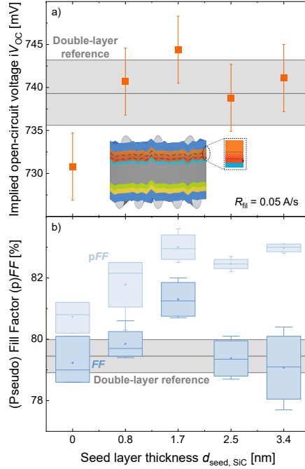
Figure 4.16.: The a) implied open-circuit voltage ( iV_{OC} ) and b) pseudo Fill Factor (pFF) and Fill Factor (FF) for varying passivating seed nc-SiC:H(n) layer thickness ( d_{seed, SiC} ). The filament current ramp ( R_{fil} ) of the seed layer is constant at 0.05 \frac{A}{s} . An increase in iV_{OC} with a growing pseudo Fill Factor (pFF)-FF gap is observed for increasing d_{seed, SiC} .
