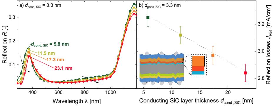
Figure 4.10.: a) Reflection ( R ) curves for varying conducting \text{nc-SiC:H(n)} layer thicknesses ( d_{\text{cond, SiC}} ) and b) the resulting calculated reflection losses ( J_{\text{Ref}} ) from a). A thicker d_{\text{cond, SiC}} leads to a reduced reflection in the layer stack. The inset depicts the sample structure with the varied layer. Permission for use granted by John Wiley & Sons - Books, from [113] via Copyright Clearance Center, Inc.
