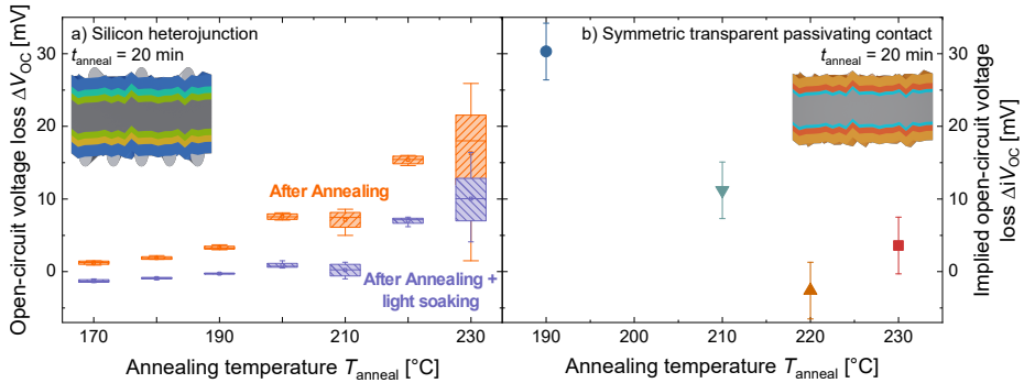
Figure 5.19.: Analysis of a) open-circuit voltage loss ( \Delta V_{oc} ) for a silicon heterojunction (SHJ) solar cell and b) \Delta iV_{oc} a symmetrically passivated wafer with the transparent passivating contact (TPC) structure for varying annealing temperature ( T_{anneal} ). The constant annealing time ( t_{anneal} ) is 20 minutes for both cases. While the SHJ solar cell exhibits degradation at temperatures above 190 °C, or 210 °C with light soaking, the symmetric TPC structure recovers at T_{anneal} of 220 °C or higher. Insets depict the sample structures of a SHJ solar cell and a symmetric TPC sample.
