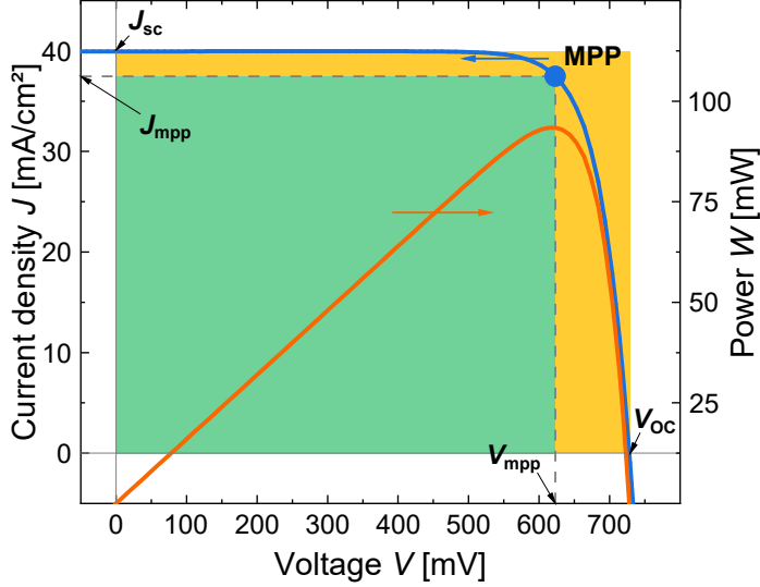
Figure 2.5.: Illustration of a JV-curve (blue) and the corresponding power (orange) of a solar cell under one sun illumination. Key solar cell parameters are highlighted. The curve is mirrored to positive currents for clarity.
