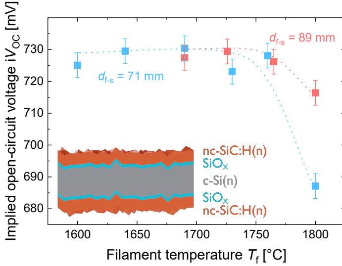
Figure 4.5.: Variation in the implied open-circuit voltage ( iV_{OC} ) as a function of the filament temperature ( T_f ) for two distinct filament-substrate distances ( d_{f-s} ). The inset shows the sample structure featuring SiO_x and nc-SiC_x:H(n) layers on both sides. The lower T_f leads to an enhanced iV_{OC} , while a larger d_{f-s} shifts the temperature of iV_{OC} decline to higher values. The dashed lines serve as visual guides.
