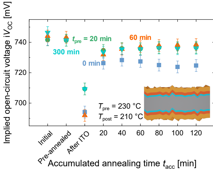
Figure 5.21.: Implied open-circuit voltages ( iV_{OC} s) of symmetrically transparent passivating contact (TPC)-passivated samples at different process stages and accumulated annealing times ( t_{acc} s). Samples have varying t_{pre} before the sputter deposition. The pre-annealing temperature ( T_{pre} ) is 230 °C, and the post-annealing temperature ( T_{post} ) is 210 °C. The inset depicts the sample structure.
