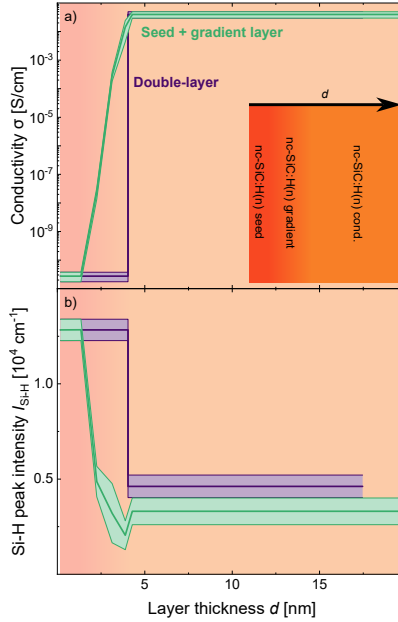
Figure 4.18.: Updated schematic cross-section of the a) electrical conductivity ( \sigma ) and b) FTIR silicon-hydrogen bond peak intensity ( I_{\text{Si-H}} ) from figure 4.13. The profiles of the approach with the seed and gradient layer are added. An early and strong increase in \sigma is visible, while the I_{\text{Si-H}} has an inverse profile. The inset shows the nc-SiC x H(n) stack with the layer thickness d . The color gradient symbolizes the shift from passivating to conducting nc-SiC x H(n).
