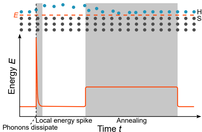
Figure 5.16.: Schematic representation of hydrogen displacement at the silicon interface due to simultaneous multi-phonon dispersion. Subsequent low-temperature annealing can restore broken silicon-hydrogen bonds. Reprinted under CC BY 4.0 from Ref. [226].
