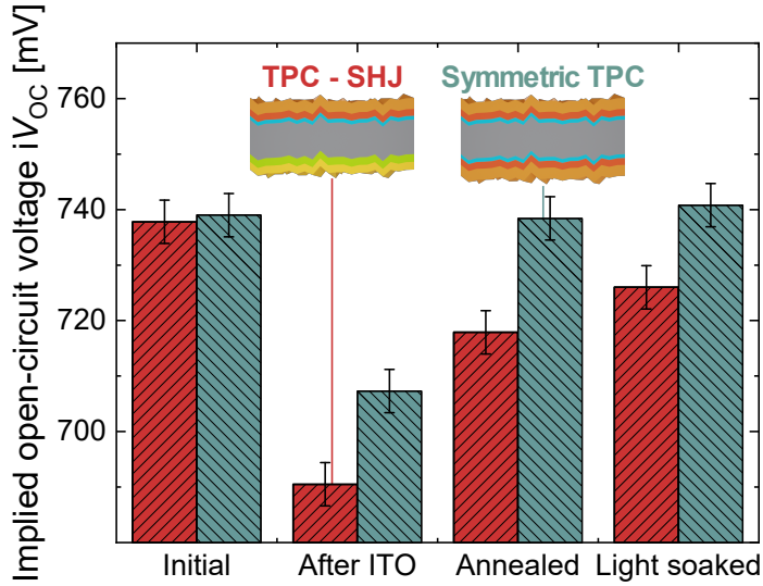
Figure 5.18.: Comparison of implied open-circuit voltage ( iV_{oc} ) for symmetrically passivated wafers with the transparent passivating contact (TPC) and solar cell precursors with a TPC front side and silicon heterojunction (SHJ) rear side at different stages of the process. Although symmetrically passivated samples fully recover after annealing, the solar cell precursors do not, indicating limitations originating from the SHJ side.
