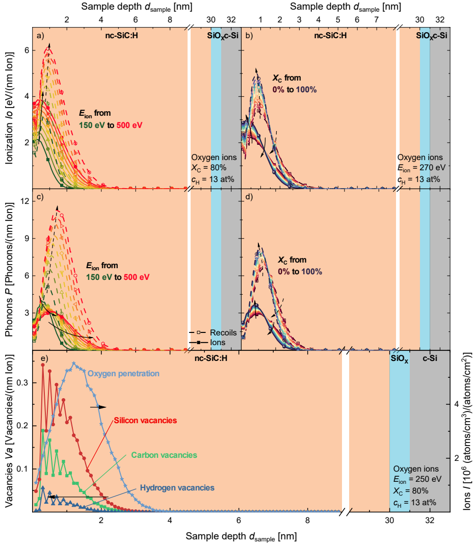
Figure 5.13.: Simulated generation profiles for a) and b) ionization ( I_o ), c) and d) phonon ( P ), and e) vacancy ( V_a ), distinguishing between primary ions (solid lines) and recoiling atoms (dashed lines). a) and c) show the respective profile for a variation of E_{ion} , while b) and d) show the profiles for different X_C .
