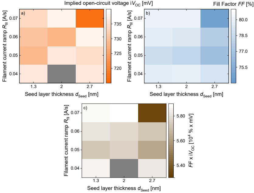
Figure 4.17.: Heatmaps for varying filament current ramps ( R_{fil} s) and passivating seed nc -SiC:H( n ) layer thicknesss ( d_{seed} , SiCs ) for the a) implied open-circuit voltage ( iV_{OC} ) and b) Fill Factor ( FF ). c) shows the same heatmap for the product of iV_{OC} and FF to more easily identify optimal combinations. The iV_{OC} favors a thicker d_{seed} , SiC and lower R_{fil} , while the opposite trend is visible for the FF . The highest combination can be achieved either for low d_{seed} , SiC in combination with low R_{fil} or lower d_{seed} , SiC with high R_{fil} .
