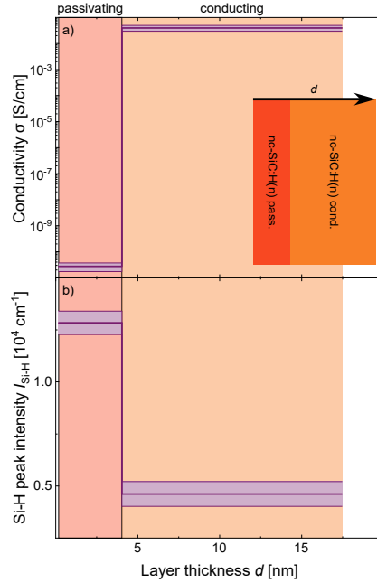
Figure 4.13.: Schematic cross-section of a) the electrical conductivity ( \sigma ) and b) the FTIR silicon-hydrogen bond peak intensity ( I_{\text{Si-H}} ) through the nc-SiC x :H(n) double layer stack. The passivating nc-SiC x :H(n) layer exhibits a high hydrogen concentration and low \sigma , in contrast to the conducting nc-SiC x :H(n), which has a high \sigma and low I_{\text{Si-H}} .
