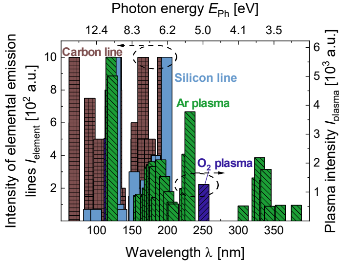
Figure 5.17.: The Intensity of elemental emission lines ( I_{\text{element}} ) for the elements carbon and silicon and the plasma intensity ( I_{\text{plasma}} ) for radiation from an oxygen and argon plasma. Data of the plasma radiation taken from ref. [228] and from ref. [273] for the possible carbon and silicon emission lines.
