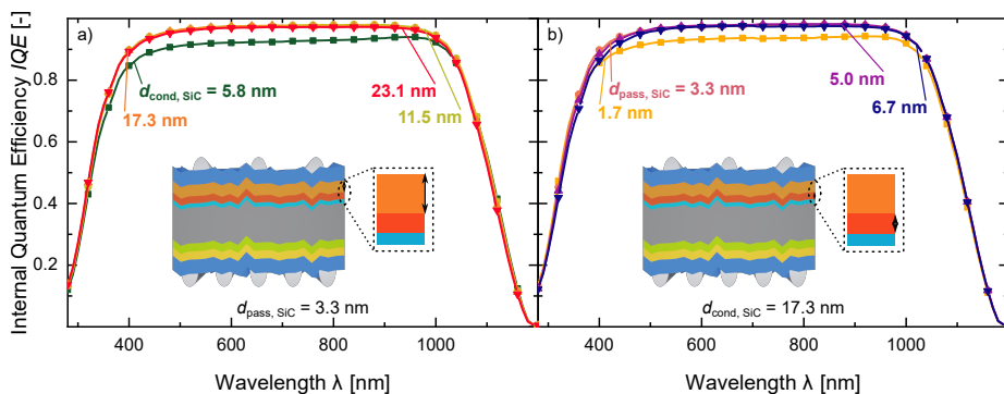
Figure 4.11.: Internal quantum efficiencies (IQEs) for variations in a) conducting nc-SiC:H(n) layer thickness ( d_{\text{cond, SiC}} ) and b) d_{\text{pass, SiC}} . For very thin d_{\text{cond, SiC}} or d_{\text{pass, SiC}} , the IQE is reduced due to poor passivation quality. Insets illustrate the varied layer within the sample stack. Permission for use granted by John Wiley & Sons - Books, from [113] via Copyright Clearance Center, Inc.
