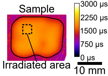
Figure 5.8.: Quasy-Steady State Photoconductance-corrected photoluminescent lifetime (PL) image of a sample part irradiated with an electron beam in a scanning electron microscope. The beam energy is set at 500 eV, with a beam current of 1.6 nA. No degradation in the irradiated area is observed. Figure b) is reprinted under CC BY 4.0 from Ref. [226].
