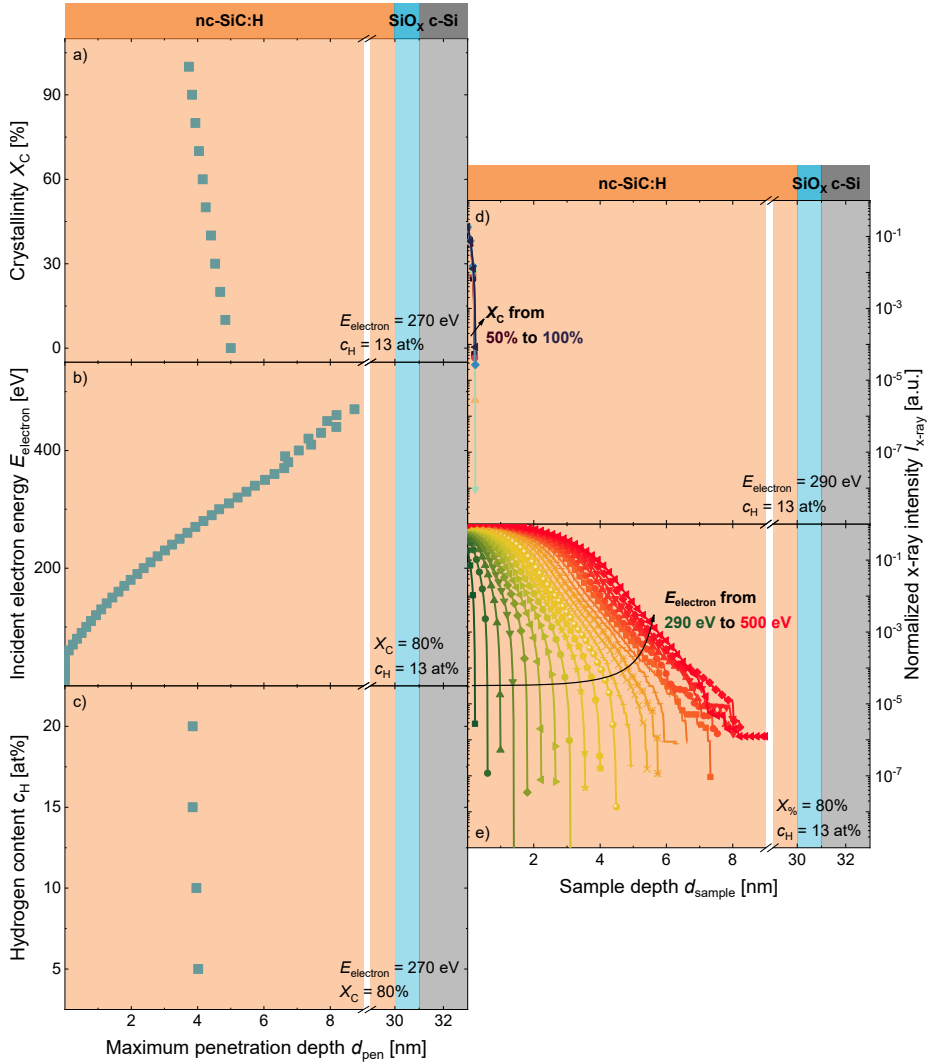
Figure 5.7.: Simulated profiles of variations of a) crystalline volume fraction ( X_C ) of the nc-SiC x :H(n), b) incident electron energy ( E_{\text{electron}} ) of the incident electron, and c) hydrogen content ( c_H ) of the nc-SiC x :H(n) on maximum penetration depth ( d_{\text{max}} ), and x-ray generation profiles depending on d) X_C and e) E_{\text{electron}} \cdot d_{\text{max}} increases for decreasing X_C and increasing E_{\text{electron}} . X-ray generation is superficial but increases for increasing E_{\text{electron}} .
