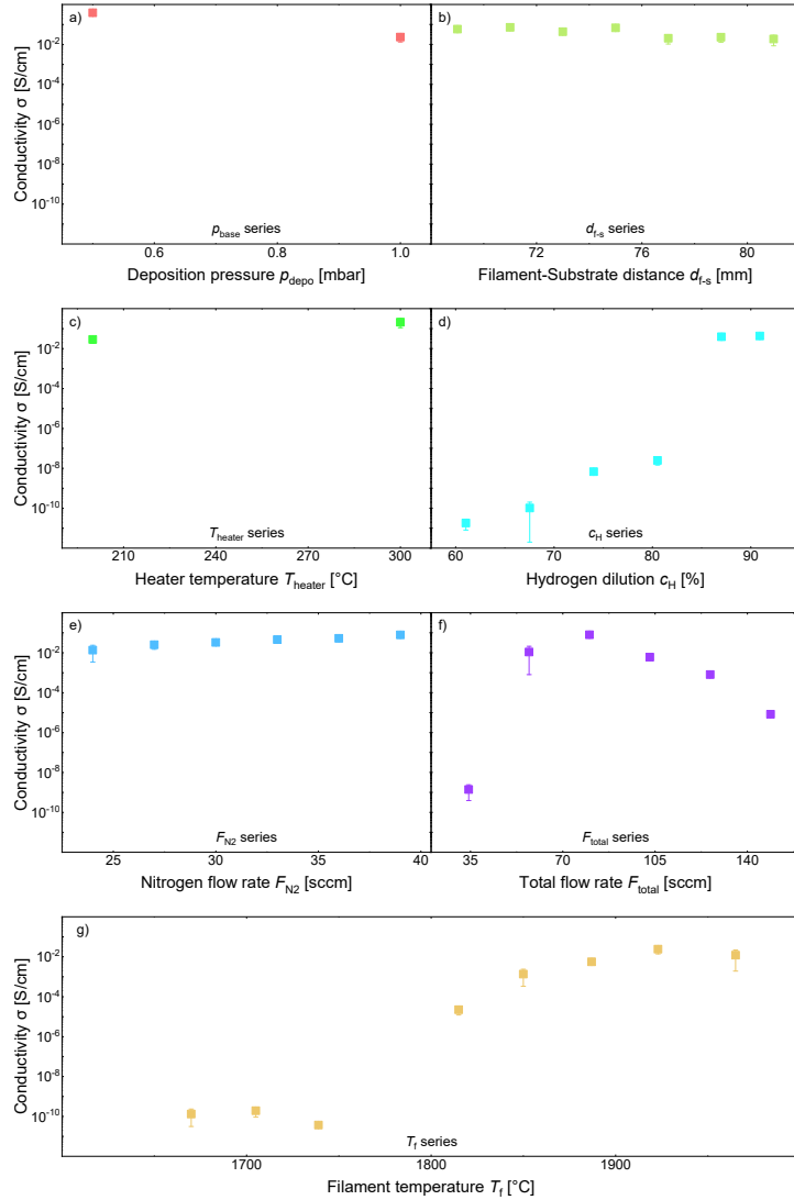
Figure 4.1.: Dependence of the lateral electrical conductivity ( \sigma ) on various deposition parameters a) deposition pressure ( p_{\text{depo}} ), b) filament-substrate distance ( d_{f-s} ), c) chamber heater temperature ( T_{\text{heater}} ), d) hydrogen dilution ( c_H ), e) nitrogen flow rate ( F_{N_2} ), f) total gas flow rate ( F_{\text{total}} ), and g) filament temperature ( T_f ). The parameters that most affect \sigma , with variations of more than nine orders of magnitude, are T_f and c_H , followed by a five orders of magnitude shift in \sigma due to F_{\text{total}} . Reproduced with permission from John Wiley & Sons - Books, from [113]; permission conveyed through Copyright Clearance Center, Inc.
