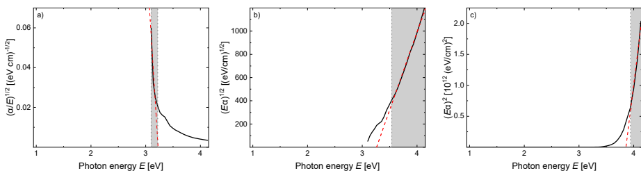
Figure C.4.: Determination of the optical band gap, together with the values of the fit, given by the red dashed line, for the a) Cody, b) Tauc and c) Tauc 2 method. The shaded area visualizes the linear part of the data used for fitting.
