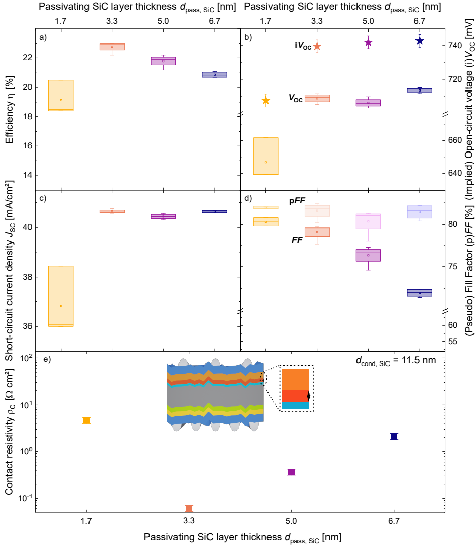
Figure 4.8.: Impact of varying the passivating nc-SiC:H(n) layer thickness ( d_{\text{pass, SiC}} ) on a) power conversion efficiency ( \eta ), b) implied open-circuit voltage ( iV_{\text{OC}} ) and open-circuit voltage ( V_{\text{OC}} ), c) short-circuit current density ( J_{\text{SC}} ), d) pseudo Fill Factor (pFF) and Fill Factor (FF), and e) contact resistivity ( \rho_c ). Extremely thin d_{\text{pass, SiC}} lead to an overall poor cell performance due to passivation challenges. Increased d_{\text{pass, SiC}} enhances passivation but reduces FF. The inset illustrates the sample structure with the varying layer highlighted in the stack.
