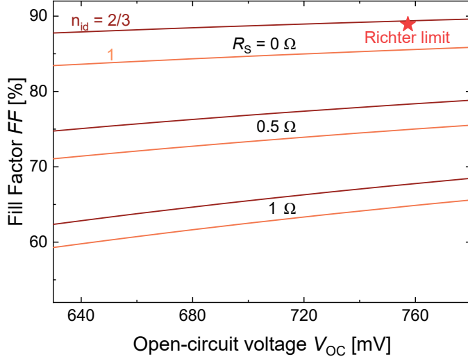
Figure 2.6.: Calculations of the dependence of FF on V_{OC} for n_{id} of 2/3 and 1 and different R_S of 0 \Omega , 0.5 \Omega and 1 \Omega . The star marks the maximum achievable FF- V_{OC} combination for wafer thicknesses and dopant concentrations used in this thesis. The impact of R_{sh} is neglected.
