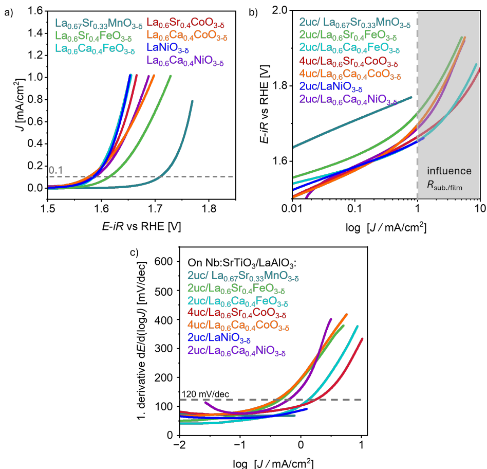
Figure 48: CV up to 1 \text{ mA cm}^{-2} of the Nb:SrTiO 3 /LaAlO 3 /catalyst stacks with only back side contact. b) Corresponding Tafel-like plot shown also in the higher current density range where the R_{\text{sub./LAO/film}} interface starts to dominate the slope of the CV curve, c) First derivative of the plots shown in b), which are the Tafel slope values as a function of the current density.
