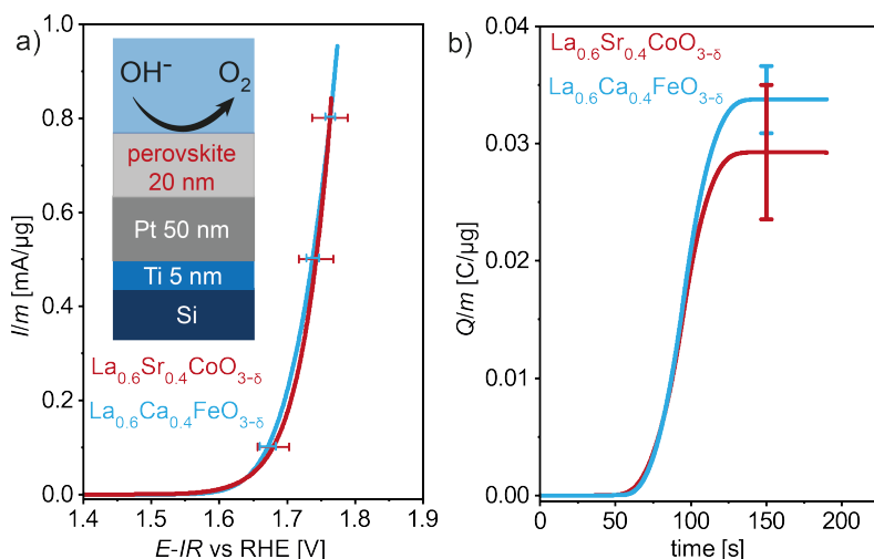
Figure 53: a) OER catalytic mass activity is shown from the averaged CV scan of \text{La}_{0.6}\text{Sr}_{0.4}\text{CoO}_{3-\delta} and \text{La}_{0.6}\text{Ca}_{0.4}\text{FeO}_{3-\delta} thin films deposited on Pt. b) Charge per \mu\text{g} catalyst passed in one CV cycle. Both perovskites generate a comparable charge within one CV scan.
