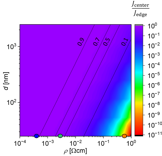
Figure E.2: Heatmap of the (J_{\text{center}})/J_{\text{edge}} ratio on a logarithmic scale to obtain the rapidly increasing inhomogeneity above a resistivity of 2 \times 10^{-2} \Omega \text{ cm} .
