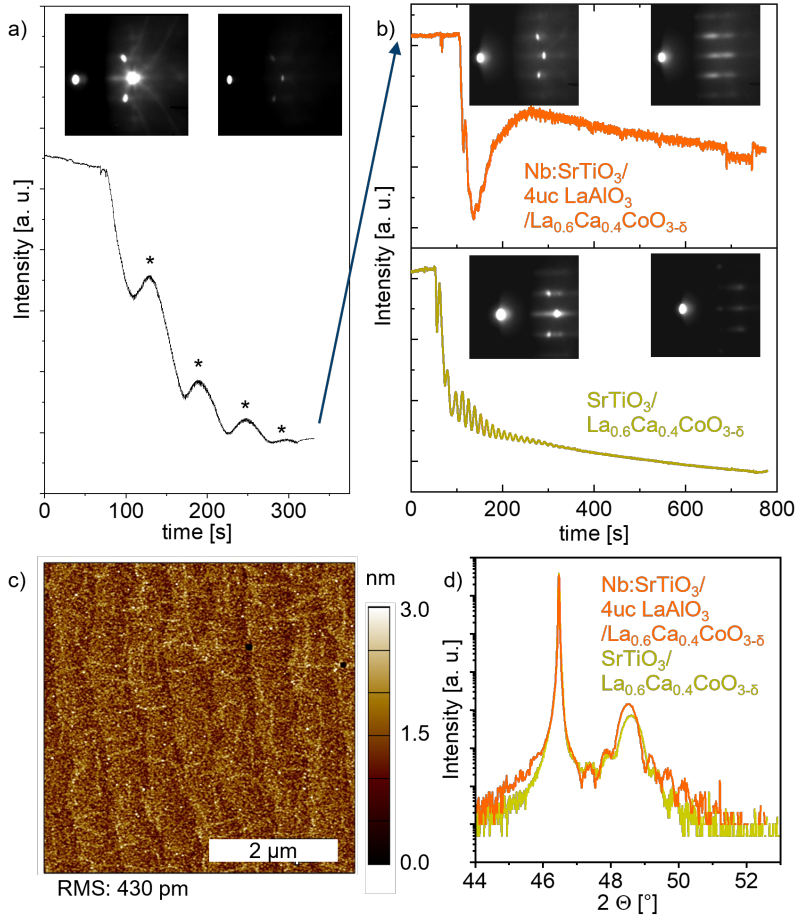
Figure 22: a) Growth of 4 unit cells \text{LaAlO}_3 on \text{Nb:SrTiO}_3 . The * mark the four local RHEED intensity maxima of the \text{LaAlO}_3 growth. b) Top graph: subsequent \text{La}_{0.6}\text{Ca}_{0.4}\text{CoO}_{3-\delta} deposition with the RHEED patterns before and after growth. Bottom graph \text{La}_{0.6}\text{Ca}_{0.4}\text{CoO}_{3-\delta} deposition directly on \text{SrTiO}_3 without \text{LaAlO}_3 layer. c) AFM of the \text{La}_{0.6}\text{Ca}_{0.4}\text{CoO}_{3-\delta} surface where \text{LaAlO}_3 layer is buried. d) XRD comparison of the (002) \text{La}_{0.6}\text{Ca}_{0.4}\text{CoO}_{3-\delta} peak grown on \text{Nb:SrTiO}_3 with a 4 uc thick \text{LaAlO}_3 interlayer, and directly deposited on a \text{SrTiO}_3 substrate.
