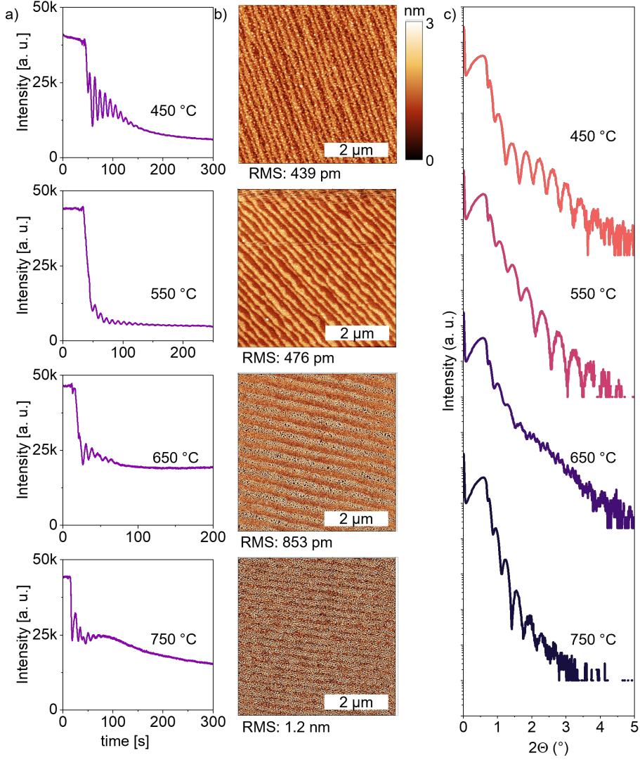
Figure 23: \text{La}_{0.6}\text{Ca}_{0.4}\text{NiO}_{3-\delta} thin films grown on \text{NdGaO}_3 with increasing temperature a) In-situ RHEED tracking of the growth. b) Corresponding AFM scans and c) XRR scans.
