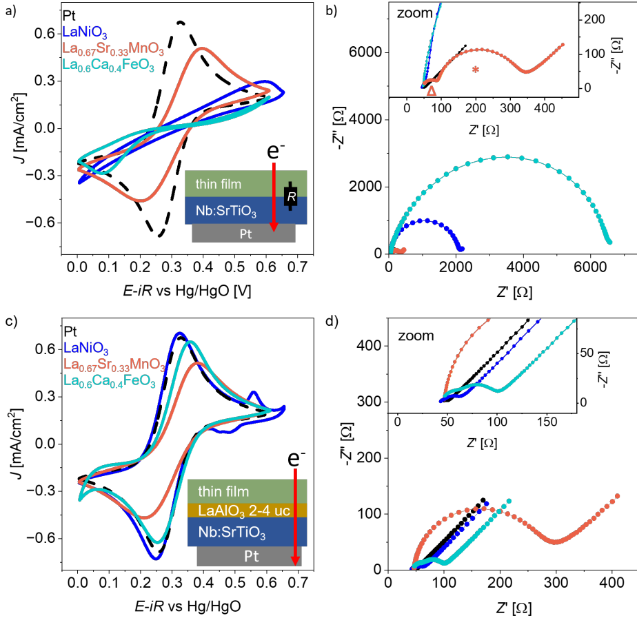
Figure 43: a) CV in hexacyanoferrate(II)/(III) electrolyte for LaNiO 3-δ , La 0.67 Sr 0.33 MnO 3-δ and La 0.6 Ca 0.4 FeO 3-δ thin films grown on Nb:SrTiO 3 in comparison to the Pt sample. The sweep rate was 30 mV/s. For LaNiO 3-δ in this case, the sweep window was extended to 0.65 V vs Hg/HgO to obtain a possible contribution from Ni oxidation. b) Corresponding impedance spectra at the OCP. Legend corresponds to a). Inset shows the zoom of the lower impedance values. Δ refers to the semi-circle in the high frequency range of La 0.67 Sr 0.33 MnO 3-δ and * refers to the semi-circle toward lower frequencies. c) CV in hexacyanoferrate(II)/(III) electrolyte for Nb:SrTiO 3 /2 uc LaAlO 3 / LaNiO 3-δ , Nb:SrTiO 3 /2 uc LaAlO 3 / La 0.67 Sr 0.33 MnO 3-δ and Nb:SrTiO 3 /4 uc LaAlO 3 / La 0.6 Ca 0.4 FeO 3-δ thin films in comparison to the Pt sample. The sweep rate was 30 mV/s. For LaNiO 3-δ , additional oxidation and reduction peaks are seen at 0.55 V and 0.45 V vs Hg/HgO, respectively, representing the Ni 2+ /Ni 3+ redox reaction. d) Corresponding impedance spectra at the OCP. Inset shows the zoom to the lower impedance values. The figure was adapted by the color scheme from our publication [176], with the rights of the license CC-BY 4.0. The LaNiO 3-δ experiments were conducted by Iris van den Bosch.
