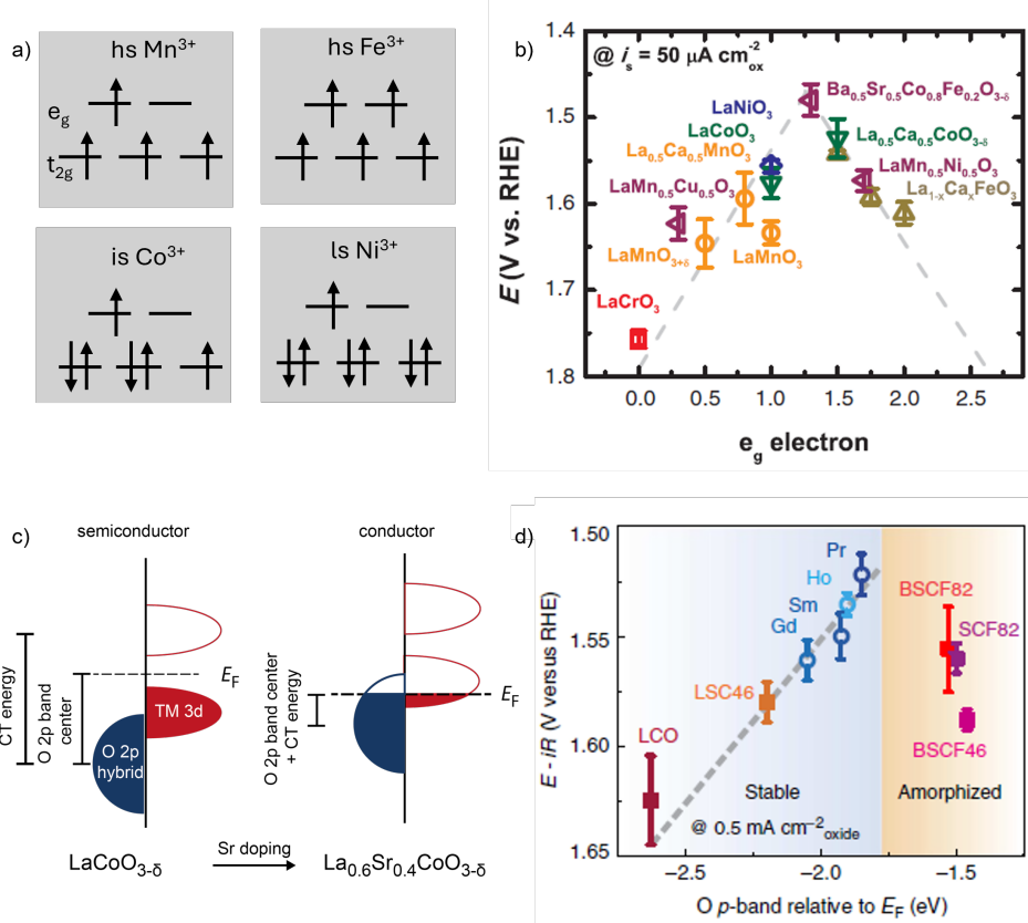
Figure 5: a) Spin configuration and e_g filling of LaMnO_{3-\delta} , LaFeO_{3-\delta} , LaCoO_{3-\delta} and LaNiO_{3-\delta} in line with ref. [13]. b) Volcano trend of the OER potential at 50\ \mu A\ cm^{-2} in dependence of the catalyst e_g filling published by Suntivich et al. from [13]. Reprinted with permission from AAAS. c) Band structure of a semiconductor and semi-metal, where the O 2p band center and charge transfer (CT) energy are drawn in. d) Volcano trend of the OER potential at 500\ \mu A\ cm^{-2} in dependence of the catalyst O 2p band center published by Grimaud et al. [83]. Reproduced with permission from Springer Nature.
