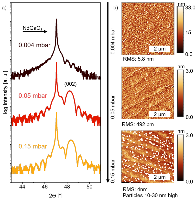
Figure 20: a) XRD b) AFM of 20 nm thick \text{La}_{0.6}\text{Ca}_{0.4}\text{CoO}_{3-\delta} thin films grown on \text{NdGaO}_3 substrates with increasing \text{O}_2 partial pressure.
