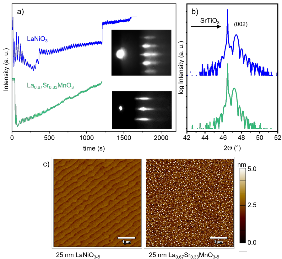
Figure A.1: a) RHEED intensity oscillations of the specular spot for 25 nm thick \text{LaNiO}_{3-\delta} , \text{La}_{0.67}\text{Sr}_{0.33}\text{MnO}_{3-\delta} thin films deposited on \text{SrTiO}_3 . Inset: final RHEED pattern. b) XRD of the two thin films after electrochemical treatment. c) AFM scans of the corresponding thin films. The thin films were fabricated by Iris van den Bosch, Emma van der Minne and Ellen Kiens at the University of Twente (Netherlands).
