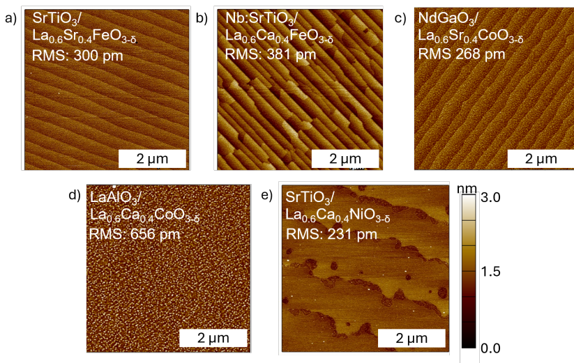
Figure 28: AFM scans of the perovskites oxide grown on the substrates with the best lattice match to the substrate a) \text{La}_{0.6}\text{Sr}_{0.4}\text{FeO}_{3-\delta} b) \text{La}_{0.6}\text{Ca}_{0.4}\text{FeO}_{3-\delta} c) \text{La}_{0.6}\text{Sr}_{0.4}\text{CoO}_{3-\delta} d) \text{La}_{0.6}\text{Ca}_{0.4}\text{CoO}_{3-\delta} e) \text{La}_{0.6}\text{Ca}_{0.4}\text{NiO}_{3-\delta} .
