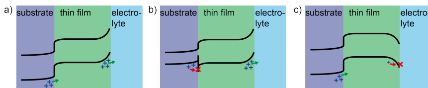
Figure 6: Band bending at the substrate/thin film interface and thin film/electrolyte interface. Holes need to move toward the electrolyte in order to receive the incoming electrons from the OER. a) Upward band bending is beneficial for the hole transport at both interfaces. b) At the substrate/thin film interface the bands are bent downward, hindering sufficient hole transport. c) At the thin film/electrolyte interface, hole transport to the electrolyte is hindered due to downward band bending. This illustration is inspired by [23].
