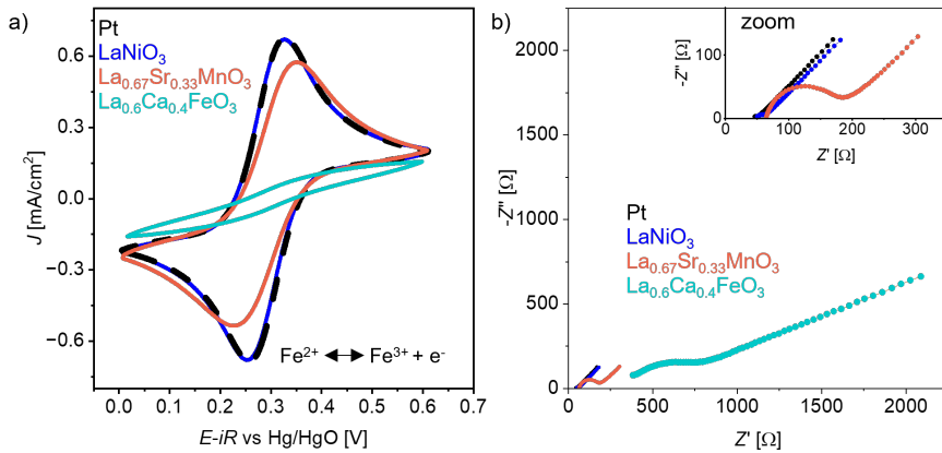
Figure 41: a) CV scans of \text{LaNiO}_{3-\delta} , \text{La}_{0.67}\text{Sr}_{0.33}\text{MnO}_{3-\delta} and \text{La}_{0.6}\text{Ca}_{0.4}\text{FeO}_{3-\delta} in \text{K}_4[\text{Fe}(\text{CN})_6]/\text{K}_3[\text{Fe}(\text{CN})_6] solution. The sweep rate was 30 mV/s. b) Corresponding impedance spectroscopy measured at OCP. The inset shows a zoom to the region of 0-350 \Omega in Z' direction. The figure was adapted by the color scheme from our publication [176], with the rights of the license CC-BY 4.0.
