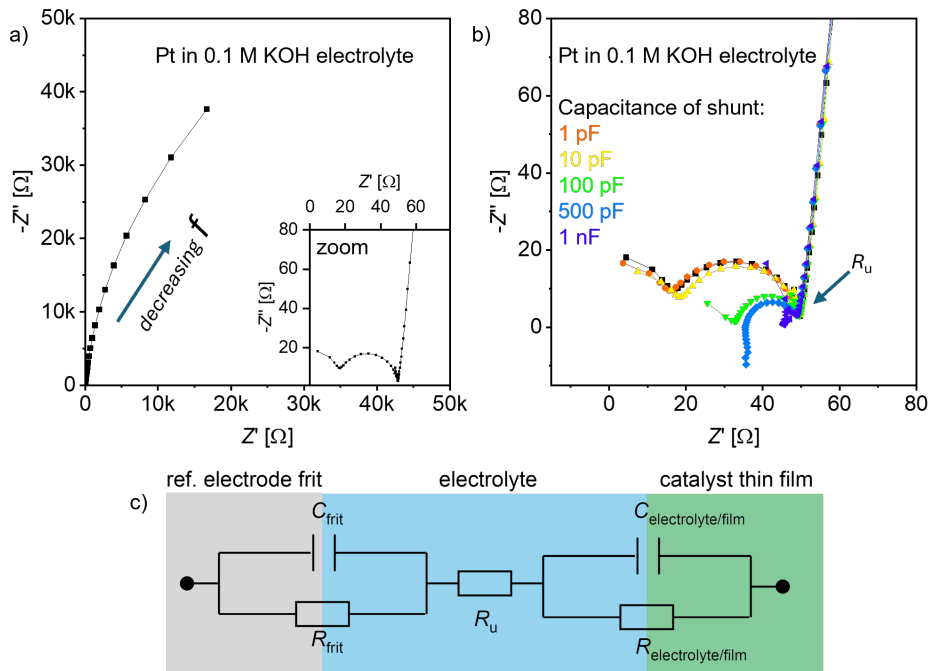
Figure 15: a) PEIS at OCP for a 50 nm thick Pt sample in 0.1 M KOH electrolyte. The initial part of a large semicircle is seen, which is attributed to the Pt thin film/electrolyte interface RC_{film/electrolyte} . The graph inset shows the zoom to the high-frequency region. A small semicircle is observed. b) The same Pt sample is tested in 0.1 M KOH electrolyte, where a shunt is connected in parallel to the reference electrode. The shunt was tested with various capacitor sizes from 1 pF to 1 nF. The size of the capacitor directly influences the small semicircle.
