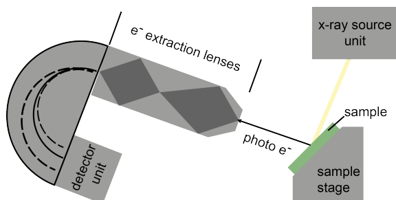
Figure 11: X-ray photo electron spectroscopy working principle. Sketch is inspired by [135].
