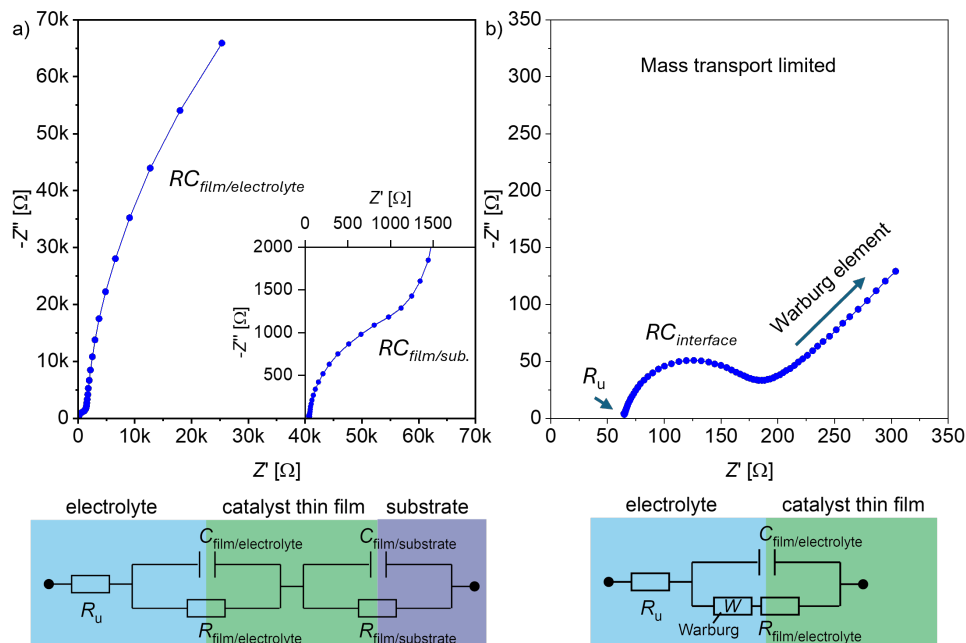
Figure 16: a) PEIS at OCP for a perovskite oxide catalyst thin film deposited on Nb:SrTiO 3 . The RC_{film/electrolyte} is here also seen toward lower frequencies. The semicircle seen in the graph inset stems from the RC_{film/substrate} interface. The signal of the reference electrode is cut off. b) PEIS at OCP in hexacyanoferrate (II)/(III) electrolyte. A charge transfer resistance from an interface is seen and a 45° incline towards low frequencies, which stems from a Warburg impedance.
