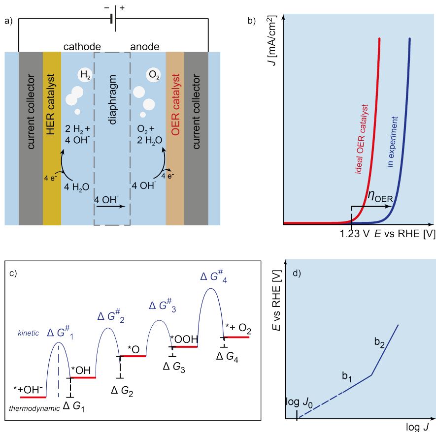
Figure 1: a) Sketch of an alkaline water electrolyzer. b) Cyclic voltammetry example of an ideal OER catalyst and catalyst in experiment, where an additional overpotential \eta_{\text{OER}} has to be applied to drive the reaction. c) Sketch of a Gibbs free energy diagram of the four electron transfer steps in the OER adapted from [41–43]. \Delta G_n is the thermodynamic energy difference from one reaction intermediate ( ^*\text{OH} , ^*\text{O} , ^*\text{OOH} , ^* + \text{O}_2 ) to another. \Delta G_n^\# is the kinetic energy of each step that has to be overcome to form the subsequent reaction intermediate. d) Illustration of the Tafel plot with two different Tafel slopes b_1 and b_2 .
