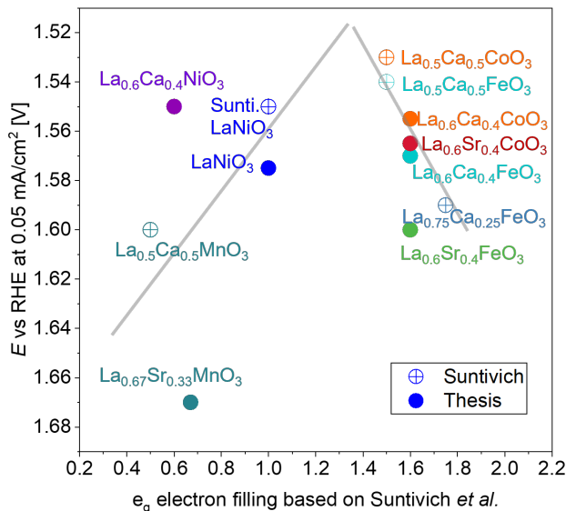
Figure 51: OER potential at 50\ \mu A\ cm^{-2} in correlation to the e_g filling from Suntivich et al. and this thesis.
