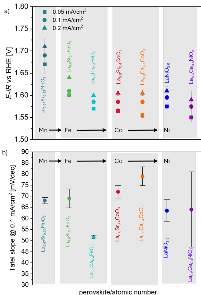
Figure 49: a) OER potential of the seven perovskites at 0.05, 0.1 and 0.2 mA cm -2 averaged from 2 samples for each perovskite. The values were taken from the geometries explained in table 15. The error bars stem from the average of those two samples. The CV scans of those can be viewed in the appendix F.3. b) Averaged Tafel slope values at 0.1 mA cm -2 of the same samples.
