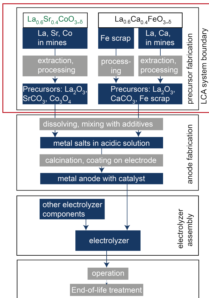
Figure 54: Life cycle of an alkaline water electrolyzer with projected production pathways for perovskite oxides \text{La}_{0.6}\text{Sr}_{0.4}\text{CoO}_{3-\delta} and \text{La}_{0.6}\text{Ca}_{0.4}\text{FeO}_{3-\delta} catalysts for the anode. The LCA system boundary includes material extraction, transportation, and precursor production.
