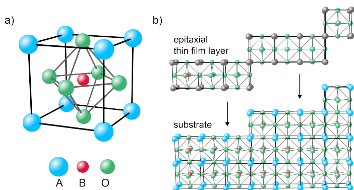
Figure 2: a) One perovskite oxide unit cell. b) Single crystalline substrate in the bottom and epitaxial thin film monolayer at the top, illustration is inspired by Weber et al. [33].
