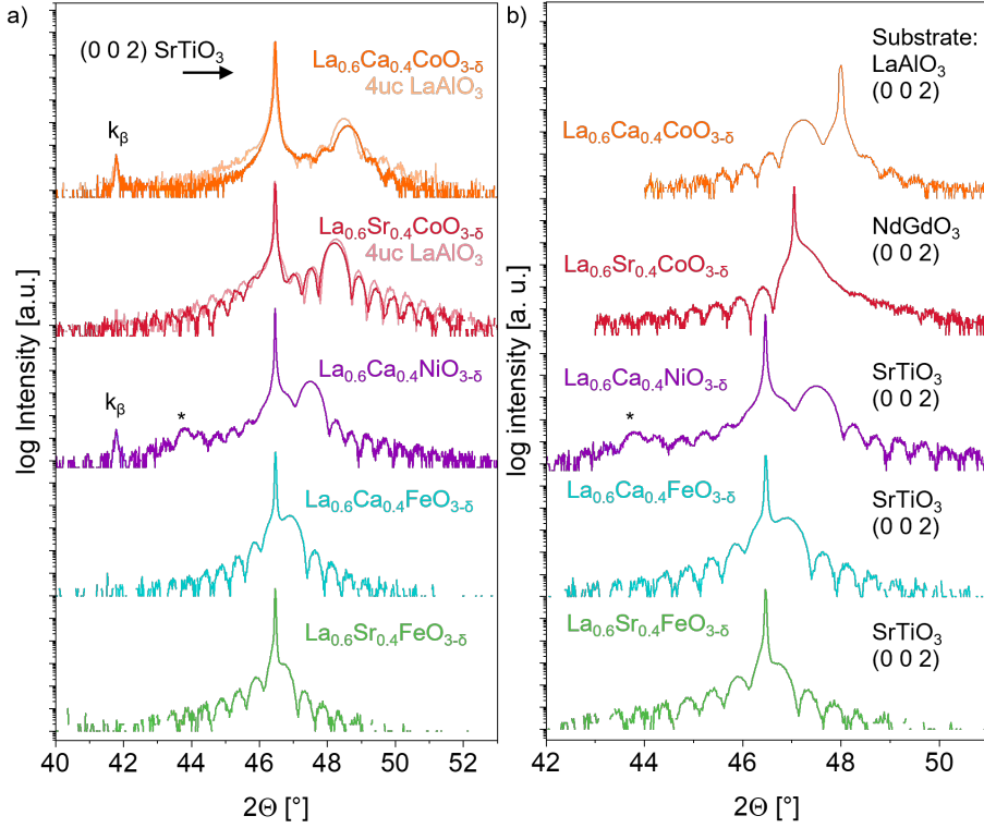
Figure 26: a) (002) reflex of perovskite oxides grown on (001) SrTiO 3 . b) Grown on least strain for the cobaltates; La 0.6 Ca 0.4 CoO 3-δ on a LaAlO 3 substrate and La 0.6 Sr 0.4 CoO 3-δ on a NdGaO 3 substrate.
