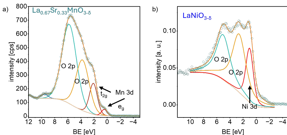
Figure A.2: XPS valence band spectrum with component fits of a) \text{La}_{0.67}\text{Sr}_{0.33}\text{MnO}_{3-\delta} measured by Emma van der Minne. b) XPS valence band spectrum of \text{LaNiO}_{3-\delta} which was taken from Kante et al. [170], with the CC-BY 4.0 license.
