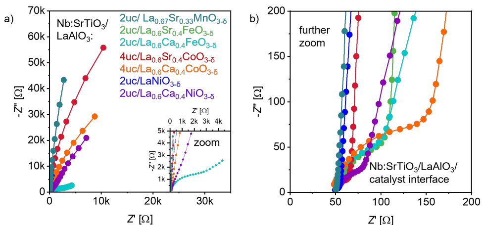
Figure 47: Impedance spectroscopy at OCP of the seven perovskite stacks on Nb:SrTiO 3 /LaAlO 3 stacks in 0.1 M KOH. The uc numbers in the legend represent the LaAlO 3 interlayer thickness. a) Shows low-frequency range with the initial part of the large semi-circle of the thin film/electrolyte interface; inset shows the zoom to the La 0.6 Ca 0.4 FeO 3-δ impedance. b) Zoom to the high-frequency region, showing the area of the R_u and contact resistance at the Nb:SrTiO 3 /LaAlO 3 /catalyst interface. The legend from a) applies also to b).
