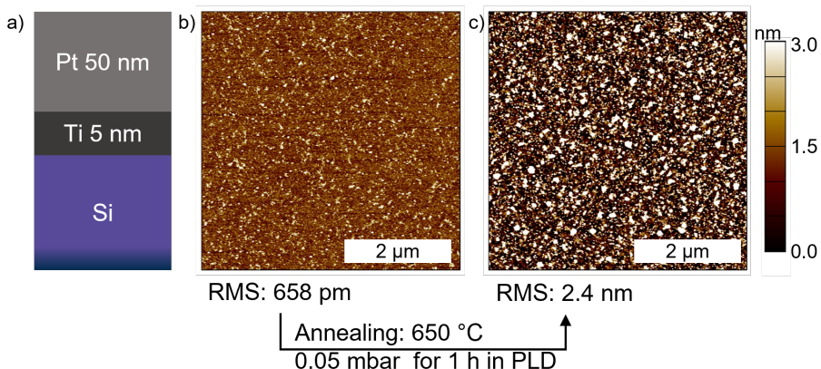
Figure 33: a) Platinized silicon stack: Si substrate, 5 nm Ti adhesive layer and 50 nm Pt. b) Surface morphology of Pt layer. c) Surface morphology of Pt after annealing for 1 h.
