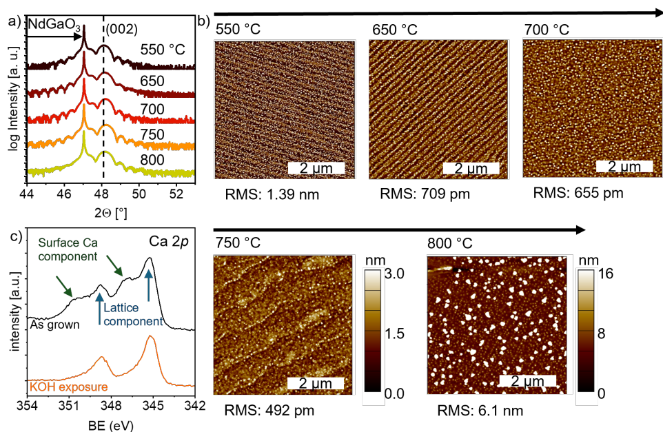
Figure 19: XRD scans recorded in the range of the (002) peak of 20 nm thick \text{La}_{0.6}\text{Ca}_{0.4}\text{CoO}_{3-\delta} thin films that were grown on \text{NdGaO}_3 substrates with increasing temperature. b) AFM of corresponding thin films with increasing temperature as listed along the arrows. c) \text{La}_{0.6}\text{Ca}_{0.4}\text{CoO}_{3-\delta} thin film XPS data of the Ca 2p core level are shown in the as-prepared state and after exposure to 0.1 M KOH solution.
