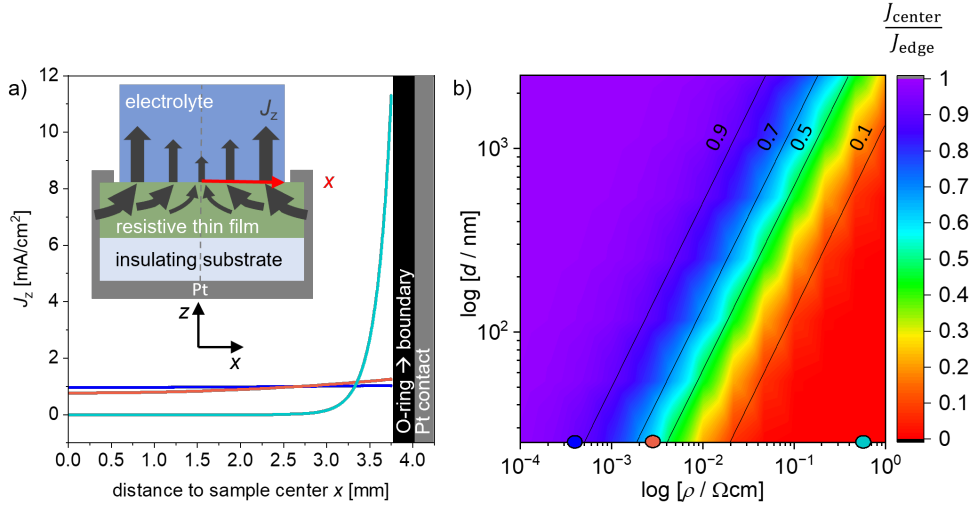
Figure 42: a) Simulated current density distribution of the thin films on insulating substrates. The inset shows a sketch of the radial current density distribution J_z(x) on resistive thin films along the x -axis of the simulation. The dashed line in the center represents the axisymmetric line cut. b) Heat map of the current density variation J_{\text{center}}/J_{\text{edge}} as a function of catalyst layer resistivity \rho and thickness d . Blue, green, and orange dots are the data points for 25 nm thick LaNiO 3-δ , La 0.67 Sr 0.33 MnO 3-δ and La 0.6 Ca 0.4 FeO 3-δ thin films, respectively. The figure was adapted by the color scheme from our publication [176], with the rights of the license CC-BY 4.0.
