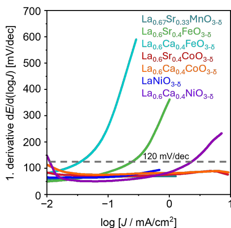
Figure 40: First derivative of the Tafel plots of the averaged CV scans from figure 39b. The first derivative represents the Tafel slope at each point of the increasing current density.
