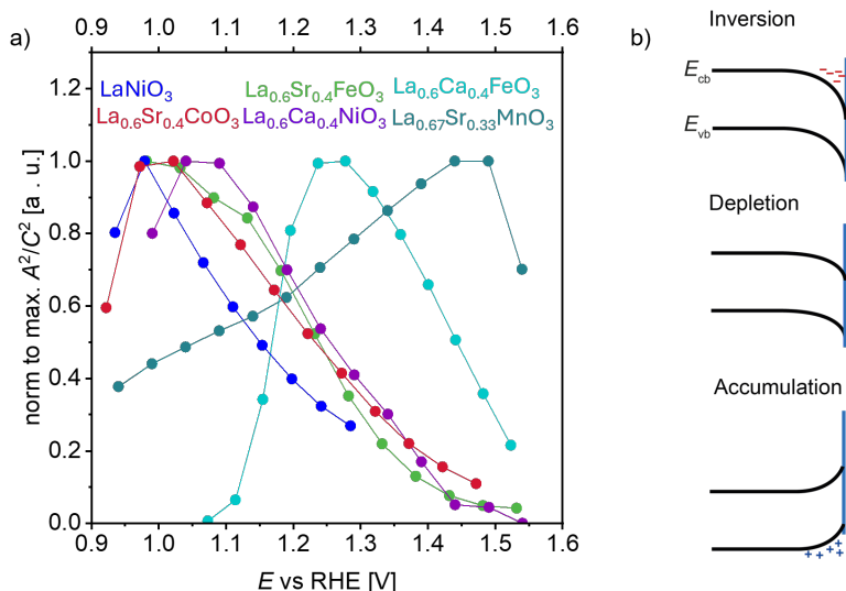
Figure 46: a) Mott-Schottky plots from OCP to near OER conditions normalized to the maximum. The analysis and the \text{La}_{0.6}\text{Sr}_{0.4}\text{CoO}_{3-\delta} plot are adapted from Heymann et al. [34], with the rights of the license CC-BY 4.0. b) Sketch of the band bending at the catalyst/electrolyte interface with an inversion (top), hole depleted (middle), and hole accumulated space charge layer (bottom) [34].
