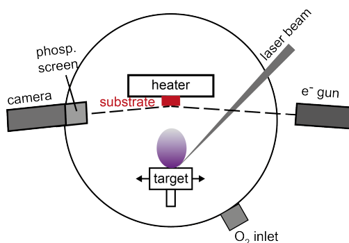
Figure 8: Design of the here used PLD system; scetch inspired by [123]. The UV laser hits the moving target. The plasma plume (purple) evolves and propagates to the substrate, which is glued to the heater. For in-situ growth detection a reflective high energy electron diffraction (RHEED) system is installed, with the electron gun focused in an incident angle on the substrate surface, and reflected to the phosphorous screen. The screen is filmed by a CCD camera (more details in section 3.2).
