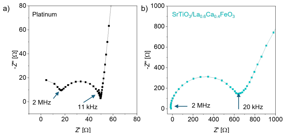
Figure E.1: a) Nyquist plot of a Pt sample in the high frequency range. The sample was placed in 0.1 M KOH and the impedance was measured at OCP. There is a semicircle observed between 2 MHz and 11 kHz. When the reference electrode is equipped with a shunt that consists of a Pt wire and capacitor in parallel, the impedance feature systematically changes with capacitor size (section 3.6.2) Hence, the impedance feature can be attributed to the frit of the reference electrode, as was also described in the literature [138]. At 11 kHz, the imaginary part of the impedance is zero and the x-axis offset represents the uncompensated resistance R_u . At lower frequencies, a large incline is seen which is attributed to the working electrode solid/liquid interface. b) Nyquist plot of 25 nm \text{La}_{0.6}\text{Ca}_{0.4}\text{FeO}_{3-\delta} on \text{SrTiO}_3 in the high frequency range. The impedance signal from the reference electrode (dominating at high frequencies) overlaps with the impedance signal of the working electrode and therefore -Z'' does not reach zero. This hinders an accurate determination of the R_u .
