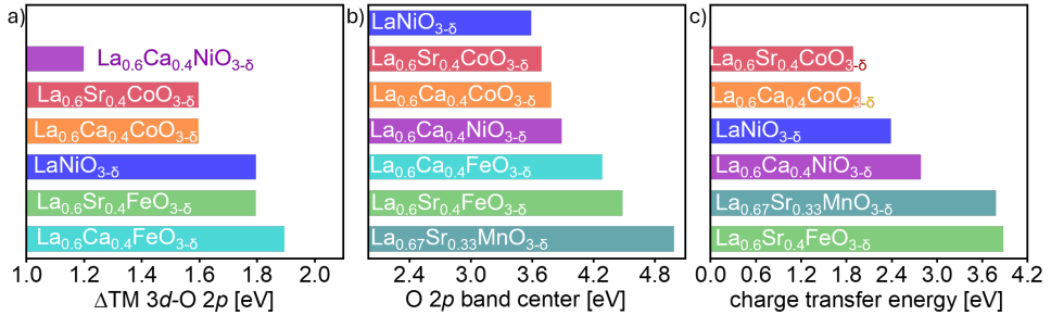
Figure 32: \Delta\text{TM } 3d\text{-O } 2p , O 2 p band center and charge transfer energy of the perovskite oxides sorted by decreasing energy values from bottom to top.
