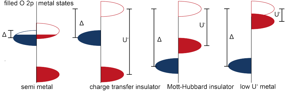
Figure 3: Metal to insulator transition of the charge transfer and Mott-Hubbard type adapted from [55, 56].
