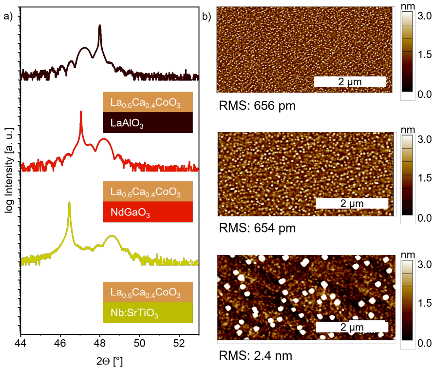
Figure 21: \text{La}_{0.6}\text{Ca}_{0.4}\text{CoO}_{3-\delta} grown on the different substrates \text{LaAlO}_3 , \text{NdGaO}_3 and \text{SrTiO}_3 to induce compressive and tensile strain. a) shows the XRD and b) the AFM.
