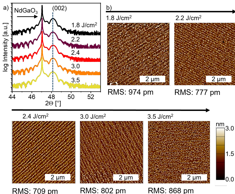
Figure 18: a) XRD scans recorded in the range of the (002) peak of 20 nm thick \text{La}_{0.6}\text{Ca}_{0.4}\text{CoO}_{3-\delta} epitaxial thin films grown on \text{NdGaO}_3 substrates with increasing laser fluence as listed accordingly. b) Corresponding AFM scans with increasing laser fluence as listed along the arrows. Particles are seen on every surface. THE RMS is the lowest at a laser fluence of 2.4 \text{ J/cm}^2 .
