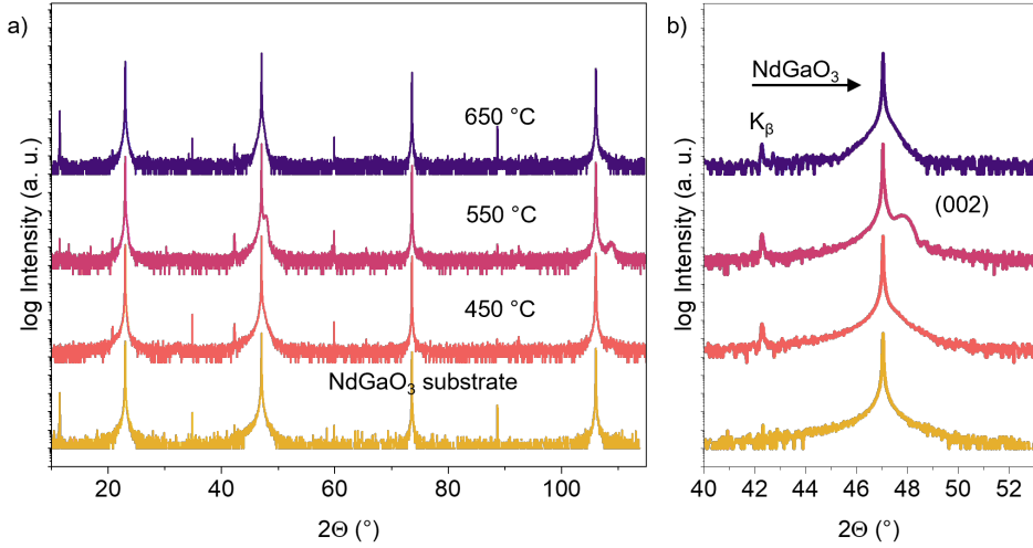
Figure 24: Temperature series of \text{La}_{0.6}\text{Ca}_{0.4}\text{NiO}_{3-\delta} a) XRD from 10^\circ - 120^\circ in 2\theta - \omega geometry. The yellow graph shows the \text{NdGaO}_3 substrate as reference. b) Zoom to the (002) peak.
