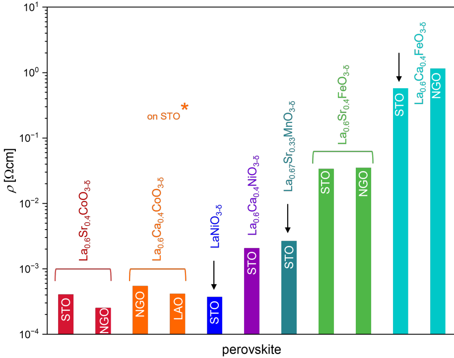
Figure 29: Resistivity trend of the here investigated perovskite oxides: on different insulating substrates, inducing different strain states. \text{La}_{0.6}\text{Ca}_{0.4}\text{CoO}_{3-\delta} showed high resistivity grown on \text{SrTiO}_3 . As its origin could be related to some other effects it is only marked with a star.
