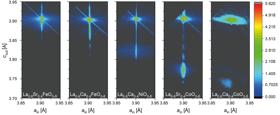
Figure 27: RSM of the perovskites on \text{SrTiO}_3 . The strain increases from the ferrates to the cobaltates.
