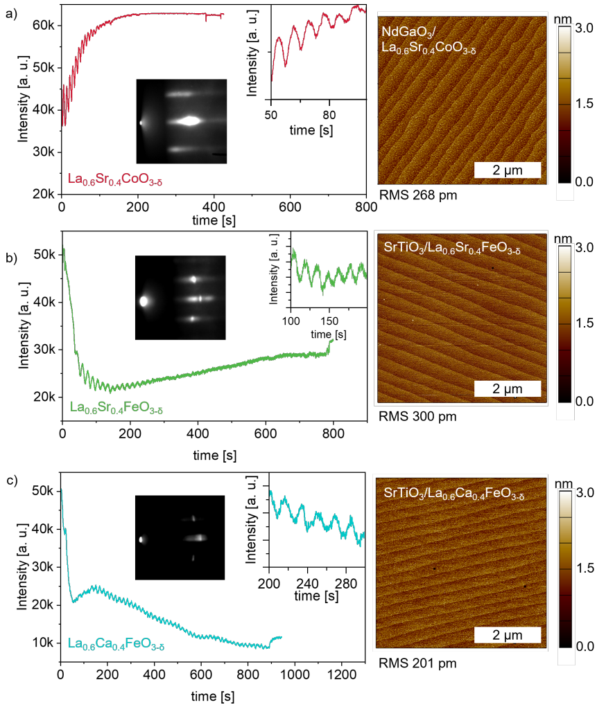
Figure 17: PLD deposition of a) \text{La}_{0.6}\text{Sr}_{0.4}\text{CoO}_{3-\delta} on \text{NdGaO}_3 b) \text{La}_{0.6}\text{Sr}_{0.4}\text{FeO}_{3-\delta} on \text{SrTiO}_3 and c) \text{La}_{0.6}\text{Ca}_{0.4}\text{FeO}_{3-\delta} on \text{SrTiO}_3 . The RHEED oscillations are shown on the left, the RHEED pattern after deposition of 20 nm in the inset, and the surface morphology on the right.
