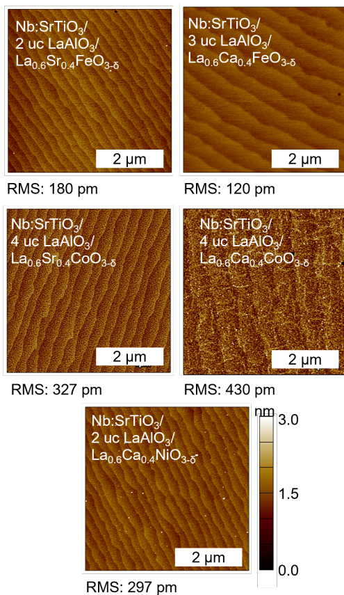
Figure B.1: AFM of the five perovskites grown by PLD on Nb:SrTiO 3 with 2-4 unit cell thick LaAlO 3 interlayer. The thin films were used for electrochemical characterization.
