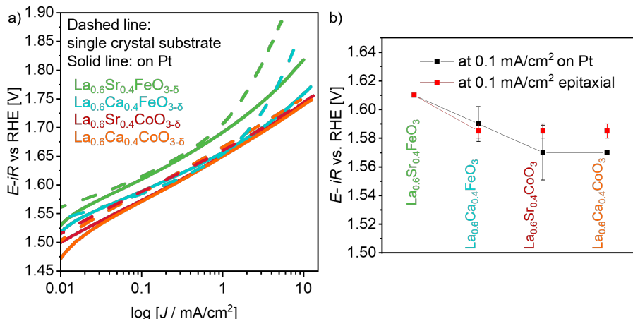
Figure F.4: a) Compares representative CV curves of \text{La}_{0.6}\text{Sr}_{0.4}\text{FeO}_{3-\delta} , \text{La}_{0.6}\text{Ca}_{0.4}\text{FeO}_{3-\delta} , \text{La}_{0.6}\text{Sr}_{0.4}\text{CoO}_{3-\delta} and \text{La}_{0.6}\text{Ca}_{0.4}\text{CoO}_{3-\delta} grown on single-crystal substrates (the ferrates on \text{Nb:SrTiO}_3/\text{LaAlO}_3 , \text{La}_{0.6}\text{Sr}_{0.4}\text{CoO}_{3-\delta} on \text{NdGaO}_3 and \text{La}_{0.6}\text{Ca}_{0.4}\text{CoO}_{3-\delta} on \text{LaAlO}_3 ) with the thin films grown on Pt from figure 50b. In the low current density range (0.1-1 \text{mA cm}^{-2} ), the OER activity of the ferrates grown on single crystalline substrates is very similar to that of the ferrates grown on Pt. Therefore, the influence of the different surface roughnesses, crystal facets, or grain boundaries on the ferrate OER activity seems small. At high current densities, the ferrates grown on Pt remain with high activity, while the ferrates grown on \text{Nb:SrTiO}_3/\text{LaAlO}_3 /thin film show increasing overpotential due to the remaining substrate/thin film interface resistance. Still, a change in slope is seen for the ferrates grown on Pt, which stems from changes in reaction kinetics or small thin film resistances as seen in figure 50c. The two cobaltates grown on single-crystal substrates show slightly higher overpotentials at low current densities compared to the thin films deposited on Pt, but are similar in the higher current density range. Possibly, crystal facet orientation or grain boundary effects might play a role here. However, the surface roughness seems to have a minor influence, as for example the \text{La}_{0.6}\text{Ca}_{0.4}\text{CoO}_{3-\delta} film on Pt has an RMS of 11 nm while the single crystal has an RMS below 1 nm. b) OER potential at a current density of 0.1 \text{mA cm}^{-2} of the epitaxial thin films in comparison to the polycrystalline thin films grown on Pt. The error bar stems from three different samples grown on Pt. The error bars for the epitaxial thin films stem from two averaged samples. The two ferrates show on both substrate types similar OER activity at this current density. The two cobaltates vary slightly. On Pt, the OER potential is lower for the cobaltates, but the standard deviation of \text{La}_{0.6}\text{Sr}_{0.4}\text{CoO}_{3-\delta} is much higher than for the ferrates. This might result from a higher influence of e.g. different crystal facets or grain boundaries. Some \text{La}_{0.6}\text{Ca}_{0.4}\text{FeO}_{3-\delta} thin films grown on Pt had the same catalytic activity as some \text{La}_{0.6}\text{Sr}_{0.4}\text{CoO}_{3-\delta} thin film layers on Pt.
