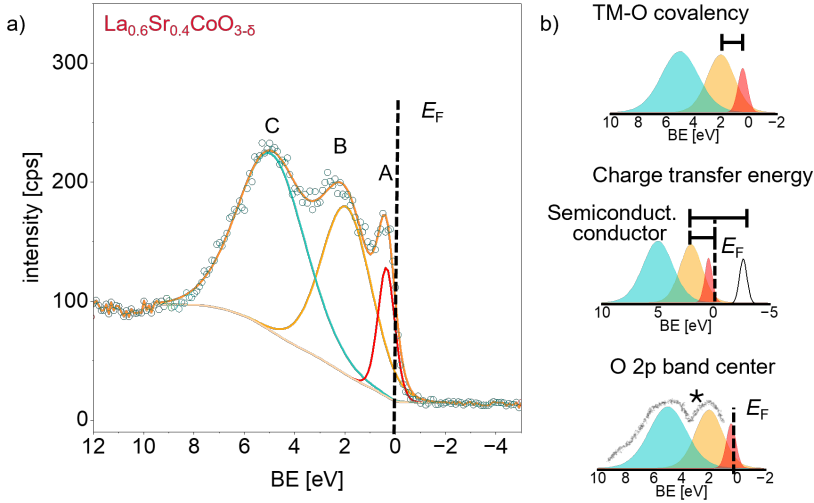
Figure 30: a) XPS valence band spectrum of \text{La}_{0.6}\text{Sr}_{0.4}\text{CoO}_{3-\delta} fitted with three components. b) Illustration of the approaches to determine the electronic structure descriptors. \Delta\text{TM } 3d\text{-O } 2p is the distance between peak A and B, referring to predominantly TM 3d and O 2p states. The charge transfer energy is the distance from peak B to the Fermi level for highly conducting perovskites, and for semiconducting material the peak B to the first unoccupied state. The O 2p band center is the centroid of peak B and C in distance to the Fermi level.
