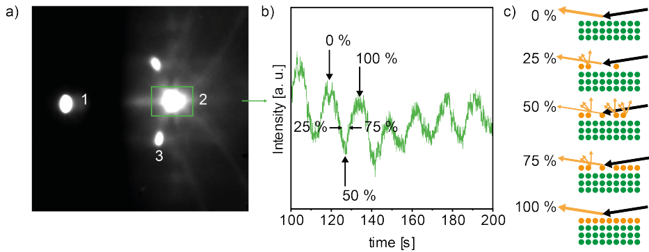
Figure 9: a) RHEED pattern of a \text{SrTiO}_3 surface. No.1 is the primary electron beam, no. 2 is the specular spot, no.3 are the diffractive spots (bottom and top). The green square indicates the area where intensity changes are tracked. b) This results in the oscillations for layer-by-layer growth over time. The percentages represent the progress of one growing monolayer. c) Schematic of the roughening and subsequent smoothing of the surface during the growth of one monolayer. The black arrow represents the incoming electron beam, the orange beam represents the reflected electron beam, and the smaller orange arrows represent the scattered electrons, reducing the intensity of the specular spot.
