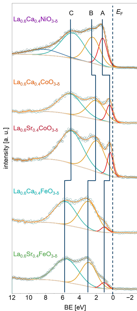
Figure 31: XPS Valence band spectra with increasing atomic number from bottom to top, \text{La}_{0.6}\text{Sr}_{0.4}\text{FeO}_{3-\delta} , \text{La}_{0.6}\text{Ca}_{0.4}\text{FeO}_{3-\delta} , \text{La}_{0.6}\text{Sr}_{0.4}\text{CoO}_{3-\delta} , \text{La}_{0.6}\text{Ca}_{0.4}\text{CoO}_{3-\delta} , and \text{La}_{0.6}\text{Ca}_{0.4}\text{NiO}_{3-\delta} ; recorded in a 15^\circ photoemission angle. Red: transition metal 3d peak, yellow: O 2p peak, blue: hybrid states.
