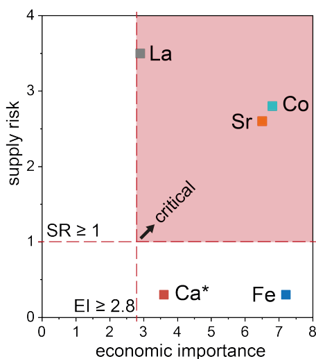
Figure 55: EU criticality assessment for the raw materials used for \text{La}_{0.6}\text{Sr}_{0.4}\text{CoO}_{3-\delta} and \text{La}_{0.6}\text{Ca}_{0.4}\text{FeO}_{3-\delta} adapted from [93]. Ca* is limestone and Fe the iron ore.
