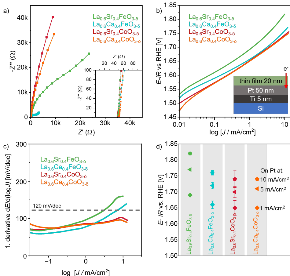
Figure 50: a) OCP impedance of 20 nm thick \text{La}_{0.6}\text{Sr}_{0.4}\text{FeO}_{3-\delta} , \text{La}_{0.6}\text{Ca}_{0.4}\text{FeO}_{3-\delta} , \text{La}_{0.6}\text{Sr}_{0.4}\text{CoO}_{3-\delta} , \text{La}_{0.6}\text{Ca}_{0.4}\text{CoO}_{3-\delta} thin films on Si/Ti 5 nm/Pt 50 nm stacks. b) Tafel-like plots of the thin films. c) Tafel slope plots of the catalysts on Pt. d) OER potentials of the four perovskites on Pt at 1, 5, and 10 \text{mA}/\text{cm}^2 .
