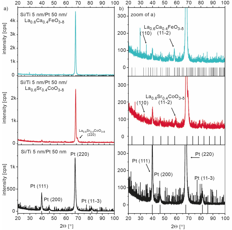
Figure 37: a) GIXRD of \text{La}_{0.6}\text{Sr}_{0.4}\text{CoO}_{3-\delta} , \text{La}_{0.6}\text{Ca}_{0.4}\text{FeO}_{3-\delta} grown on Pt thin films, the bottom scan stems from a Pt thin film sample as a reference. b) Zoom of a) to the lower intensity regime.
