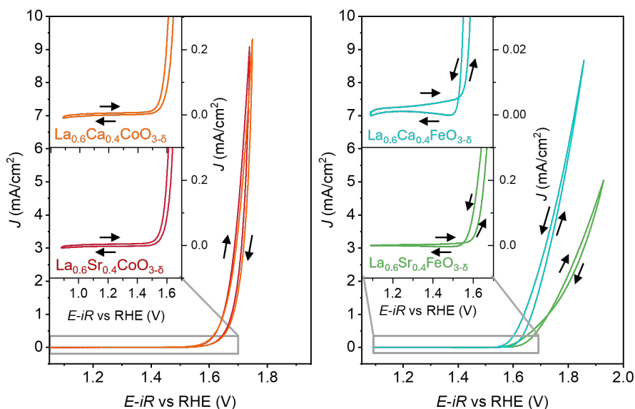
Figure F.2: CV scan from close to OCP to the OER voltage regime. The scan rate was 10 mV/s. a) shows the CV from the two cobaltates grown on insulating substrates \text{NdGaO}_3 and \text{LaAlO}_3 . The hysteresis is caused by capacitive charging and discharging. b) shows the CV of the two ferrates. The hysteresis is anomalous. The backward sweep shows higher current densities than the forward sweep from the current density maximum to 1.5 V vs RHE. Then it crosses the forward sweep. The backward sweep of \text{La}_{0.6}\text{Sr}_{0.4}\text{FeO}_{3-\delta} crosses at around 1.7 V vs RHE the forward sweep for the first time and at 1.5 V vs RHE for the second time. The reasons could be a change in coverage, rate-determining step or change in oxidation state. However, this remains an open question.
