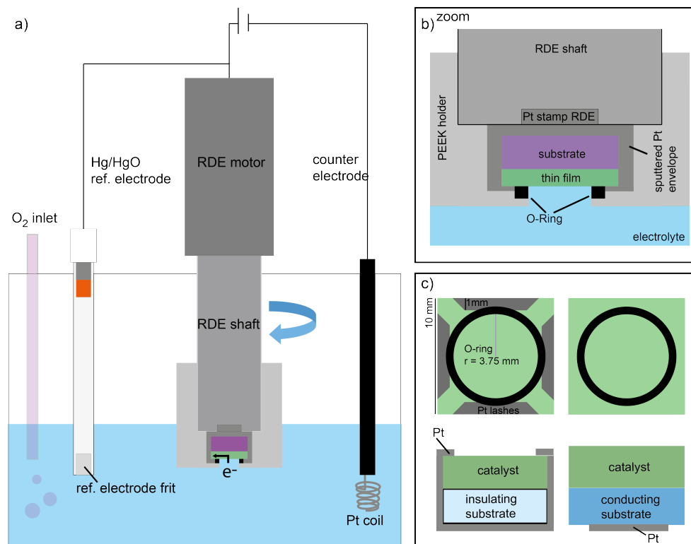
Figure 13: a) 3-electrode RDE setup. The \text{Hg}/\text{HgO} reference electrode, Pt counter electrode, and RDE with attached thin film are immersed in the electrolyte. The electrolyte is purged with \text{O}_2 gas. b) Zoom to the RDE shaft where the sample is mounted. The sample is placed in a custom-made PEEK holder. The backside and edges are sealed with an O-ring from the electrolyte. c) Pt contacts sputtered for insulating substrates (left) and for \text{Nb}:\text{SrTiO}_3 substrates (right).
