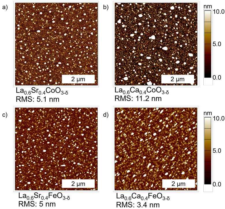
Figure 34: AFM of a) La 0.6 Sr 0.4 CoO 3-δ b) La 0.6 Ca 0.4 CoO 3-δ c) La 0.6 Sr 0.4 FeO 3-δ d) La 0.6 Ca 0.4 FeO 3-δ grown on Si/Ti 5 nm/Pt 50 nm.
