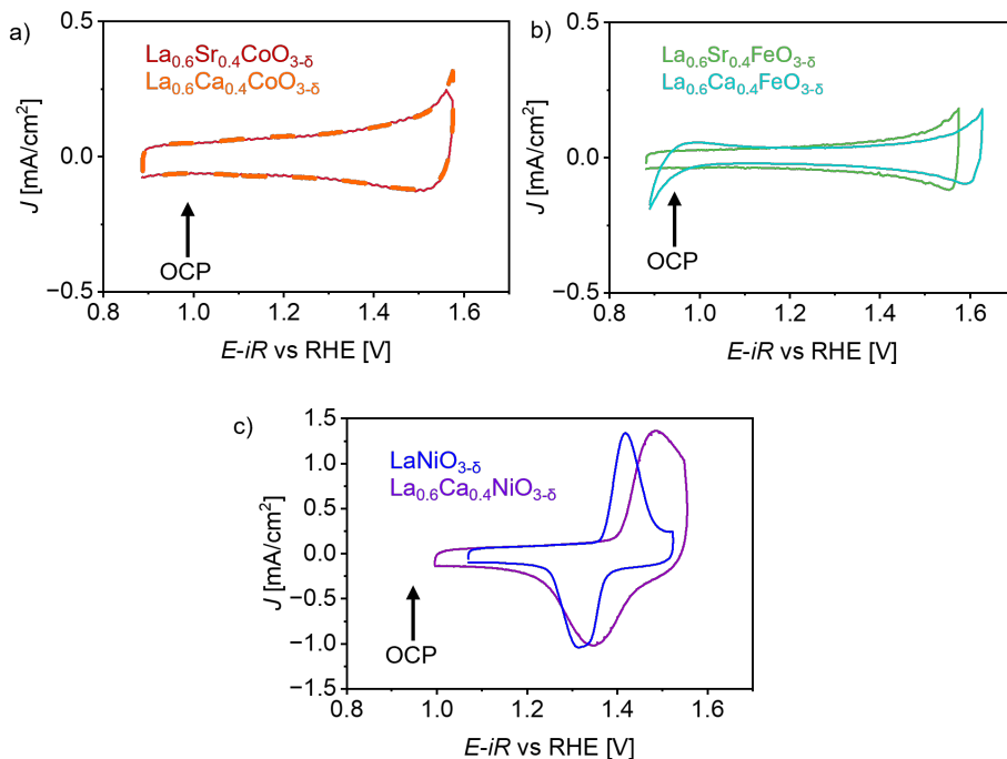
Figure F.1: CV scans of a) \text{La}_{0.6}\text{Sr}_{0.4}\text{CoO}_{3-\delta} , \text{La}_{0.6}\text{Ca}_{0.4}\text{CoO}_{3-\delta} b) \text{La}_{0.6}\text{Sr}_{0.4}\text{FeO}_{3-\delta} , \text{La}_{0.6}\text{Ca}_{0.4}\text{FeO}_{3-\delta} and c) \text{LaNiO}_{3-\delta} , \text{La}_{0.6}\text{Ca}_{0.4}\text{NiO}_{3-\delta} from 0.9/1.0 V to about 1.6 V vs RHE with a scan rate of 500 mV s -1 . \text{La}_{0.6}\text{Ca}_{0.4}\text{FeO}_{3-\delta} undergoes a redox reaction in the OCP region, causing a lower impedance value at the solid/liquid interface. This is not the case for the other perovskites. Nevertheless, all perovskites show redox reactions towards the OER voltage regime. The two Nickelates exhibit strong redox peaks around 1.4 V vs RHE which is attributed to \text{Ni}^{2+}/\text{Ni}^{3+} [19].
