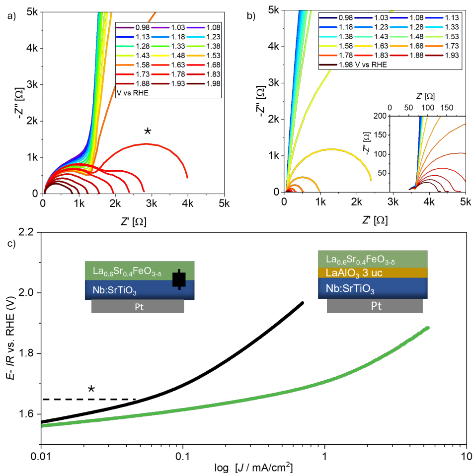
Figure 44: Stair case impedance spectroscopy towards the OER voltage regime in a) for Nb:SrTiO 3 / 20 nm La 0.6 Sr 0.4 FeO 3-δ and b) Nb:SrTiO 3 / 3 uc LaAlO 3 / 20 nm La 0.6 Sr 0.4 FeO 3-δ . As oxygen gas evolves, the RDE rotation is set to 1600 rpm. c) Tafel-like plot of the averaged, second CV scan with and without LaAlO 3 interlayer. The * marks where the catalyst/electrolyte interface impedance is still bigger than that of the substrate/thin film interface.
