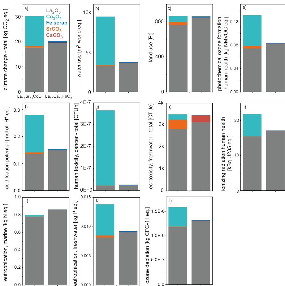
Figure 57: Environmental impact category results of the precursors required to produce 1 kg of \text{La}_{0.6}\text{Sr}_{0.4}\text{CoO}_{3-\delta} and \text{La}_{0.6}\text{Ca}_{0.4}\text{FeO}_{3-\delta} .
