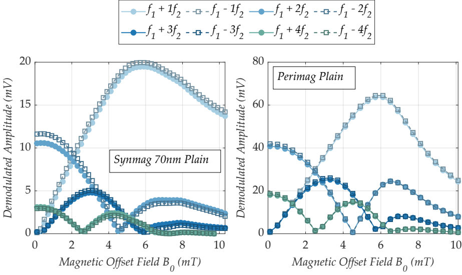
Figure 3.8: Offset-scan recorded with an offset magnetic field, generated through a DC in the LF coil in superposition to the LF magnetic field. This scan was recorded for Synmag 70nm (left) and Perimag (right) particles from Micromod Partikeltechnologie GmbH.
