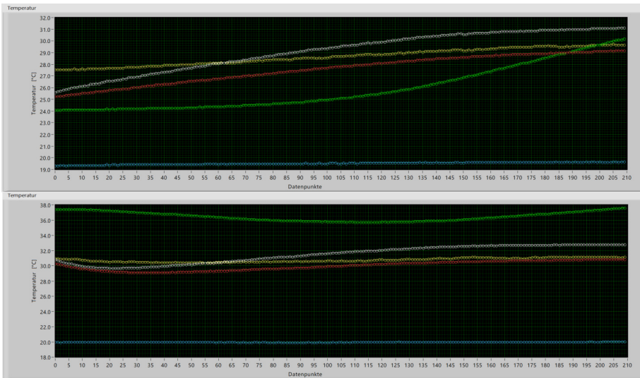
Figure I.1: Screen shots of temperature recordings in the MH (green graph) of the magnetic reader during offset scans with settings of LF500 and LF1000. A National Instruments DAQ and a custom LabView Software were used for data acquisition. The white, yellow and red graphs are recorded at different locations on the magnetic reader PCB. The blue graph indicates the temperature outside of the magnetic reader.
