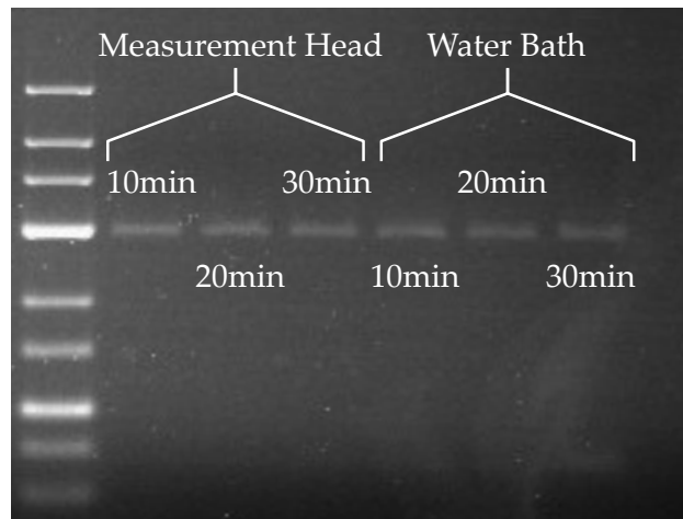
Figure 6.5: Gel image of RPA inside measurement head and water bath at different incubation times. Adopted and modified from [59].
