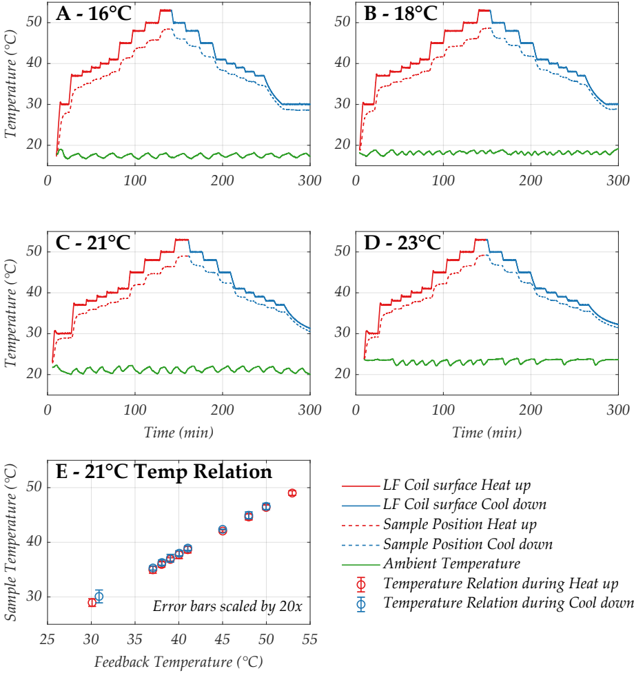
Figure 6.3: Recorded characterization data for feedback temperature control, sample position temperature and ambient (laboratory) temperature of 16 °C, 18 °C, 21 °C, 23 °C (A-D) and linear exemplary dependency of controller temperature vs. sample position temperature at 21 °C (E). The standard deviation bars in E are scaled by 20× and indicate the stability of the temperature control at sample position. Adopted and modified from [59].
