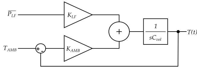
Figure 5.1: Block diagram of a lumped parameter model for the LF coil surface temperature.
