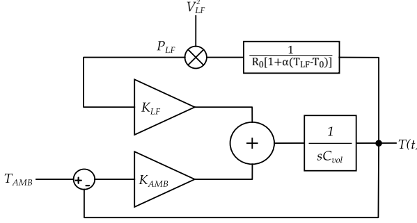
Figure 5.4: Block diagram of a lumped parameter model for the LF coil surface temperature depending on the changes in resistance with temperature.
