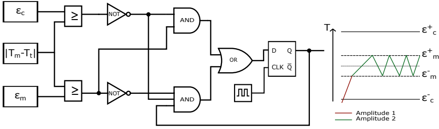
Figure 6.1: Equivalent logic for a PWM controller with differentially adjustable heating and measurement LF amplitude and schematic of controlled temperature using this logic.
