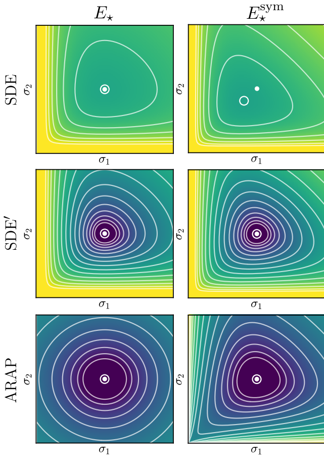
Figure 9: Following the visualization style of [ASGS23], we plot the energy landscape (dark colors correspond to small values) for different distortion measures and their symmetrized versions on [0, 2]^2 . The minimum of the function is indicated by a circle, and a dot at (1, 1) marks the expected location of the minimum for an isometry-promoting function. Note that the symmetrized version of the standard SDE does not promote isometry.
