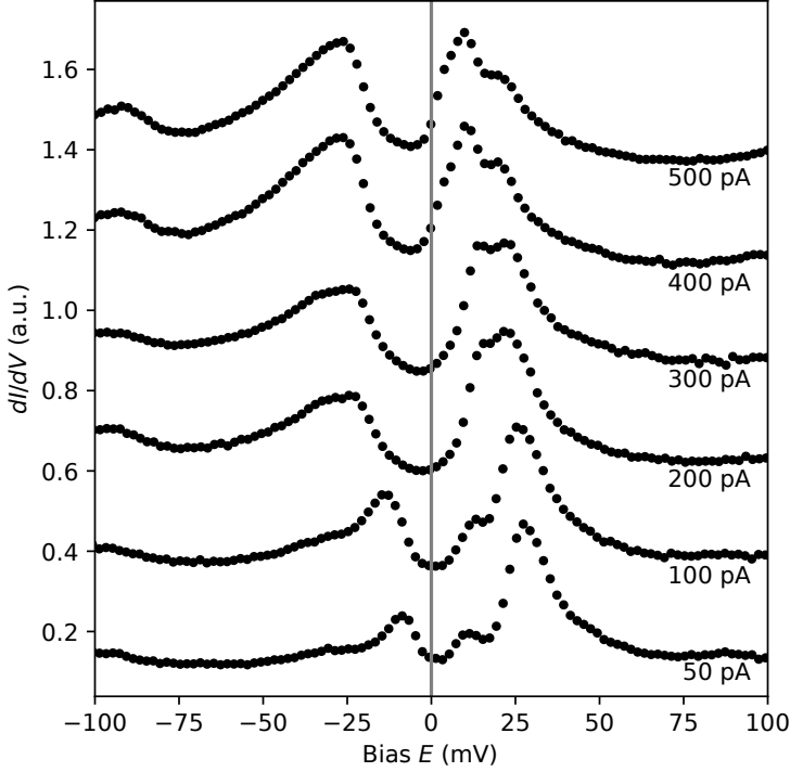
Fig. 6.14: Raw data of the scanning tunneling spectra of TBLG on hBN. The scan range is from -100 mV to 100 mV.
