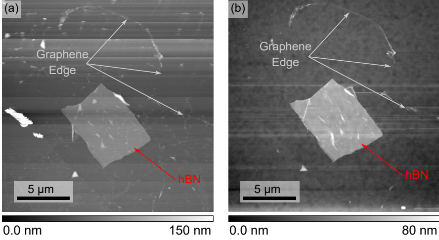
Fig. 6.6: AFM images of the twisted bilayer graphene on hBN (a) before and (b) after annealing in H/Ar atmosphere. 20 μm x 20 μm field of view (scan speed: 12 μm/s, setpoint: 1000 mV).
