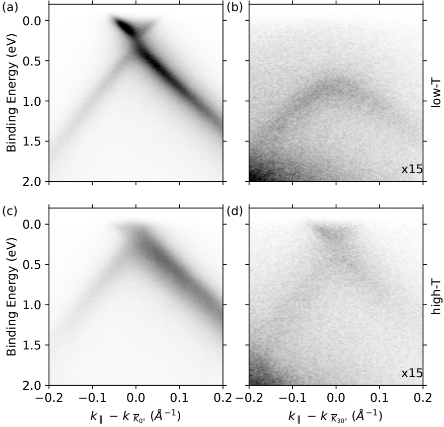
Fig. 5.3: (a, b) ARPES EDMs recorded at the \bar{K}_0 and \bar{K}_{30} points of the graphene layers along the \bar{\Gamma}\bar{K} direction of the low-T sample, respectively. (c, d) Same as (a, b) for the high-T sample.
