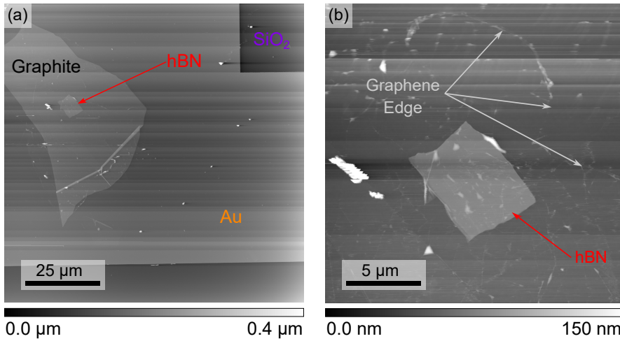
Fig. 6.5: AFM images of twisted bilayer graphene on hBN before annealing in H/Ar atmosphere. (a) 100 \mu\text{m} \times 100 \mu\text{m} field of view (scan speed: 60 \mu\text{m/s} , setpoint: 300 mV). (b) 20 \mu\text{m} \times 20 \mu\text{m} field of view (scan speed: 12 \mu\text{m/s} , setpoint: 1000 mV).
