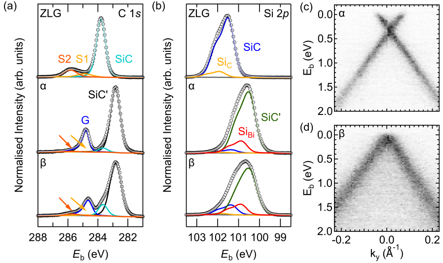
Fig. 3.1: (a, b) C 1s and Si 2p XP spectra of the ZLG, \alpha , and \beta phases of Bi-intercalated graphene on SiC(0001). For the \alpha and \beta phases, the components S1 and S2 are marked by yellow and red arrows, respectively. (c) ARPES data at the \bar{K} point of the graphene for the \alpha phase. (d) Same as (c) for the \beta phase. [98]
