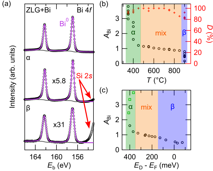
Fig. 3.2: (a) Bi 4f XP spectra of ZLG after Bi deposition but before intercalation (top) and of Bi-intercalated QFMLG after preparation of the \alpha (middle) and \beta phase (bottom) at 350°C and 900°C, respectively. Red arrows mark the shoulder of the Si 2s peak located just outside the scan range. The spectra are shifted vertically for clarity and normalized to the Bi 4f_{7/2} peak. (b) The amount of Bi A_{\text{Bi}} in the sample (according to equation 3.4, black circles) and the degree of intercalation D (equation 3.1, red crosses), plotted against the annealing temperature of the sample. (c) Amount of Bi A_{\text{Bi}} on the sample as a function of the energy of the Dirac point E_D , which is a measure of the graphene doping level [98].
