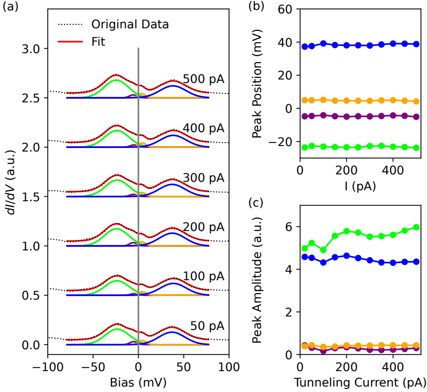
Fig. 6.19: (a) STS of TBLG on graphite. The scan range is from -100 mV to 100 mV. The original data and the fit are shown without background subtraction, but for the fit a quadractic background was subtracted. (b) Peak positions of the fit versus the tunneling current. The colors used correspond to the colors of the fits in (a). (c) Same as (a), but showing the peak amplitudes instead of positions.
