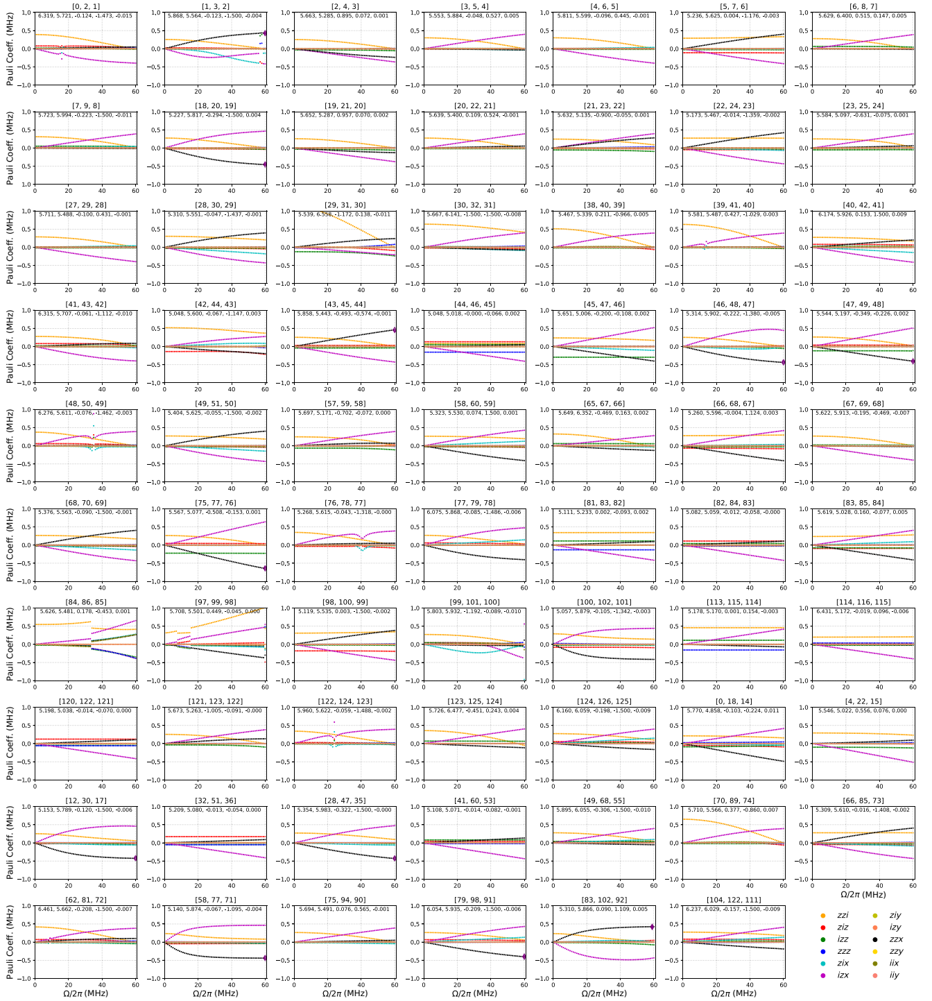
FIG. 11. Verification of Pauli coefficients for generating CZZ gate using optimized parameters, with Q_1 serving as measure qubits, Q_2 and Q_3 as the data qubit. The title of each panel indicates the labels of the evaluated qubits. The inset shows the optimized parameters in the form [\omega_{c12}, \omega_{c23}, A_1, A_2, A_3] , where A_j = \Omega_j/\Omega , and \Omega is the drive amplitude plotted along the x -axis. In selected panel where CZZ gate fidelity exceeding 90%, the diamond marks the drive amplitude at which the CZZ gate reaches its maximum fidelity.
