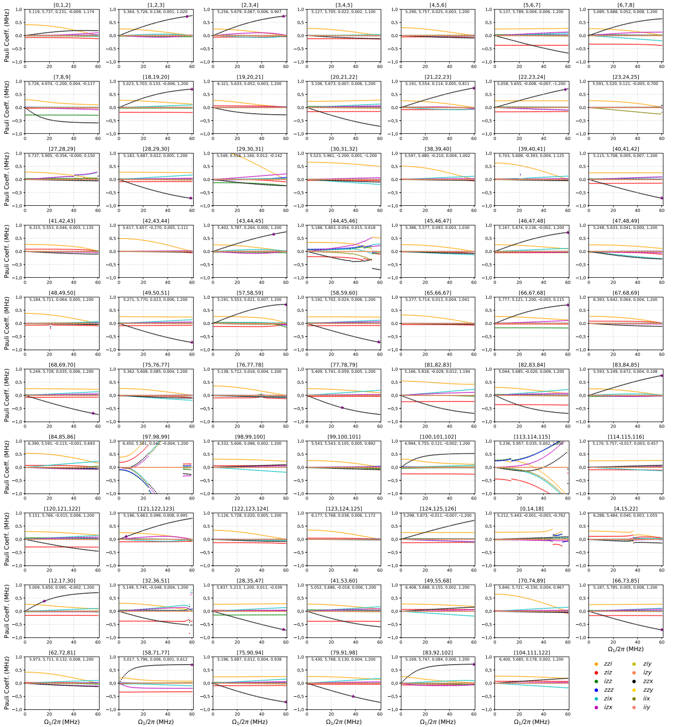
FIG. 8. Verification of Pauli coefficients for GHZ state generation using optimized parameters, with Q_1 and Q_3 serving as control qubits and Q_2 as the target qubit. The title of each panel indicates the labels of the evaluated qubits. The inset shows the optimized parameters in the form [\omega_{c12}, \omega_{c23}, A_1, A_2, A_3] , where A_j = \Omega_j / \Omega , and \Omega is the drive amplitude plotted along the x axis. In selected panels where GHZ state fidelity exceeding 90%, the star marks the drive amplitude at which the GHZ state reaches its maximum fidelity.
