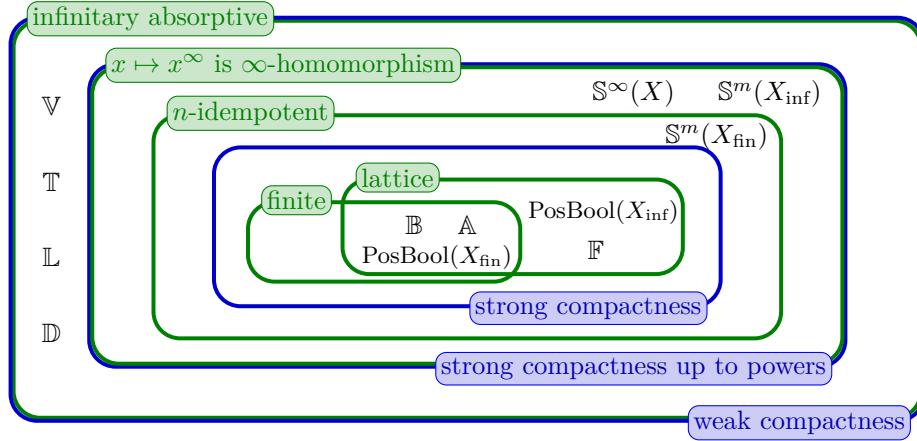
■ Figure 2 Relationship between variants of compactness and algebraic properties of the underlying semiring. While X_{\text{fin}} is a finite set of variables and X_{\text{inf}} an infinite set, X is of arbitrary cardinality.
