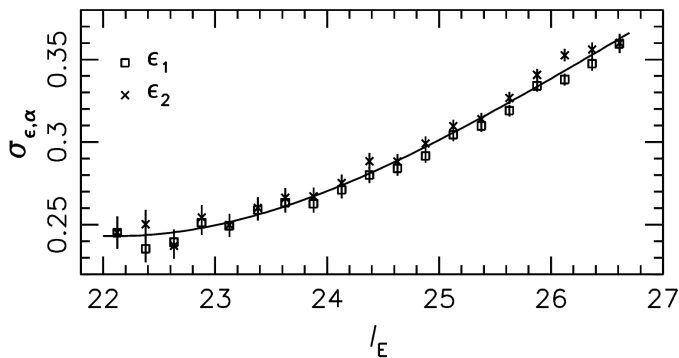
Fig. 9. Dispersion of the fully-corrected KSB+ ellipticity estimates as a function I_E , shown for both ellipticity components \epsilon_1 and \epsilon_2 . The smooth curve shows the best-fit third-order polynomial interpolation function, which is used for the computation of the empirical shape weight.
