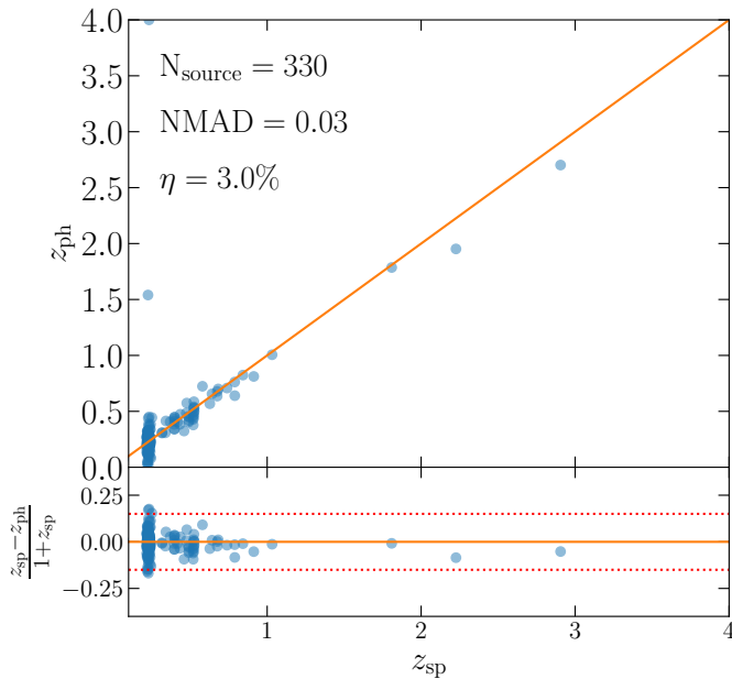
Fig. 3. Comparison of the best Phosphoros-derived photometric redshifts ( z_{\text{ph}} ) with spectroscopic redshifts ( z_{\text{sp}} ) for sources in the A2390 field. The top panel shows the direct comparison, while the bottom panel displays the redshift residuals defined as (z_{\text{sp}} - z_{\text{ph}})/(1 + z_{\text{sp}}) . The normalised median absolute deviation (NMAD) and outlier rate ( \eta ) are indicated. Dashed lines at \pm 0.15 show the residual threshold.
