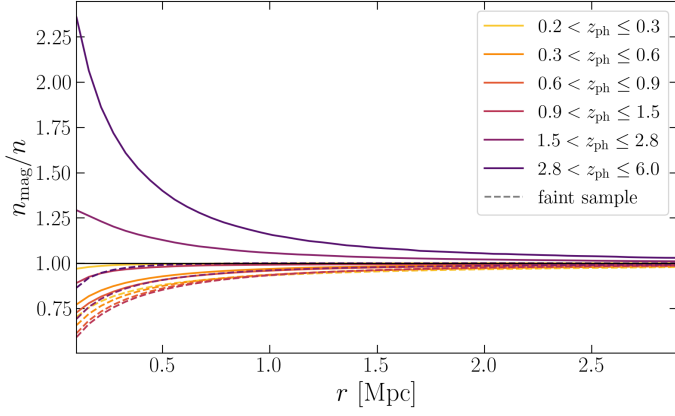
Fig. 14. Impact of magnification on source number densities for our setup and an M_{200c} = 1.5 \times 10^{15} M_{\odot} , c_{200c} = 4 NFW halo. The solid and dashed lines show the bright ( 22.0 < I_E < 24.5 ) and faint ( 24.5 < I_E < 26.5 ) samples, respectively.
