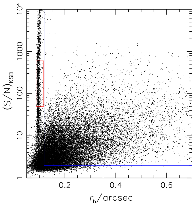
Fig. 7. Distribution of the KSB+ signal-to-noise ratio S/N_{\text{KSB}} versus half-light radius r_h for objects in the unfiltered KSB+ catalogue. The red box and blue lines indicate the pre-selection regions for the stars that are employed in the PSF modelling and for the galaxies, respectively. For clarity only a random subset of 20% of catalogue entries is displayed. Stars and noisy or poorly resolved galaxies are further removed from the shear catalogue via cuts in photometric redshift, magnitude, the SExtractor signal-to-noise ratio, and additional KSB+ selections (see H20).
