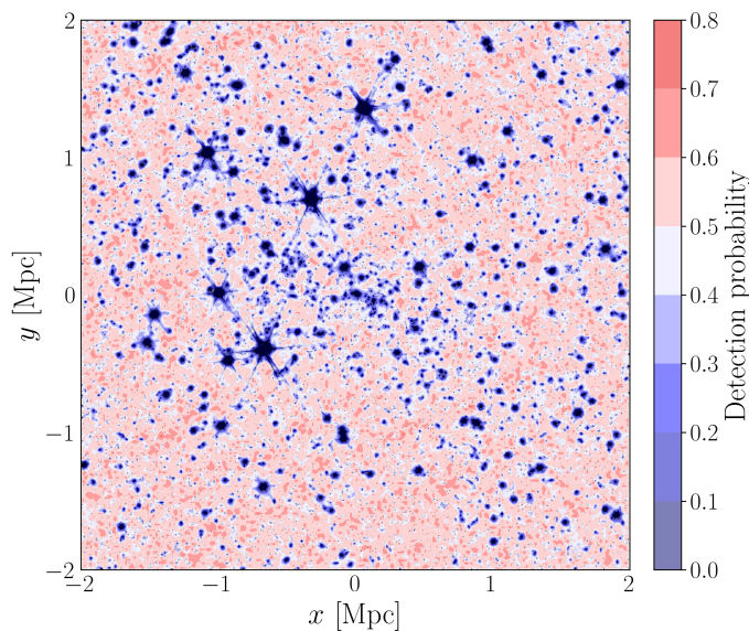
Fig. 12. Overlaid with the monochrome VIS image of Abell 2390, the colour coding shows the detection probability map of the whole injection input sample in the inner 4 \text{ Mpc} \times 4 \text{ Mpc} , with no selection in input magnitude, photo- z , or other quantities applied. The image injection pipeline captures cluster galaxies and foreground stars including their diffraction spikes.
