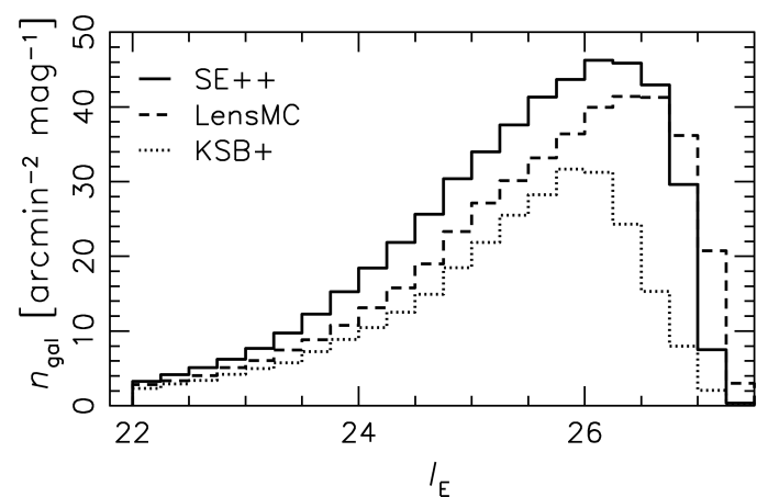
Fig. 6. Number density of objects in the LensMC (dashed), SE++ (solid), and KSB+ (dotted) weak lensing source catalogues, computed within the central 0:555 \times 0:555 of the VIS stack, after applying shear selection cuts and removal of objects in masked areas, but without applying photometric redshift selections.
