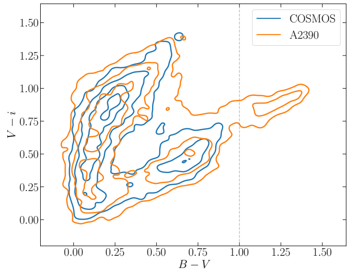
Fig. 4. Galaxy number density in the B - V , V - i colour-colour space for our A2390 catalogue and the COSMOS2020 catalogue with matched bands. Contours show the relative number density, with both blue and orange distributions sharing the same contour levels. The grey dashed line shows the selection cut.
