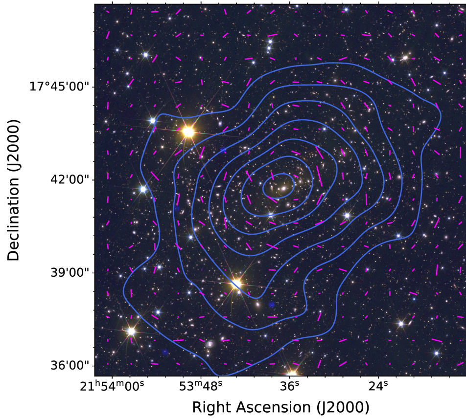
Fig. D.1. As Fig. 18, but employing the KSB+ shear catalogue.
