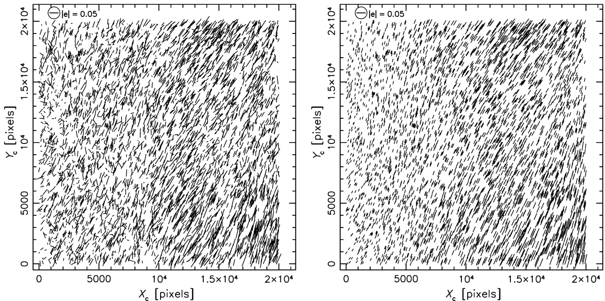
Fig. 8. Spatial variation of the PSF polarisation \epsilon_\alpha measured using a KSB+ Gaussian filter scale r_g = 0''.16 (left panel) and its 2D third-order spatially interpolated model (right panel). Here we consider the central 20000 \times 20000 pixels of this VIS stack (extending slightly beyond the primary WL region of interest, see Sect. 2.2), where the depicted coordinates (X_c, Y_c) relate to the pixel positions in the stack (X_s, Y_s) as (X_c, Y_c) = (X_s - 10799, Y_s - 10499) . The whisker in the top left indicates a reference polarisation with |e| = 0.05 .
