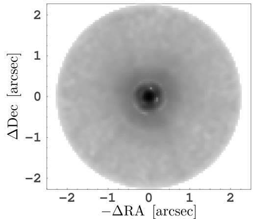
Fig. 2. VIS point-spread function recovered by PSFEx in the centre of the field of view. Pixel intensities are scaled on a logarithmic stretch. The image sampling is 0''.05 per pixel. The negative pixels close to the centre are artefacts caused by the oversampling, limited number of stars, and regularisation scheme applied by PSFEx (see Bertin 2011).
