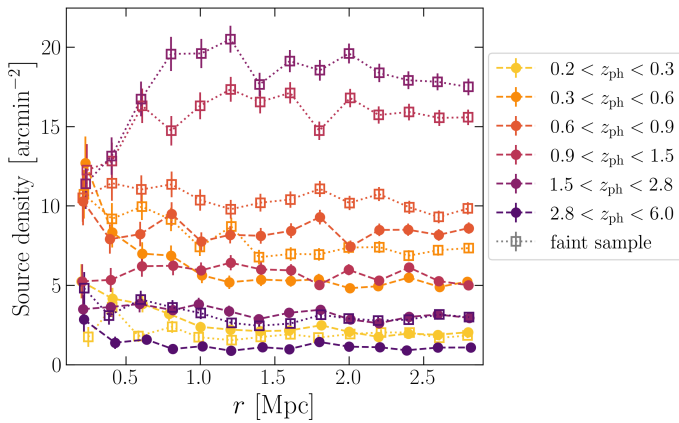
Fig. 11. Number density profiles of WL sources in bins of photo- z (colour-coded) and magnitude, where the solid and open symbols correspond to the bright and faint sample, respectively. Error-bars indicate Poisson uncertainties. In this figure, we account for masked areas, but not for obscuration.
