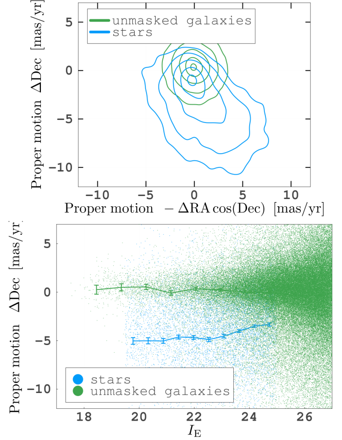
Fig. A.2. Top: Proper motion of stars (blue) and galaxies (green), showing clear evidence for more spread and shifted motion of the former population. Bottom: Proper motions of stars (blue) and galaxies (green) along the Declination direction as a function of I_E magnitude, illustrative of a stable systematic trend with magnitude, and thus indicative of mild cross contamination.
