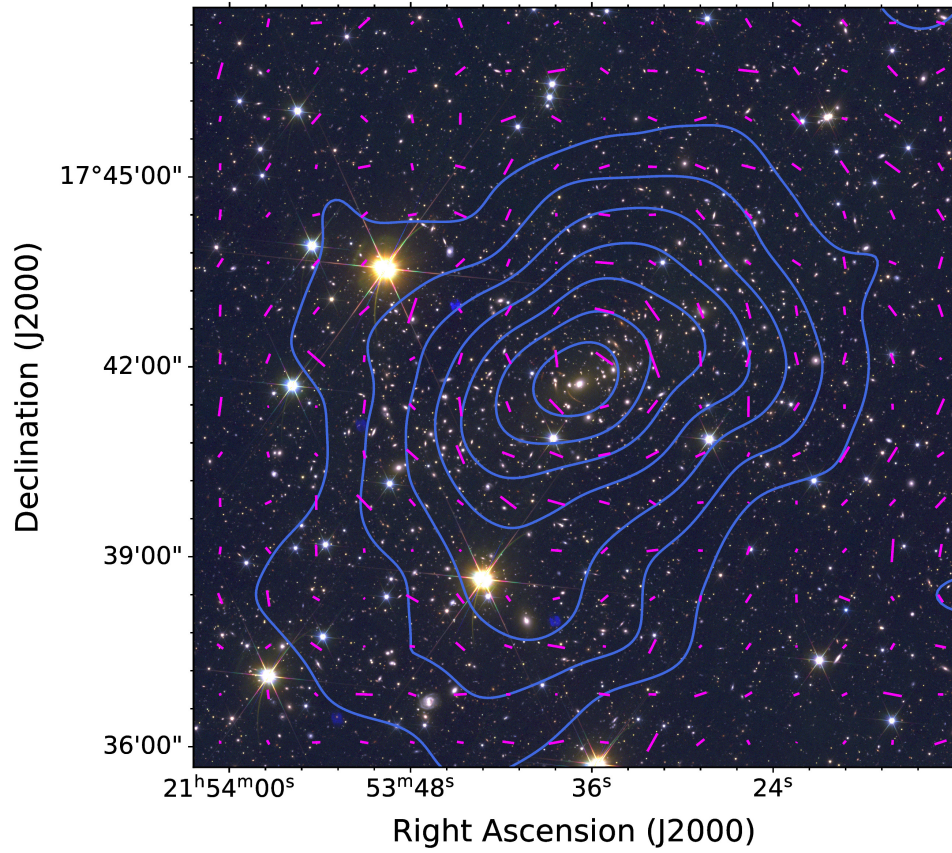
Fig. D.2. As Fig. D.1, but employing the SE++ shear catalogue.
