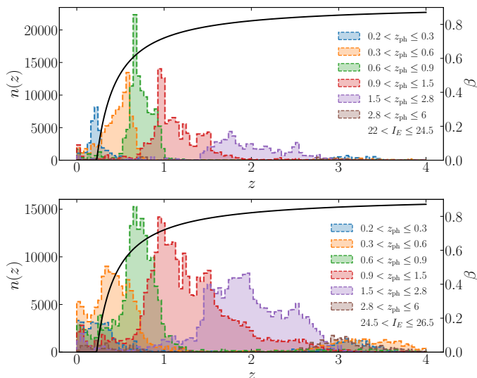
Fig. 5. Redshift distributions for each of our redshift and magnitude bins using the SE++ shear weights. The upper panel shows the distributions for the magnitude range 22 < I_E < 24.5 , and the lower panel for the range 24.5 < I_E < 26.5 . The black curve shows the geometric lensing efficiency \beta(z) , with the corresponding axis plotted on the right.
