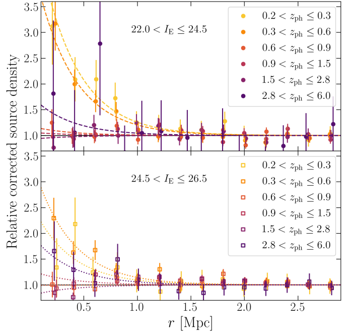
Fig. 15. Source number density profiles after correction for the impact of source obscuration and magnification, scaled to the corresponding mean value of the three outermost annuli. The increase over the baseline is a direct measure of the boost factor that we need to apply to compensate for cluster member contamination. We show an exponential model fit as dashed ( 22.0 < I_E < 24.5 ) and dotted ( 24.5 < I_E < 26.5 ) curves.
