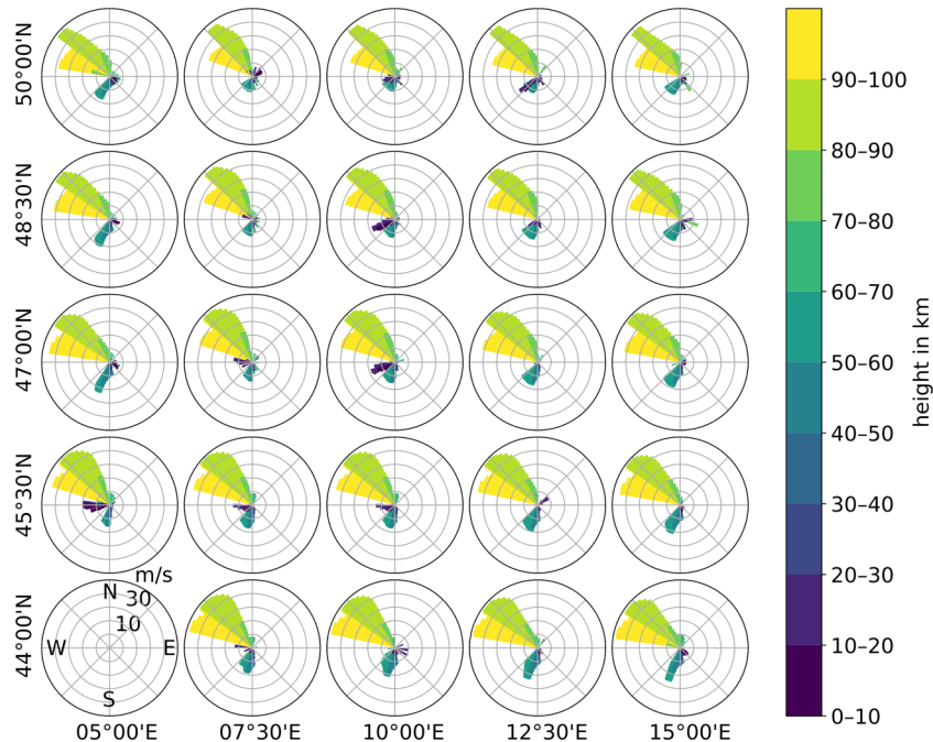
Figure 4. Grid of polar plots with 1.5° distance in N–S direction and 2.5° distance in W–E directions displaying wind direction, speed and height (colour). The direction of the colour-coded bins corresponds to the wind direction. The length of the bars denotes wind speed, ranging from 0 to 50 \text{m s}^{-1} (one circle corresponds to a 10 \text{m s}^{-1} increment). Each position of a polar plot within this grid corresponds to the location of its respective 1-D atmospheric model, which was employed to calculate these wind directions and speeds. Data is provided by the NCPAG2S-Client (NCPAG2S-CLC: Hetzer, C.H., 2024).
